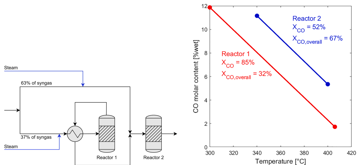
Fig. 7. DRI-EAF + SEWGS plant. Schematic of the split configuration adopted in the WGS section (left). Performance in terms of CO conversion of the WGS reactors (right).
