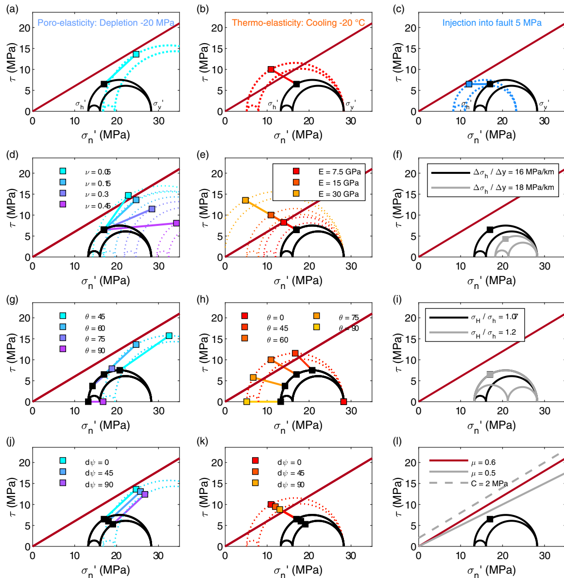
Fig. 9. Comparison of poro-elastic and thermo-elastic stress changes and sensitivity to various geomechanical parameters, for simplified lateral extensive reservoir geometry. Input values: normal faulting regime, depth: 2500 m, vertical stress gradient: 22 MPa/km, minimum horizontal stress gradient \Delta\sigma_h/\Delta y : 16 MPa/km, pore pressure gradient: 10.7 MPa/km, horizontal stress ratio \sigma_H/\sigma_h : 1.07, Young's modulus E : 15 GPa, Poisson's ratio \nu : 0.15, fault dip \theta : 70 degrees fault strike w.r.t. \sigma_H \phi : 0, friction coefficient \mu : 0.6, and cohesion C = 0 MPa. Poro-elastic stress changes are computed for a -20 MPa pressure drop with pressures within the fault following those of the reservoir, thermo-elastic stress changes for -20 degrees temperature decrease (cf. Soltanzadeh & Hawkes, 2009). a) poro-elastic stress change b) thermo-elastic stress change, c) direct pressure increase in the fault, with initial stress state in black and final stress state depicted by the dotted line. Black marker: initial fault stress, colored line: stress path, colored marker: final fault stress. Sensitivities of poro-elastic stress changes are shown for d) Poisson ratio, g) dip, and j) strike, and sensitivities of thermo-elastic stress are shown for e) Young's modulus, h) dip, and k) strike. Furthermore effect of horizontal stress gradient (f), horizontal stress ratio (i) and effect of fault friction and cohesion (l) on initial stress are shown.
