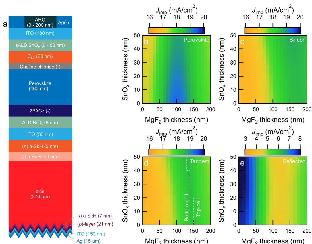
Figure 3. Optical simulations of perovskite/SiHJ tandem devices. (a) Schematic sketch of the perovskite/SiHJ solar cell used for simulations. (b–e) Implied photocurrent density in (b) perovskite top-cell, (c) silicon bottom-cell, (d) tandem cell, and (e) implied reflected photocurrent density. The dashed line in (d) distinguishes between configurations that are limited either by the bottom-cell or by the top-cell.
