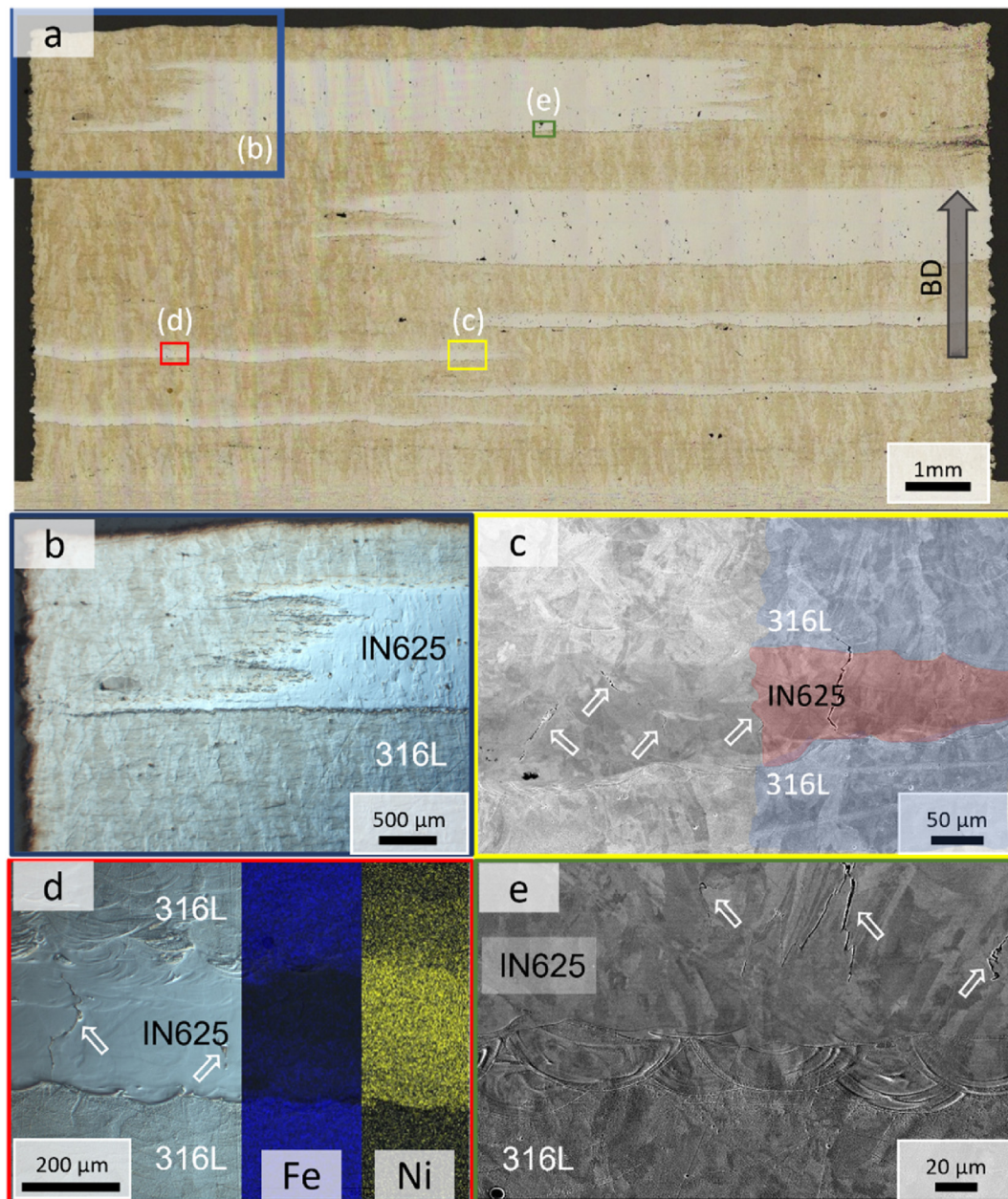
Fig. 3 – Cross-sectional micrographs, recorded using confocal laser scanning microscopy (a,b,d) and SEM (c,e) indicate the presence of micro-cracks in IN625 regions of the multi-metal sample. Each magnified area from (b) to (d) is highlighted in colour in (a). IN625 regions appear brighter in the overview (a) and the build direction (BD) is indicated by an arrow. An additional chemical analysis by EDS (d) revealed a morphological sharp interface whenever IN625 was applied on S316L but a blurred interface when S316L was applied onto IN625. Perpendicular to the BD, an intermixing at the interface of ~1 mm in width could be determined (b). Bundles of grains with a preferred orientation that correlates with the BD could be determined in the SEM images (c) and (e).
