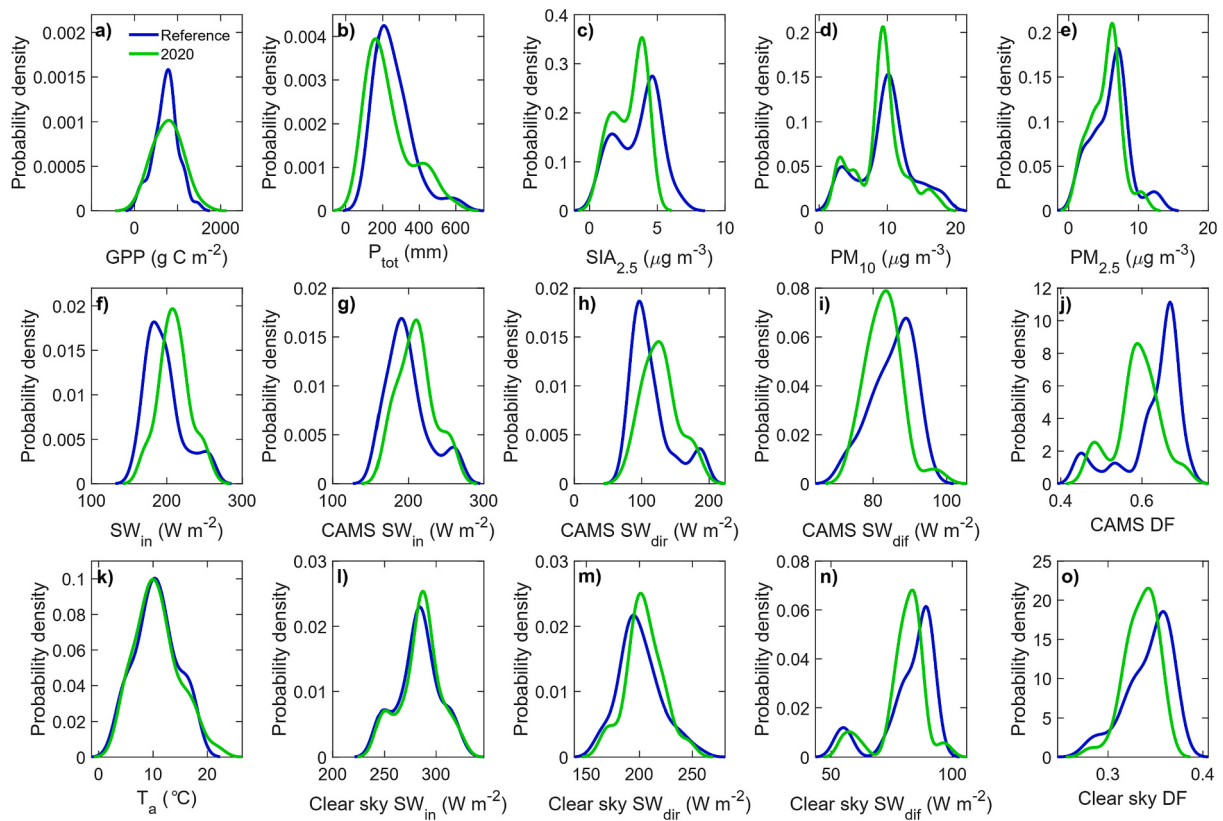
Fig. 3. Comparison of reference (blue line) and 2020 spring (green line) probability density distribution across 44 sites in Europe for (a) GPP (gross primary production), (b) P_{\text{tot}} (precipitation), (c) \text{SIA}_{2.5} (secondary inorganic aerosol smaller than 2.5 \mu\text{m} ), (d) \text{PM}_{10} (particulate matter smaller than 10 \mu\text{m} ), (e) \text{PM}_{2.5} (particulate matter smaller than 2.5 \mu\text{m} ), (f) \text{SW}_{\text{in}} (incoming shortwave radiation, measured on-site), (g) \text{SW}_{\text{in}} from the Copernicus Atmosphere Monitoring Service (CAMS), (h) CAMS \text{SW}_{\text{dir}} (direct radiation), (i) CAMS \text{SW}_{\text{dif}} (diffuse radiation), (j) CAMS DF (diffuse fraction), (k) T_a (air temperature), (l) clear sky \text{SW}_{\text{in}} , (m) clear sky \text{SW}_{\text{dir}} , (n) clear sky \text{SW}_{\text{dif}} and (o) clear sky DF.
