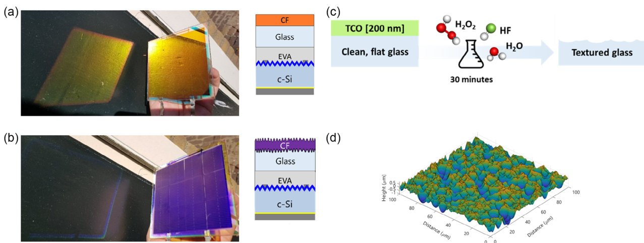
Figure 4. Two different colored mini-PV modules (10 × 10 cm) based on aluminum–back surface field (Al–BSF) laser-cut solar cells. a) An orange CF deposited at the top of flat glass ( p = 10 , \text{SiO}_2 = 90 nm, \text{SiN}_x = 100 nm), which produces significant glare. b) The glare is completely reduced by deposition of the CF on a randomly textured glass ( p = 10 , \text{SiO}_2 = 68 nm, \text{SiN}_x = 164 nm). More information about these results can be found in the work of S. Villa. [15] c) Wet–chemical etching procedure of glass mediated by transparent conductive oxide. [44] d) Atomic force microscope image of a typical etched glass used for improving color stability (statistical data of the randomly textured surface can be found in the work by Loeff [33] ).
