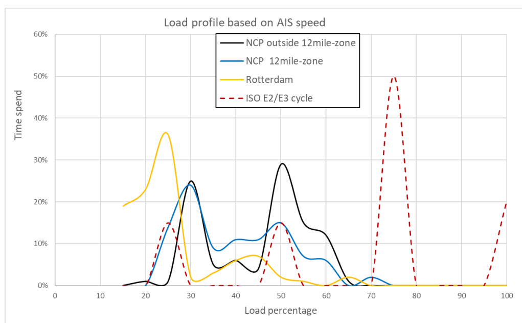
Figure 2-2. Projected average load profile on the North Sea, Netherlands Continental Plat. Source TNO, 2019.
