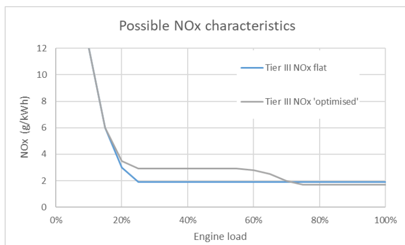
Figure 2-1. Possible NO x characteristic, both with E2/E3 cycle average of 1.9 g/kWh. Lowering NO x to 1.7 g/kWh for high load points, makes it possible to increase NO x to almost 3 g/kWh up to 70% load.
