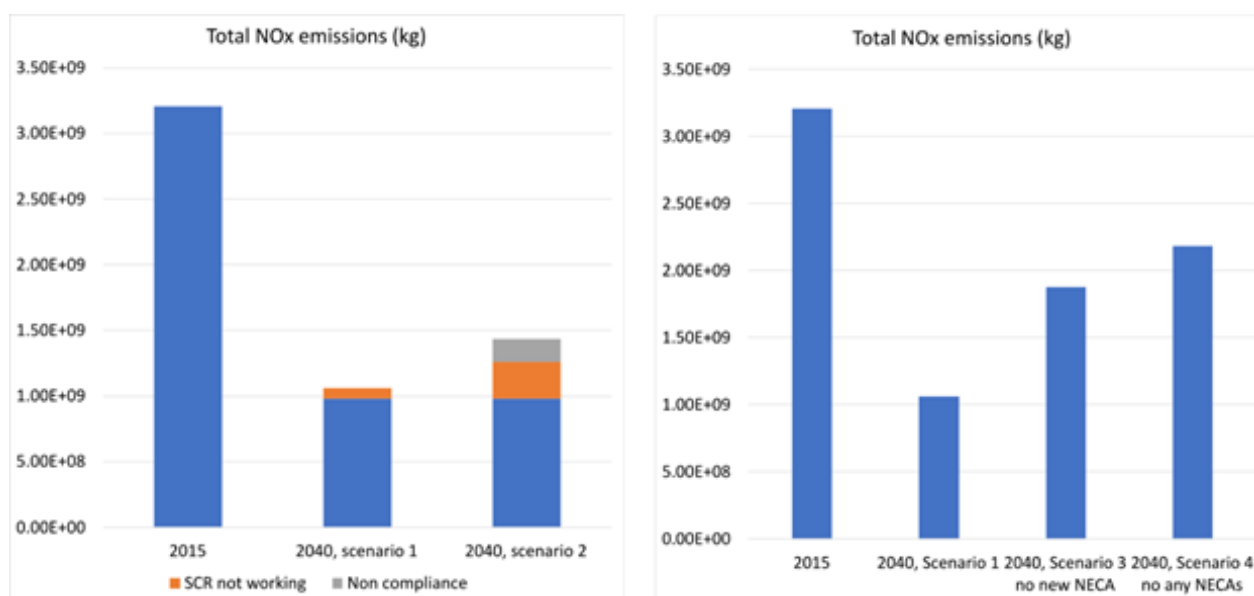
Figure 4-I Total emissions of nitrogen oxides (NO x ) from shipping in Europe in 2015 and 2040 under different regulatory scenarios simulated using the STEAM model (from SCIPPER D5.4).
