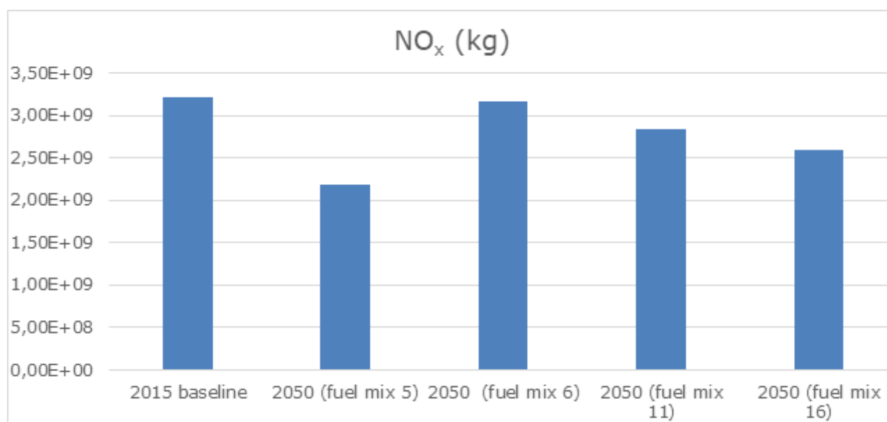
Figure 4-2 Total shipping emissions in 2050 compared to 2015 for CO 2 (top) and NO x (bottom) for the DNV fuel mix scenarios 5, 6, 11, and 16 (from SCIPPER D4.3).
