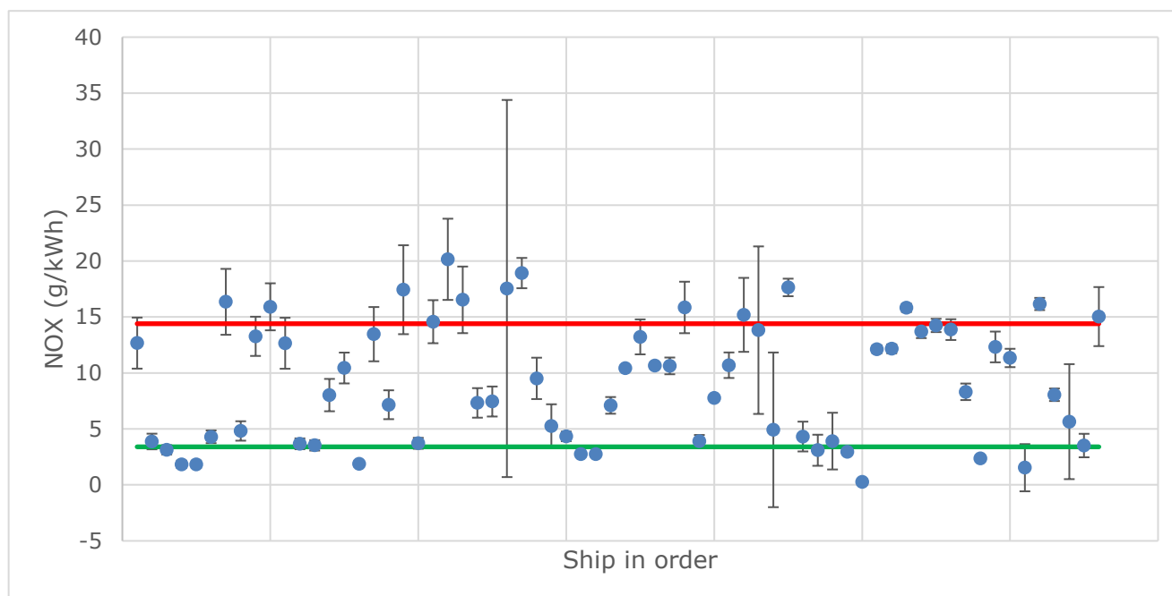
Figure 5-1. Remote sensing observations of Tier III ships keel laid from 2021 within the North European NECA. The measurements were carried out in different projects by fixed remote measurements at Great Belt bridge (13 ships, Chalmers, SHIPTRASE), and Wedel (1 ship, BSH, SCIPPER) and by airborne measurements in Danish and French waters (10 ships, Explicit, French Maritime Authority) and in Rotterdam (73 ships, TNO). The green line shows the Tier III limit value (all ships have slow speed engines); the red line shows the Tier II limit value.
