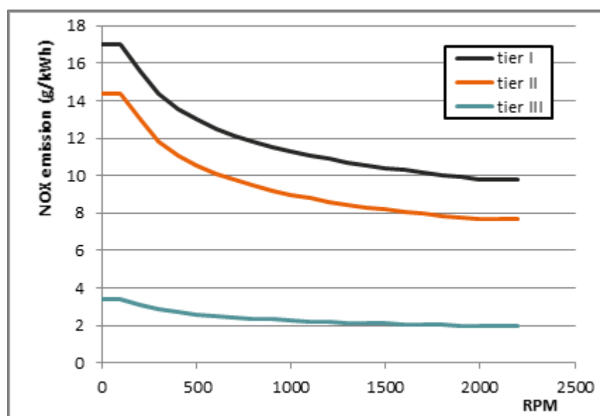
Figure 2-2. IMO regulations in emissions of NO x from marine engines.
