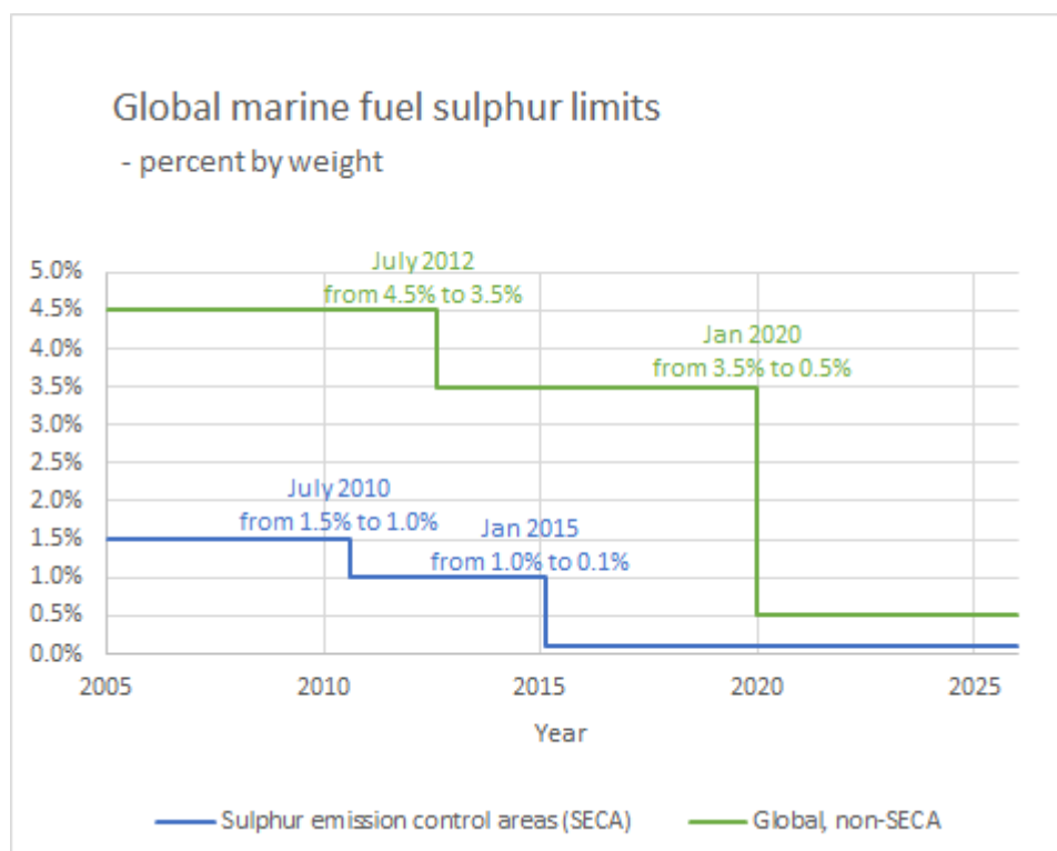
Figure 2-1. Global marine fuel sulphur regulations
