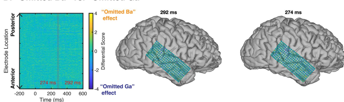
Fig. 5. Comparison of the experimental conditions using generalized linear model (GLM) analysis. First, GLM analysis was applied to investigate the effect (beta coefficients) of the experimental conditions (“Ba,” “Ga,” “Omitted Ba” and “Omitted Ga”) to HFA responses. Next, the difference between two effects of different condition was calculated as “Ba” vs. “Ga” (A), “Ba” vs. “Omitted Ba” (B), “Ga” vs. “Omitted Ga” (C), and “Omitted Ba” vs. “Omitted Ga” (D). (A) Topographies are from the specific time points in the channel by time map of differential effects between two conditions. A positive value (yellow color) means that the “Ba” effect was bigger than “Ga” and a negative value (blue color) means that the “Ga” effect was bigger than “Ba” for each electrode. This GLM analysis yields “Ba” and “Ga” features that can be distinguished in a time domain (see the channel by the time map in A), whereas spoken and omitted sounds can be spatially distinguished (see topographies of A and B).
