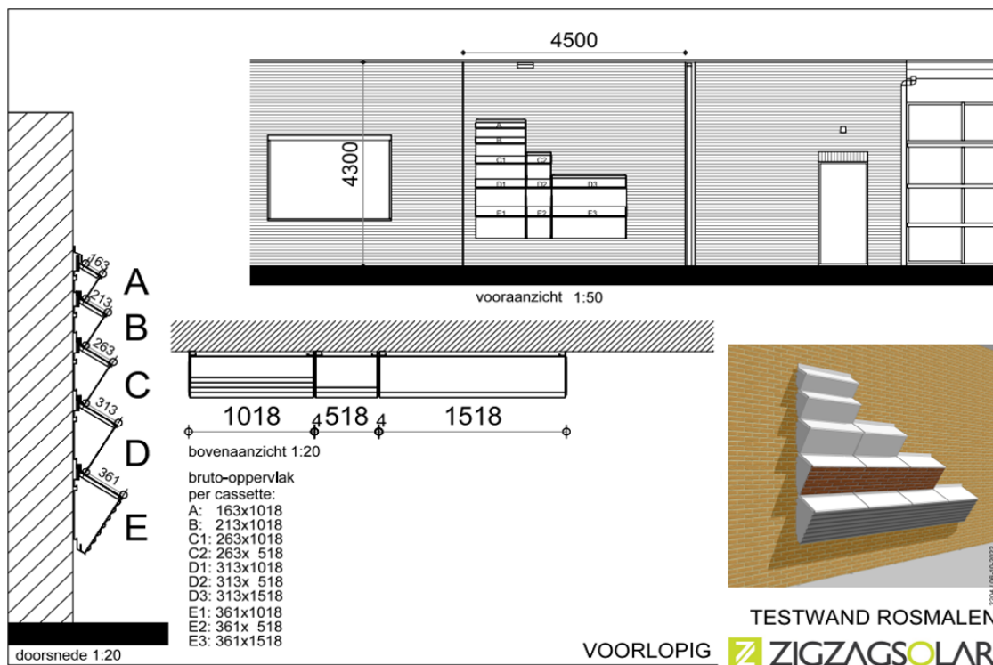
Figure 12: BIPV-demonstrator in SolarEMR-project shows freedom of shape for the ZigZag Solar façade: 10 different sizes (labeled A till E3) are requested from the integrator company (ZigZag Solar) and assembled by the supplier of the laminates (TNO).
