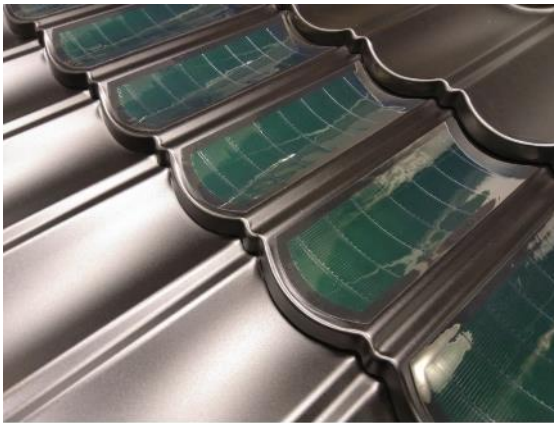
Figure 7: Curvature in the laminates is needed when the application with curved roof tiles is desired.
