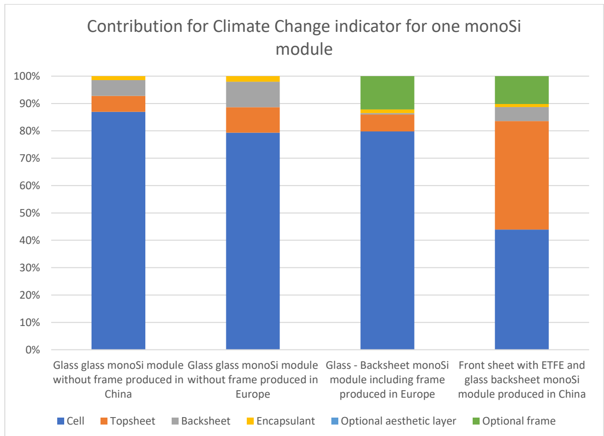
Figure 23: Comparison between several scenarios of modules with different composition and location of production. Aesthetic layers are not shown yet because of the lack of information regarding its composition. Backsheet of third scenario is composed of PVF,PET and LLDPE (surrogates of real elements composing the backsheet).
