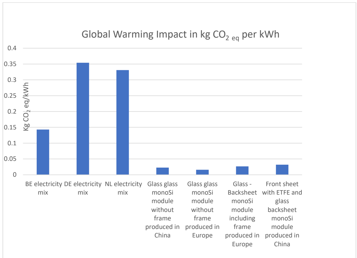
Figure 26: Comparison with national electricity mixes and electricity generated by solar modules. Higher scores are expected for modules when adding share of infrastructure and balance of system. National electricity mix data from https://ourworldindata.org/grapher/carbon-intensity-electricity?tab=table (data of 2021).
