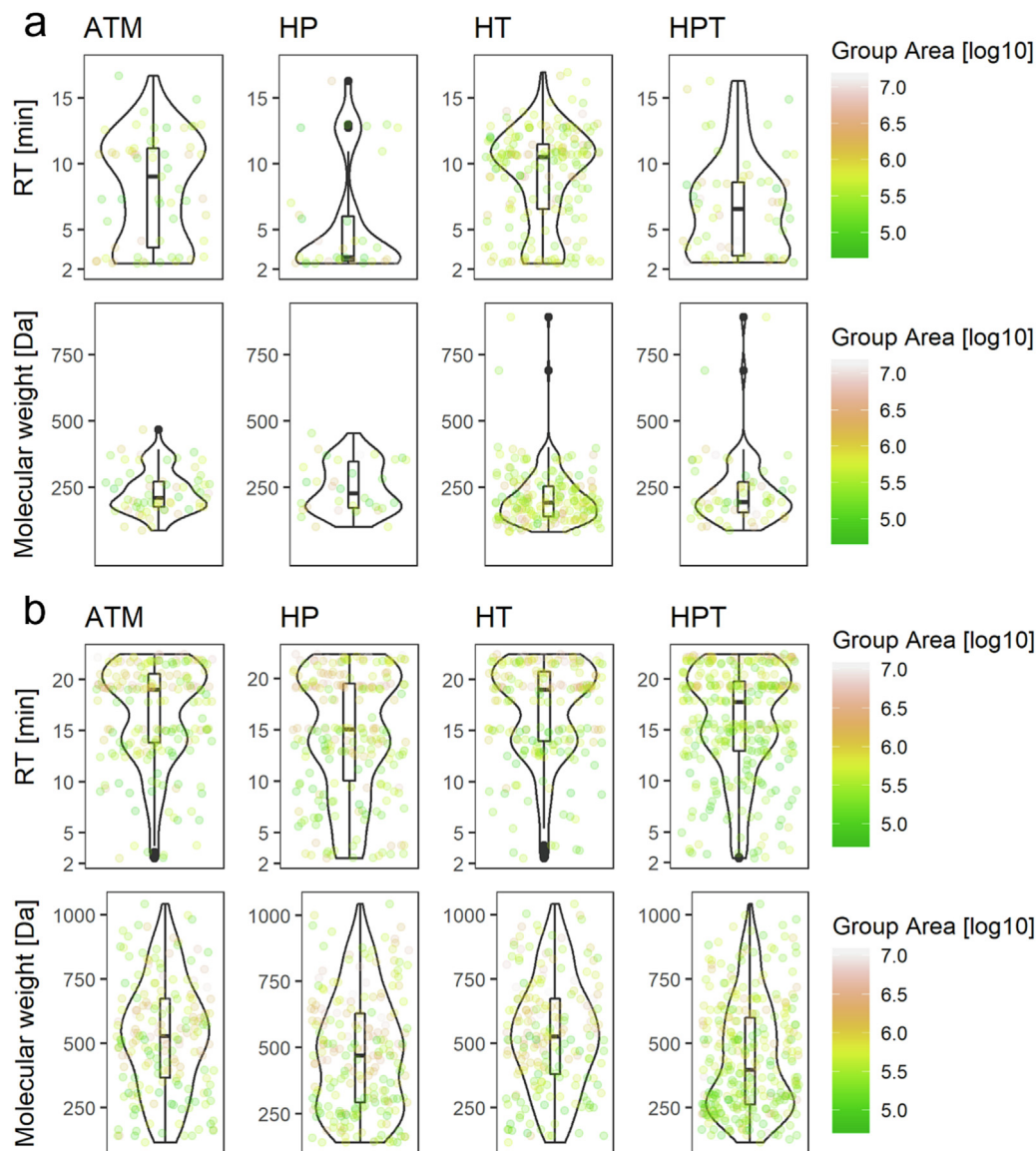
Fig. 2. Retention time and molecular weight distributions of features in positive ionisation mode for (a) the liquid phase (features with \log_2\text{FC} > 5 between FBW + S samples and FBW samples were considered) and (b) the solid phase (features with \log_2\text{FC} > 5 between FBW + S samples and UPW + S samples were considered) for the four conditions.
