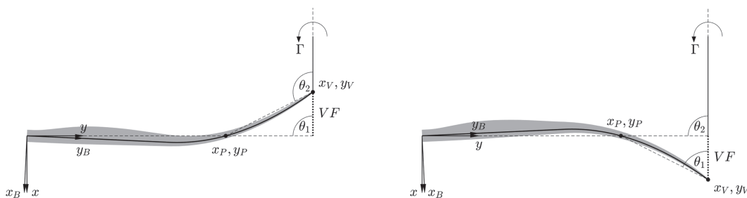
FIGURE 4 Schematic of the additional/missing vortex filament (dotted line) for an aft swept blade (left) and forward swept blade (right)
