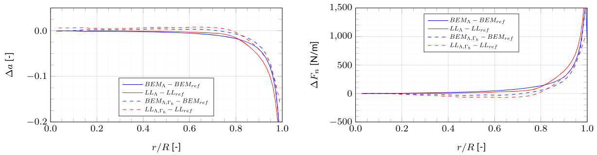
FIGURE 11 Spanwise distribution of sweep induced changes to the axial induction factor (left) and normal force (right), case: U = 10 \text{ m/s} , \lambda = 9 , \beta_{pitch} = 0^\circ , y_{start} = 0.5R , x_{tip} = -0.2R , \gamma = 2
