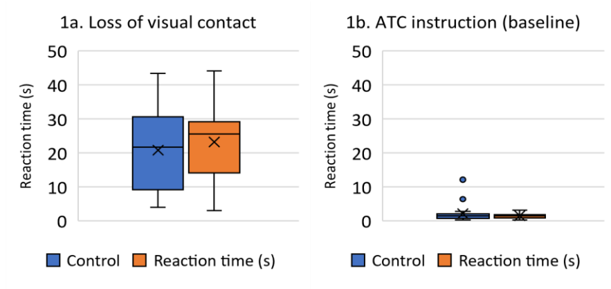
Figure 4. Tukey boxplots of time to first response in go-around test scenarios 1a and 1b
