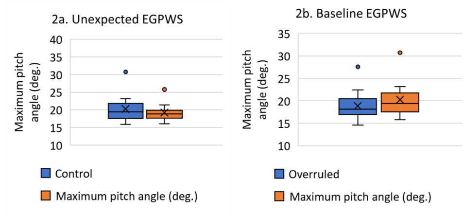
Figure 17. Tukey boxplots of maximum pitch angle in test scenarios 2a and 2b
