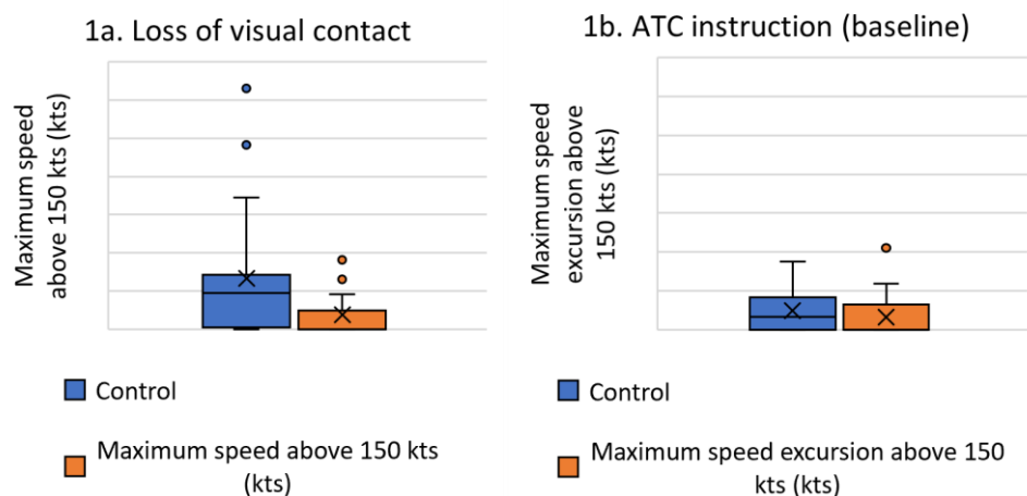
Figure 8. Maximum speed excursion above upper bound of 150 kts
