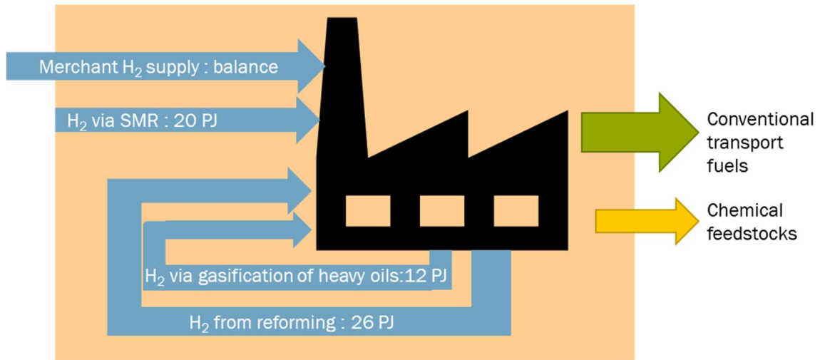
Figure 3.1 Schematic presentation of hydrogen flows to the fossil refineries (captive values are derived from MIDDEN report (PBL & TNO, 2020a))
