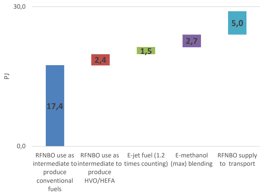
Figure 4.2 Illustration of case 2
