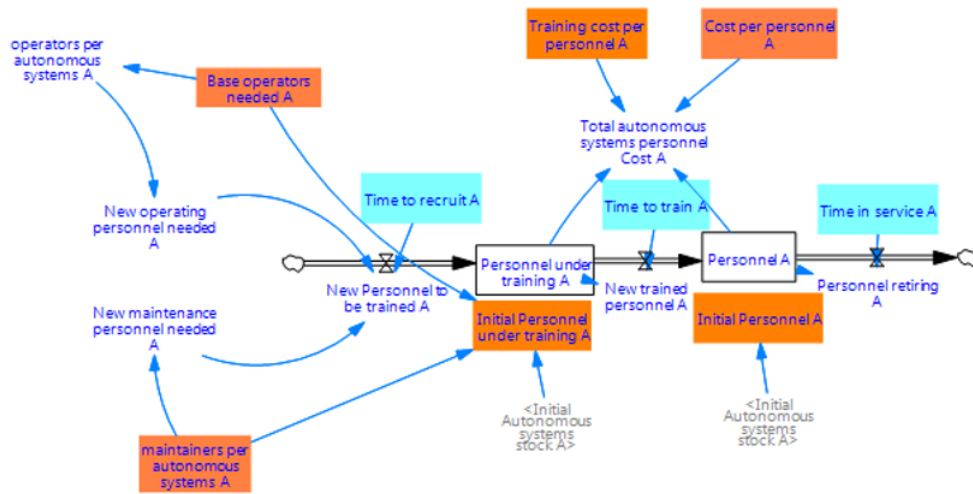
Figure 6: Personnel for operating and maintaining the autonomous capabilities of Nation A.
