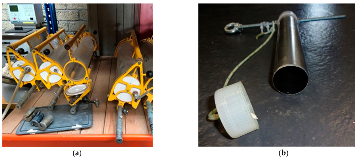
Figure 3. Tools for water and sediment sample collection: (a) water sample collection bottles with a volume of 3 L, and (b) tubes for sediment sample collection with a diameter of 40 mm. Samples for metal analysis were collected using polypropylene tubes.
