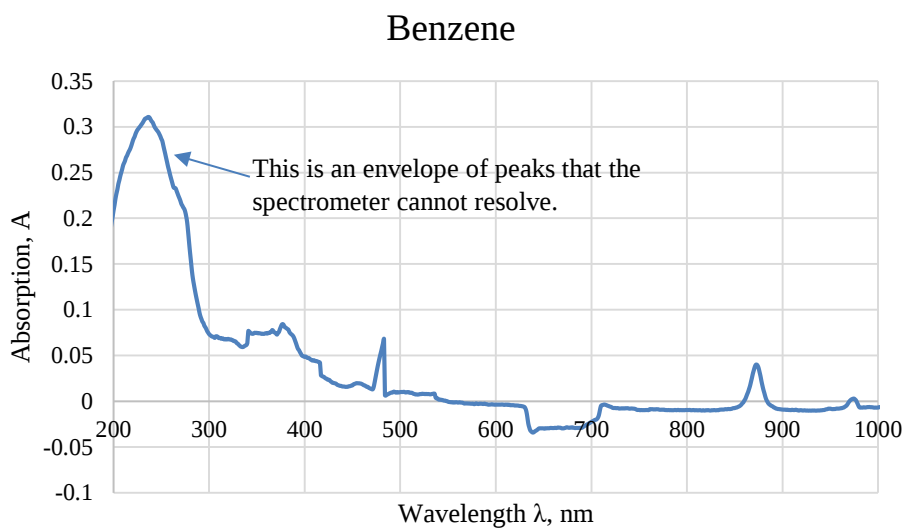
Figure 15. UV-VIS spectrum of benzene.
