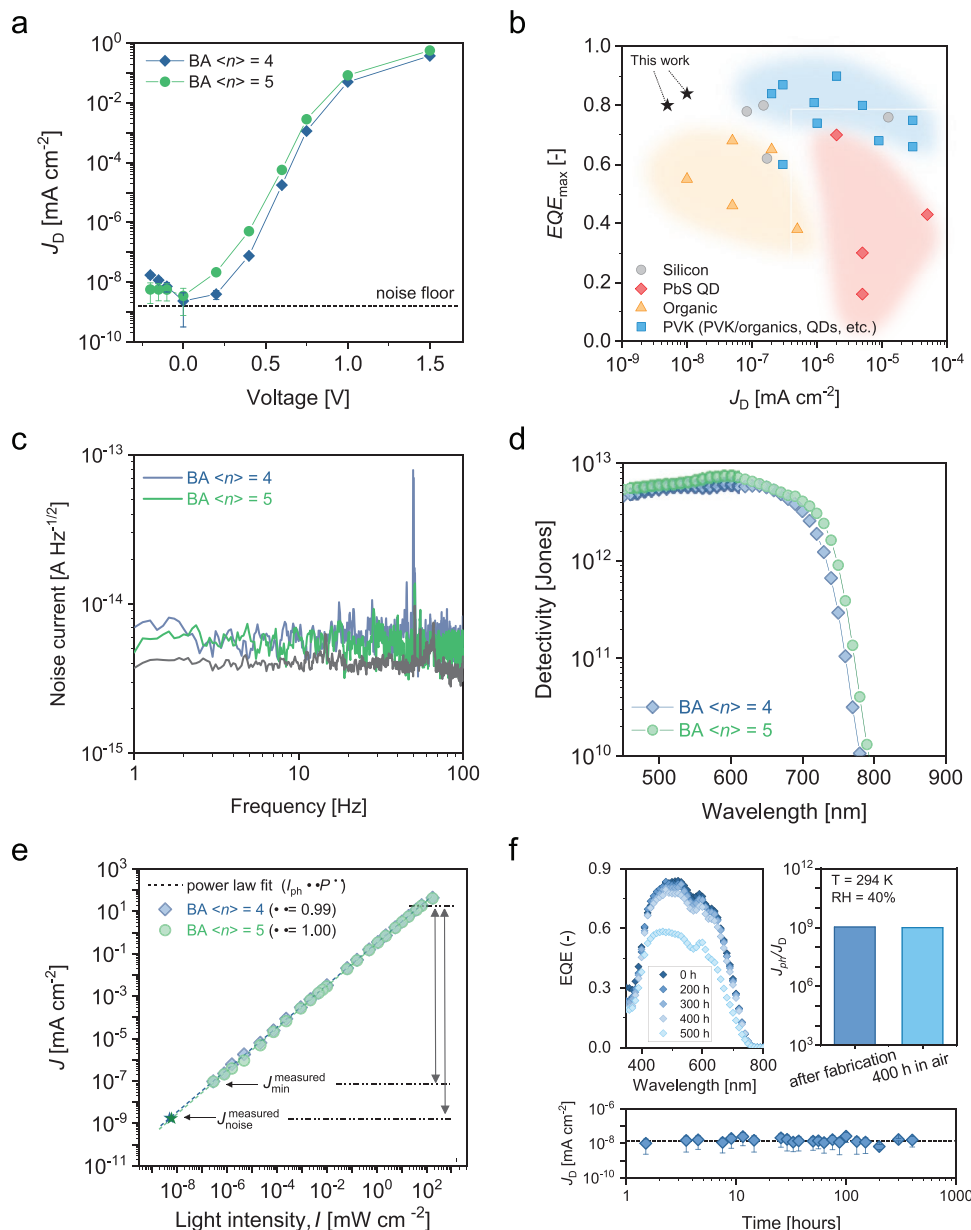
Figure 5. a) J – V characteristics in dark; from -0.2 to +0.6 \text{ V} , J – V have been reconstructed from constant voltage measurements over time at discrete biases. Whiskers represent standard deviation. b) Plot of maximum EQE versus minimum J_D comparing our PPDs with state-of-art solution-processed photodiodes and commercial silicon. For each device, J_D at V = -0.2 \text{ V} is reported. Further details are in the Supporting Information. c) Noise current spectral density as a function of frequency measured at -0.2 \text{ V} for the best devices. Each spectrum is obtained with an average of 15 measurements. Harmonics with large amplitude in the spectrum are due to powerline interference. Black line represents the noise floor of the setup ( \approx 4 \times 10^{-15} \text{ A Hz}^{-1/2} ). d) Specific detectivity of the photodiodes versus wavelength under reverse bias ( -0.2 \text{ V} ). e) Photocurrent, J_{ph} , measured at -0.2 \text{ V} for a broad range of light intensities (540 nm). Lines denote a linear fit, with \alpha the power law exponent equal to unity. f) Stability in air (RH 40%) of BA \langle n \rangle = 4 PPD after >400 \text{ h} , expressed in terms of EQE (top left), J_{ph}/J_D ratio (top right), and J_D over time (bottom). J_{ph} is integrated from the EQE spectrum at V = 0 \text{ V} , J_D is measured at constant voltage measurements over time at discrete biases (symbols and whiskers represent mean values and standard deviation).
