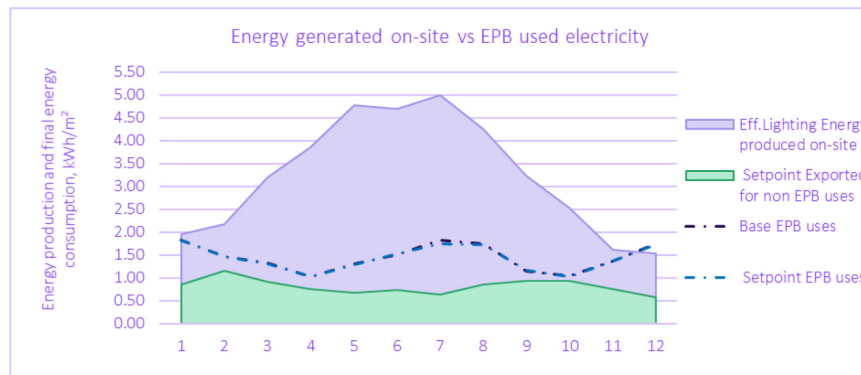
Fig. B.2.5. Annual energy performance for energy flexibility scenario Epc21 considers the tighter setpoints for heating and cooling for the Austrian demo.
