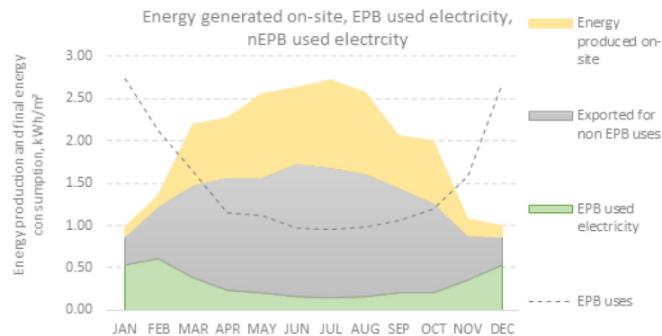
Fig. B.1. Energy generation on-site compared to EBP uses for the base case design of the Spanish demo.
