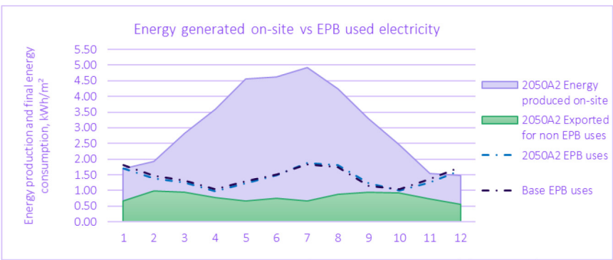
Fig. B.2.3. Energy generation on-site compared to EPB uses CL2 scenario of the Austrian demo.
