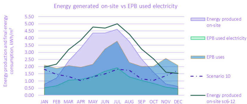
Fig. B.2.2. Energy generation on-site for final design compared to EPB uses for the base case design of the Austrian demo. Negative non-renewable primary energy consumption means that there is a surplus of renewable energy onsite compared to EPB uses.
