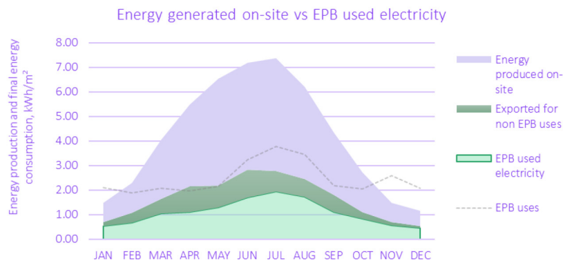
Fig. B.2.1. Energy generation on-site compared to EPB uses for the base case design of the Austrian demo.
