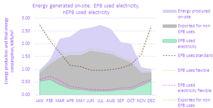
Fig. B.2. Spanish: Annual energy performance for energy flexibility scenario F11 (flexible).
