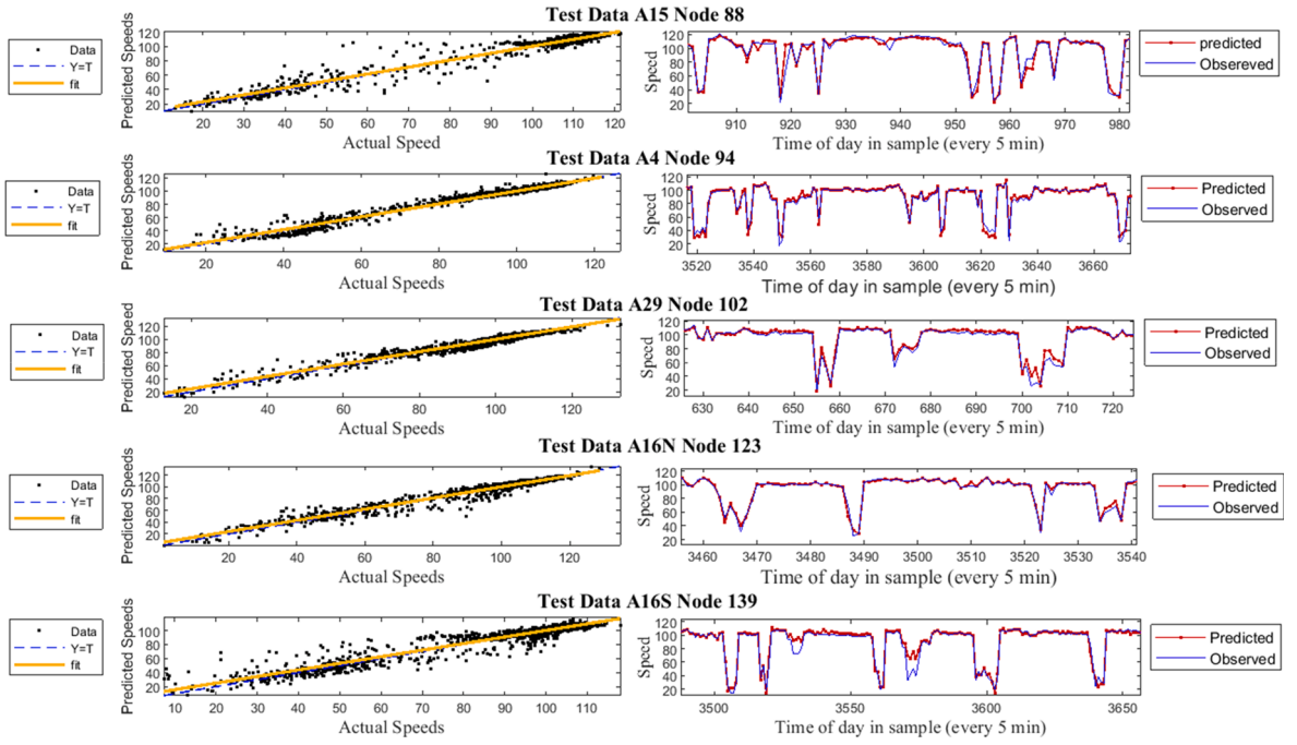
Fig. 8. Linear fit between observed and predicted speed.
