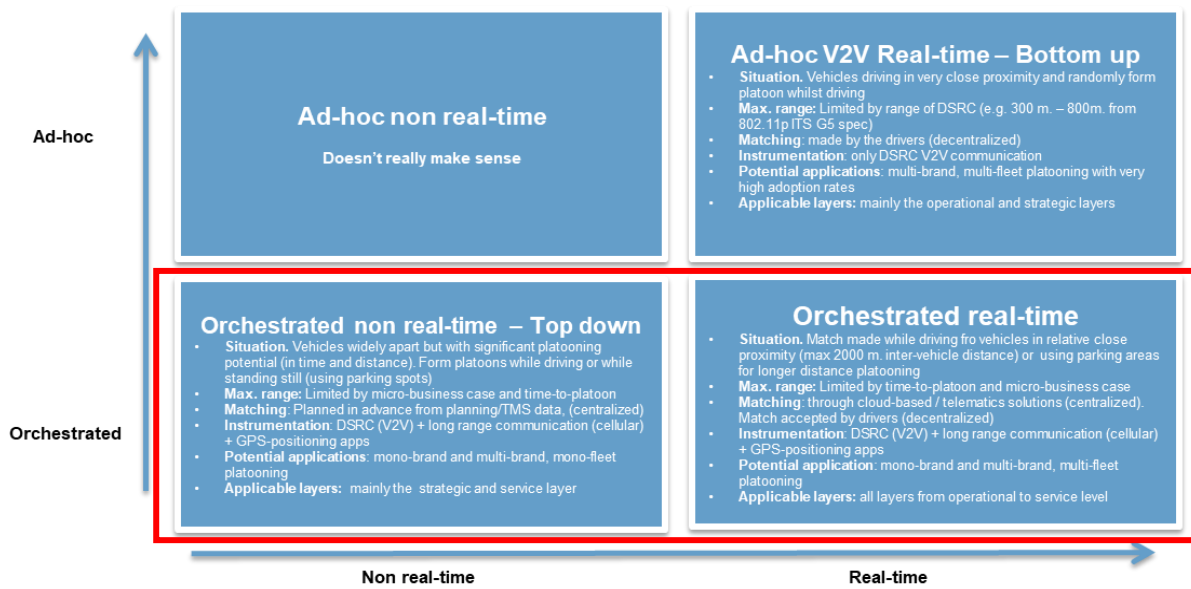
Figure 4-5: Platooning formation (red box) (Burgmeijer, 2017).
