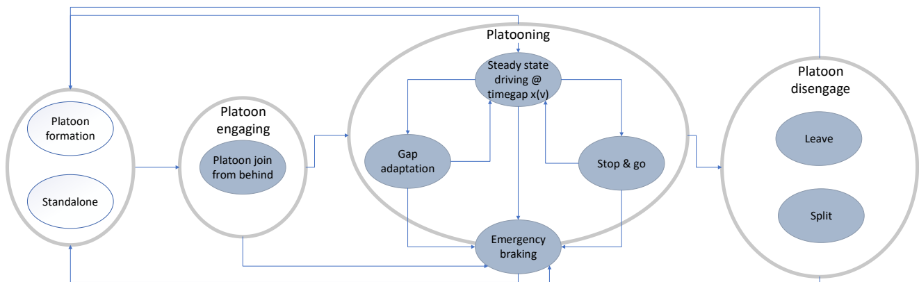
Figure 3-3: High level manoeuvres interaction.
