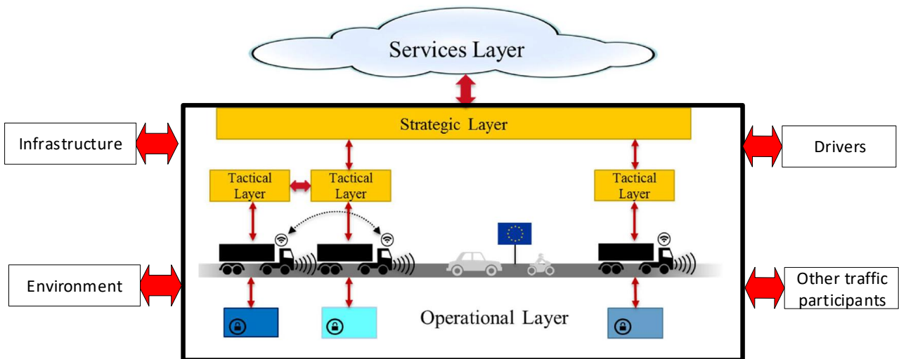
Figure 4-7: Main interfaces.
