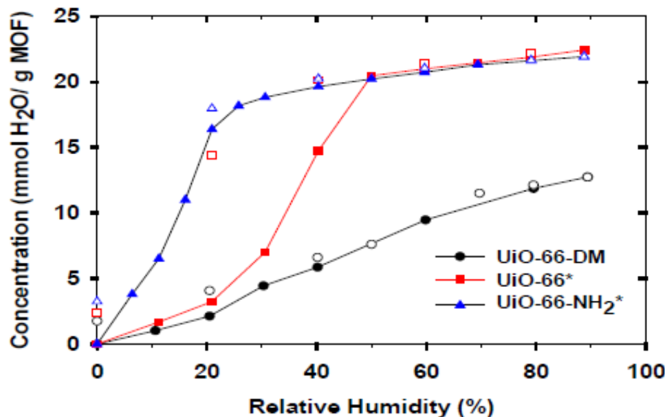
Figure 3-20: Water Vapor Sorption/Desorption Isotherm for Desolvated Compounds of UiO-66-DM, UiO-66, and UiO-66-NH 2 (Closed symbols – adsorption; Open symbols – desorption) [40].
