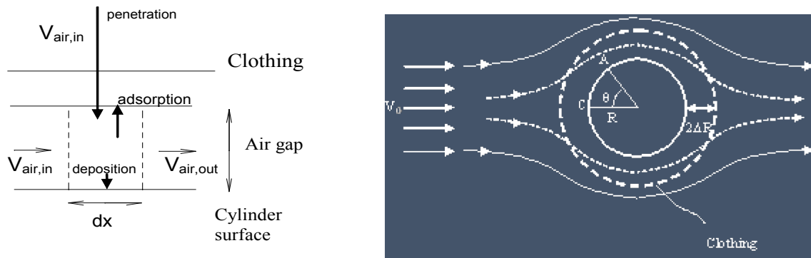
Figure 3-2: Schematic View of the Analytical Approach in Which Several Processes from the Full CFD Simulations Have Been Neglected or are Estimated. Results and picture from Brasser, TNO, Netherlands [4]-[5].
