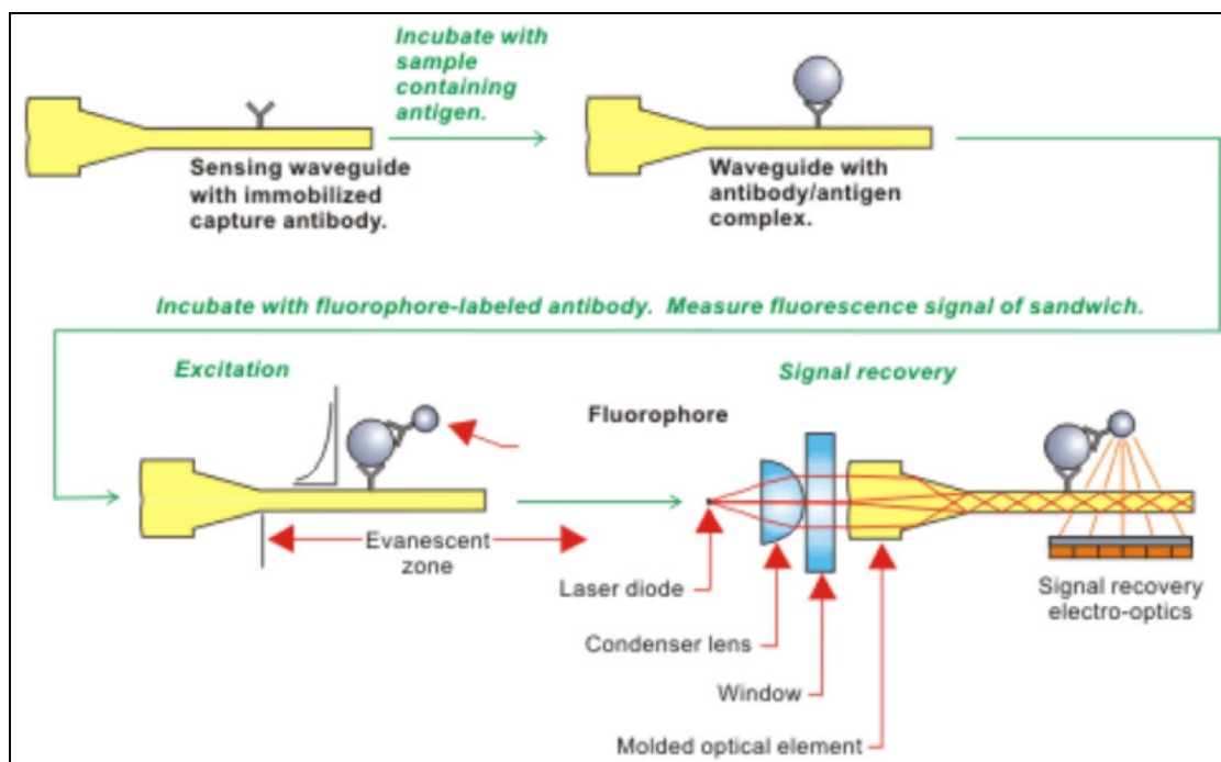
Figure 2-9: The Evanescent Wave Concept.
