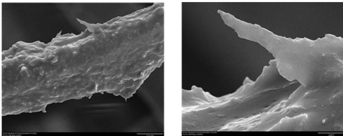
Figure 3-11: SEM Image of a Fluorinated Nylon Fiber with Newly Developed Coating Technology. The nylon surface has needle-shape multiscale protuberances that can provide reduced contact between a liquid and a solid as reported in FY 12.
