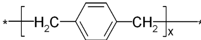
Figure 4-2: Parylene Polymer.
