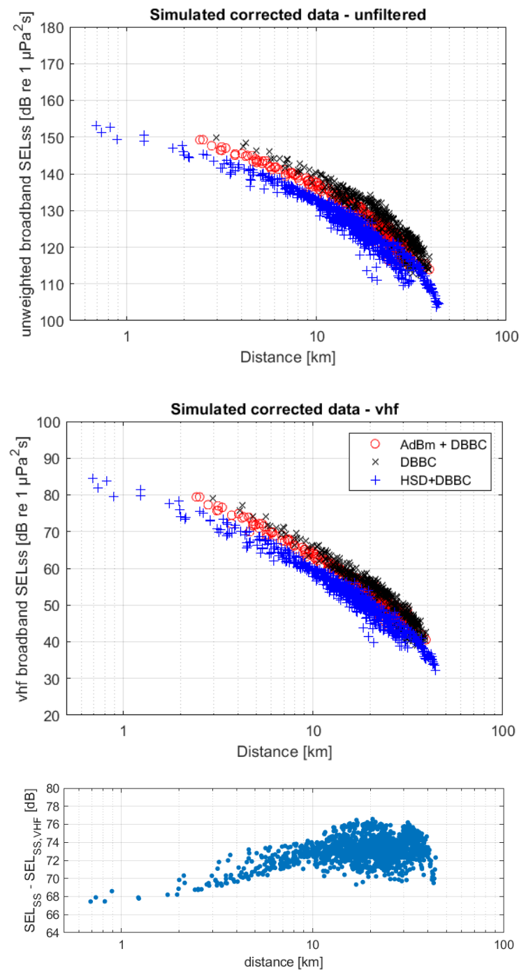
Figure 14 Modelled broadband (50 Hz – 500 Hz) SELss as a function of the pile-recorder distance (one marker for each pile recorder combination), using the model calibration. Upper: unweighted SELss; Middle: porpoise-weighted \text{SEL}_{\text{SS,VHF}} . The three mitigation configurations are indicated by three different markers and colours. The lower figure shows the difference between the unweighted and weighted SELss as a function of distance, illustrating that the weighted SELss drops faster with increasing distance.
