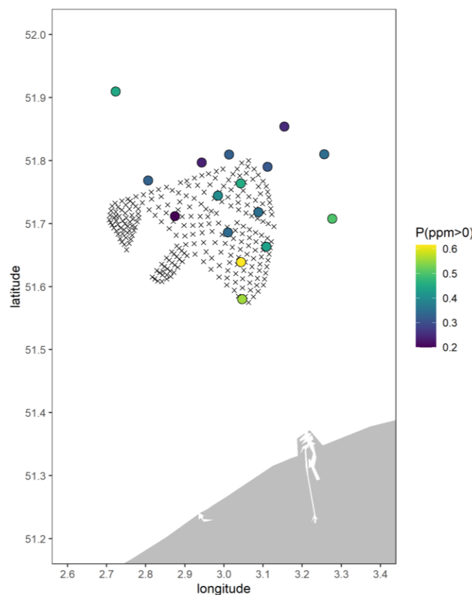
Figure D.12 Predictor effect plot of the random intercept for location for the unweighted SEL based Bernoulli model. The plots show the predicted probability of a porpoise positive minute (PPM), while setting mdtps to -1 (meaning no piling), and ignoring the other random effects/smoothers (which average out to 0).
