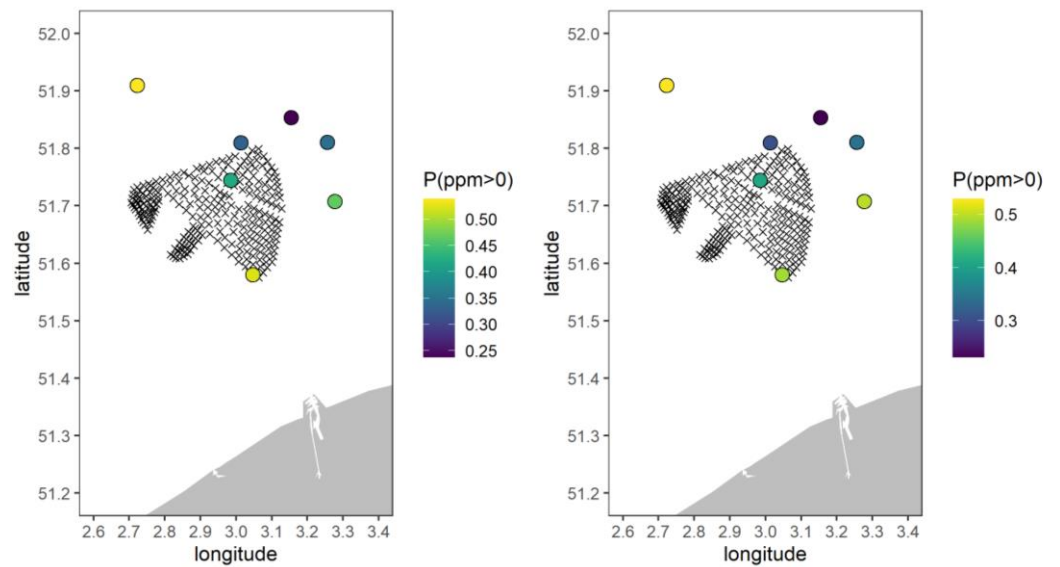
Figure F.5 Predictor effect plot of the random intercept for location for the regular SPL Bernoulli models. The left plot is from the VHF-weighted SPL Bernoulli model, and the right plot from the unweighted SPL Bernoulli model. The large points indicate the random effects, the crosses indicate the positions of the piling locations, and a small part of the land mass is visible to the south. The aspect ratio of the figure has been corrected for the longitude and latitude locations. The plots show the predicted probability of a porpoise positive minute (PPM), while ignoring the other smoothers (which average out to 0). The red dashed lines indicate the 95% confidence interval.
