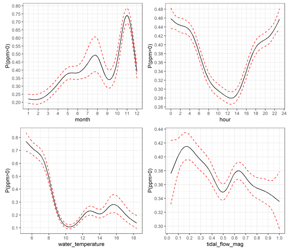
Figure D.10 Predictor effect plot of the regular smoothers for the distance based Bernoulli model. The plots show the predicted probability of a porpoise positive minute (PPM), while setting mdtps to -1 (meaning no piling), and ignoring the other random effects/smoothers (which average out to 0). The red dashed lines indicate the 95% confidence interval.
