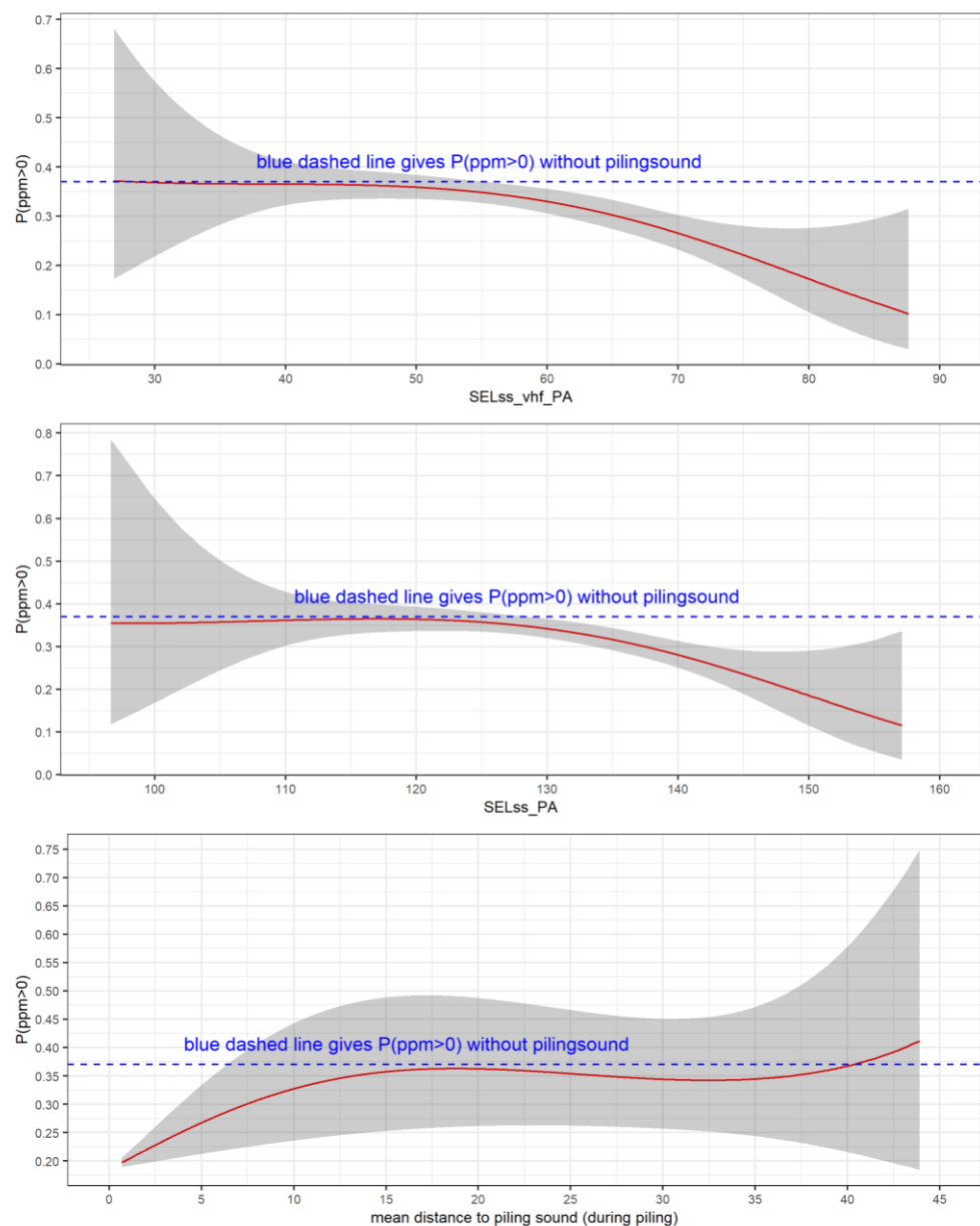
Figure 23 Comparison of the main effects of the three Bernoulli models for the Borssele data. Upper: VHF-weighted \text{SEL}_{\text{ss, VHF}}(50\text{-}500\text{Hz}) ; Middle: unweighted \text{SEL}_{\text{ss}}(50\text{-}500\text{Hz}) ; Lower: distance to pile. The blue dashed lines give the average probability for detection porpoise clicks ( \text{PPM}/h > 0 ) in the area based on a model for the time periods in which no piling took place. The shaded area indicates the 95% confidence interval of the model predictions. Note that the vertical scales of the plots differ.
