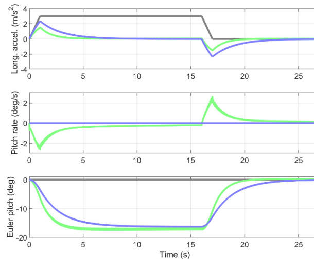
Figure 2. Output of the SOMS model (blue lines) and the Observer model (green lines) in response to a stepwise increase in longitudinal acceleration (gray line in upper panel) representative of a “static” takeoff run, where the engines are set at takeoff thrust with the brakes on and the aircraft starts to accelerate as soon as the brakes are released. The upper, middle, and lower plots show, respectively, longitudinal acceleration, pitch rate, and Euler pitch angle.
