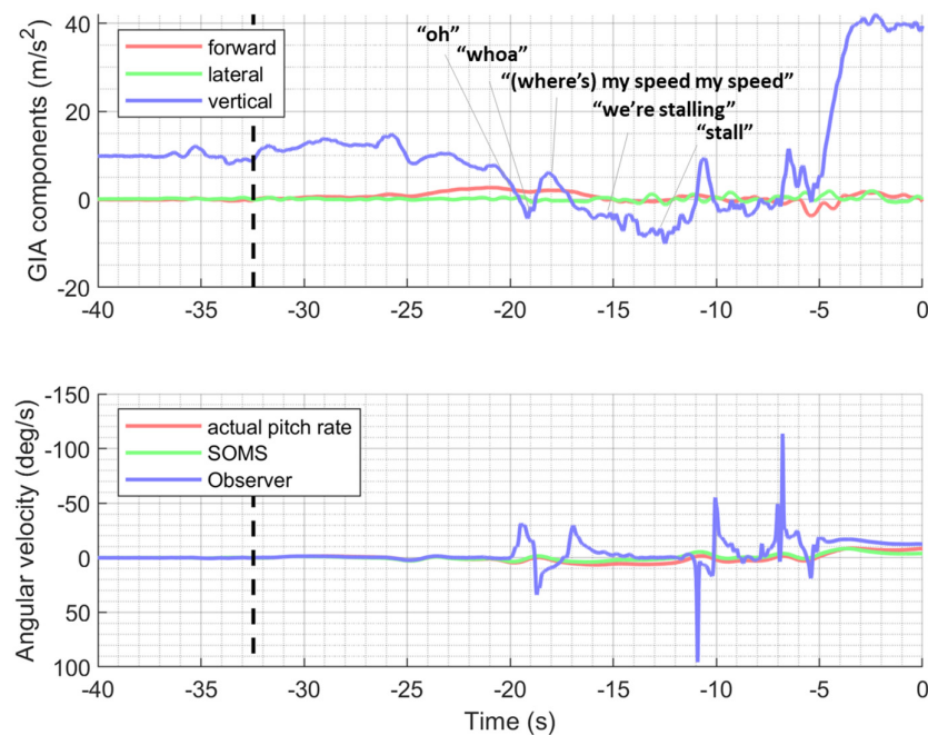
Figure 5. Time histories of the recorded GIA components (upper panel, \text{m/s}^2 ) and actual and predicted pitch rate (lower panel, \text{deg/s} ). The PF's callouts in the upper panel were copied from Appendix D within reference [1].
