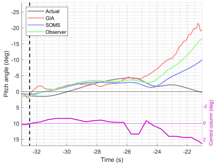
Figure 4. The same time histories as in Figure 3 but zoomed in between -33 and -21 s.
