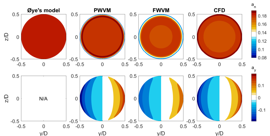
Figure 3. Induction field at the actuator disc on the axis normal to disc and y axis from different models when yaw angle = 0 deg and C_T = 0.6 .
