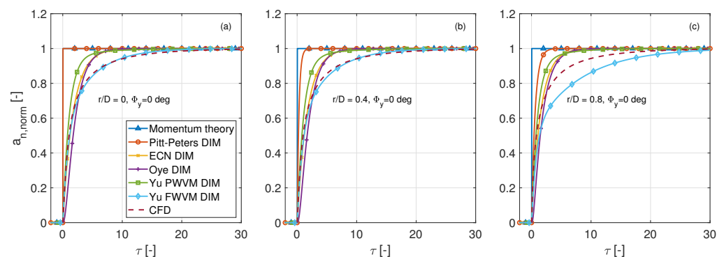
Figure 5. Normalized induction factor a_{n, norm} at different positions when base C_T = 0.6 , \Delta C_T = +0.1 , \Phi_y = 0 deg, (a) r/D = 0 (b) r/D = 0.4 (c) r/D = 0.8 , \tau is Non-dimensionalized time \left(\frac{tU_0}{R}\right) .
