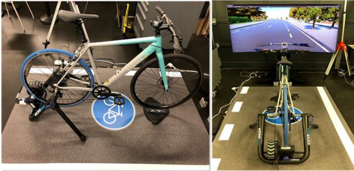
Figure 9. Virtual reality bicycle simulator
