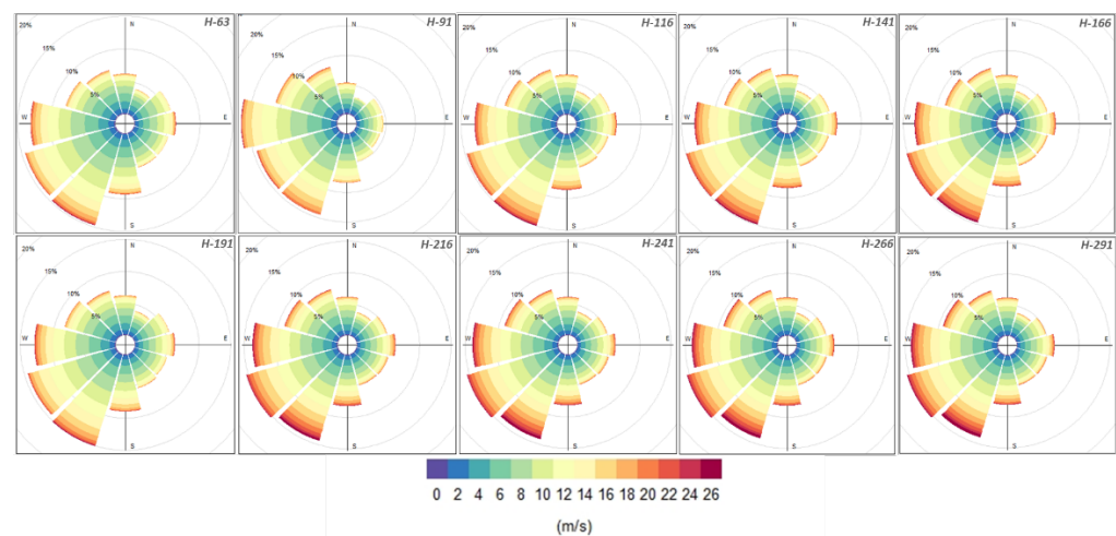
Figure 5 Wind roses at different heights showing the wind prevailing direction for the 2016 -2020 period.
