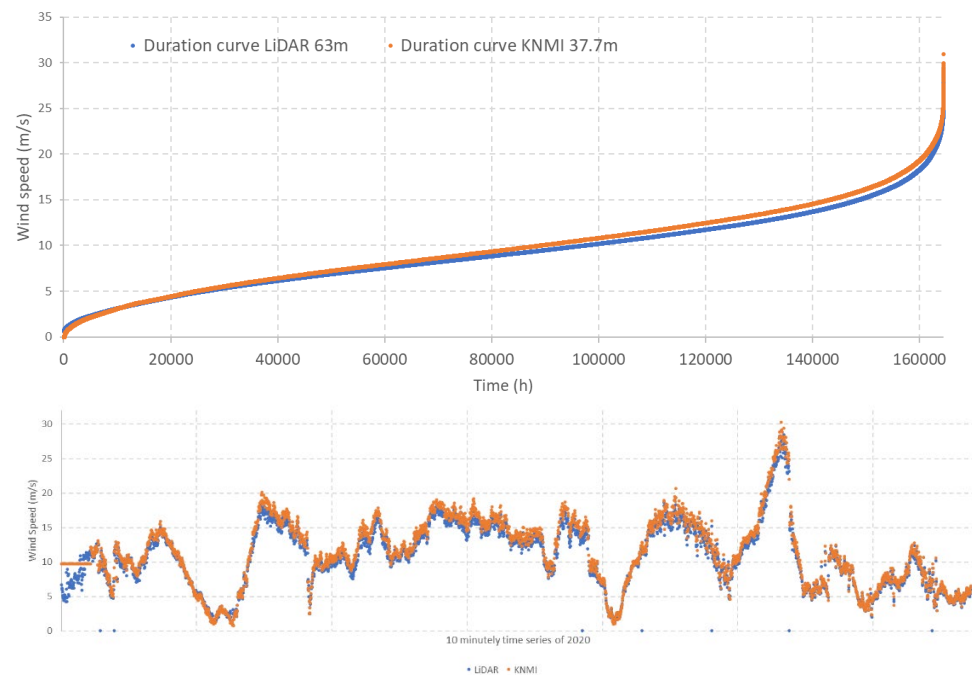
Figure 13 Comparison of the (top) wind speed duration curves for 2016-2020 and (bottom) time series 2020 between LiDAR (blue) and KNMI (orange) measurements at the K13a platform.
