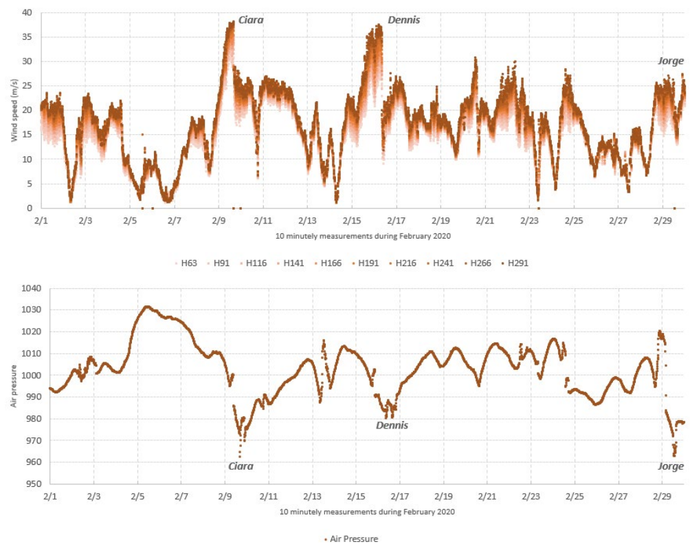
Figure 19 (Top) Wind speed (m/s) at different heights and (bottom) air pressure (hPa) measured at K13a during February 2020.
