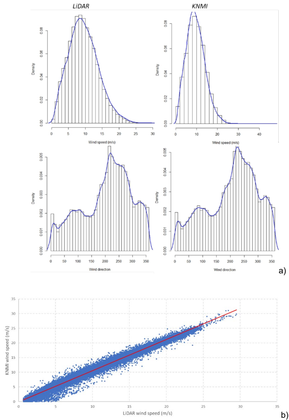
Figure 12 (a) Distribution histograms the wind speed (m/s) and wind direction (°) between the LiDAR at 63 m height and KNMI at 37.7 m height measurements at the K13a platform, before the filtering of the outliers; b) scatter plot between LiDAR (x-axis) and KNMI measurements (y-axis) after the filtering of the outliers.
