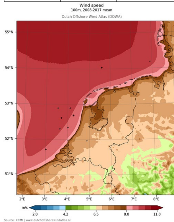
Figure 11 100 m mean wind speed between 2008-2017 provided by the Dutch Offshore Wind Atlas.
