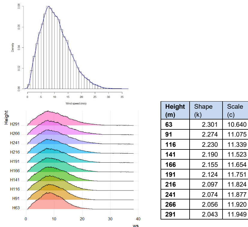
Figure 6 (top) Weibull distribution and curve fitting at 141 m height and (bottom) Weibull distributions at different heights for the measurement campaign with k and c parameters (table) at K13a for 2016-2020.
