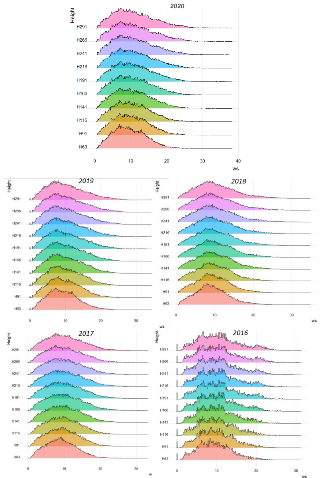
Figure 9 Annual Weibull distributions at different heights at the K13a platform for the 2016-2020 period. Note that 2016 indicates larger wind variability since only two months are considered (the campaign started on the 1 st of November 2016).
