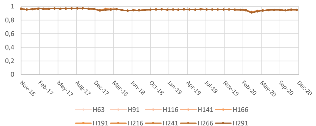
Figure 4 Monthly averages of the data available (%) measured by the ZX 300M LiDAR by height at the K13a platform.
