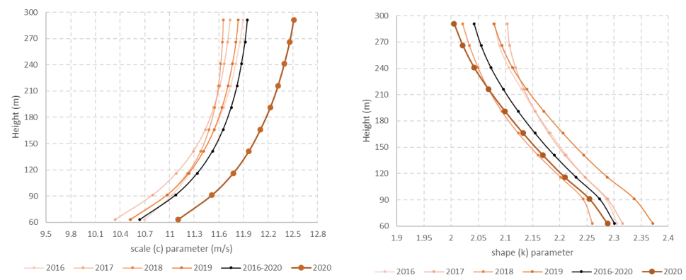
Figure 8 Annual Weibull (left) scale and (right) shape parameters at different heights at the K13a platform from 2016 to 2020.
