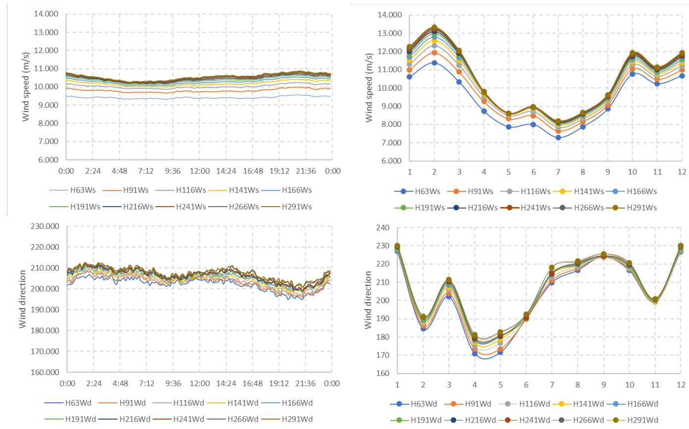
Figure 7(right) Monthly wind speed and direction averages and (left) daily cycle averages at different heights for the 2016-2020 period.
