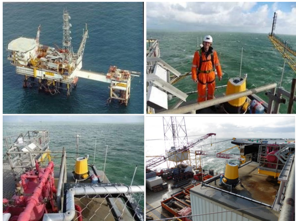
Figure 3 a) Front of K13a platform (geographical coordinates 51° 56'N, 3° 40'E); b) c) and d) location of the LiDAR installation.
