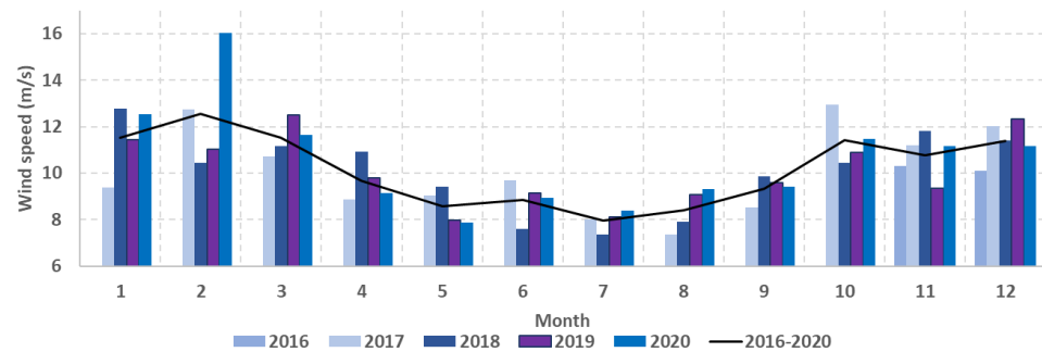
Figure 10 Annual wind speed (m/s) monthly averages bars at 141 m height and 2016-2020 monthly average (black line).
