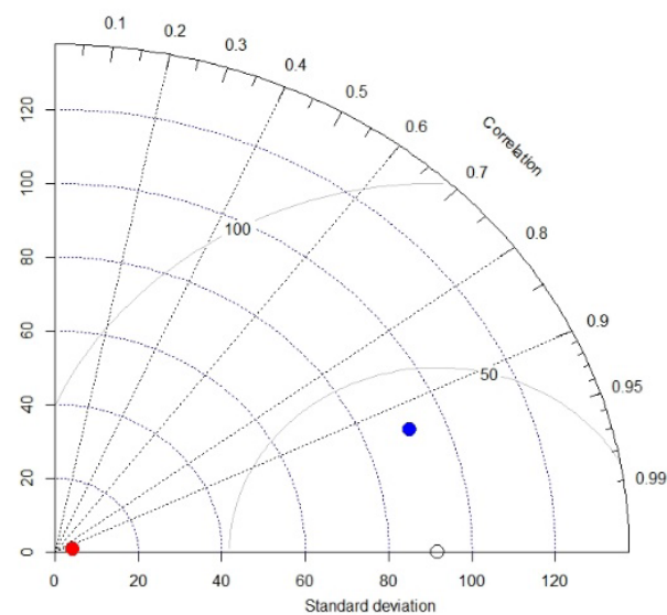
Figure 14 Taylor diagram for wind speed (red) and wind direction (blue) for KNMI as reference and LiDAR at the K13a platform. X and Y axis represent the Standard deviation, white marker represent normalized standard deviation with RMSE ~ 0 and correlation =1.
