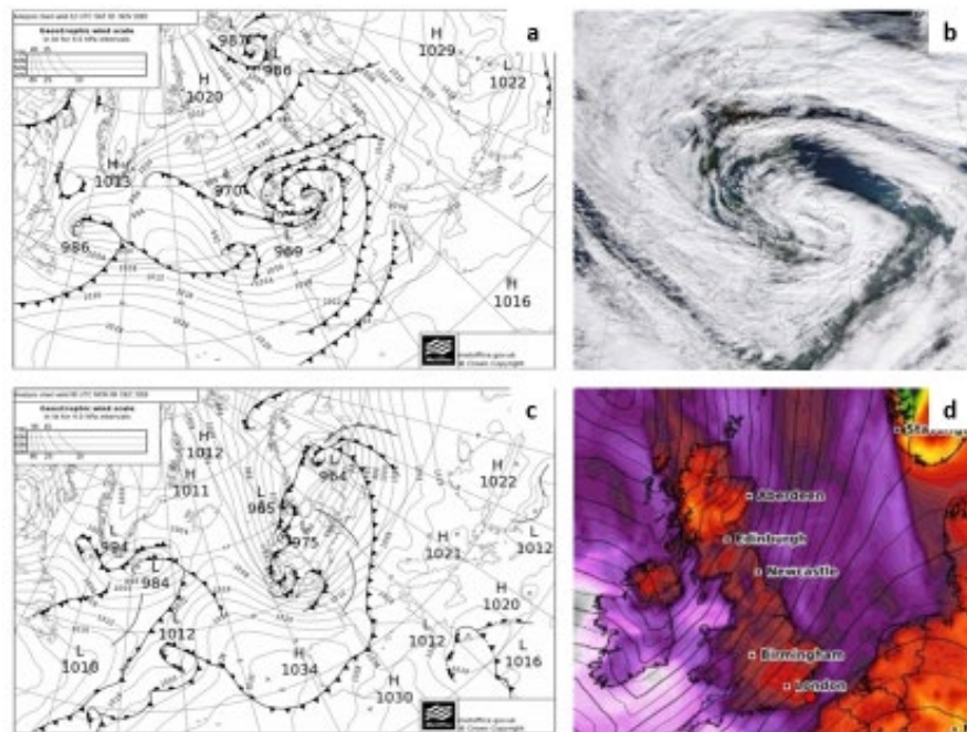
Figure 18 Analysis chart (a) and satellite image (b) over the North Sea UK and Dutch coast on the 2 nd of November 2016. C) isobars and d) zooming out the isobars over UK and The Netherlands representing the Atiyah storm on the 8 th of December 2019 [image extracted from the Met Office, UK, copyright Met Office / NASA/ NOAA].
