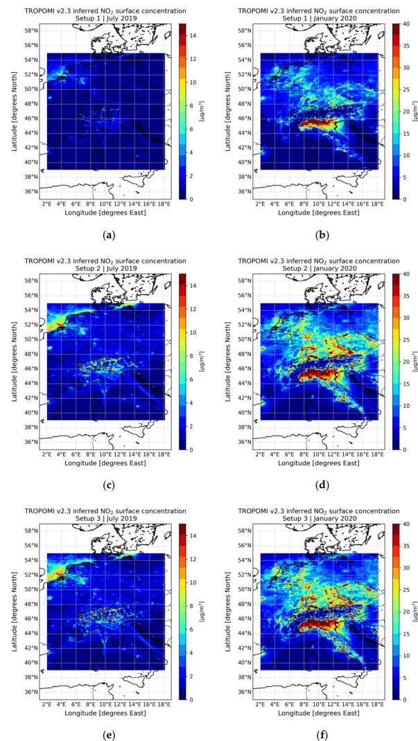
Figure 4. Mean TROPOMI v2.3 inferred \text{NO}_2 surface concentrations (in \mu\text{g}/\text{m}^3 ) for July 2019 (left column) and January 2020 (right column) for each setup, calculated using the (a,b) LOTOS-EUROS model output; (c,d) LOTOS-EUROS output after application of the TM5-MP averaging kernels; (e,f) TROPOMI and LOTOS-EUROS products after application of the CSO AMFs.
