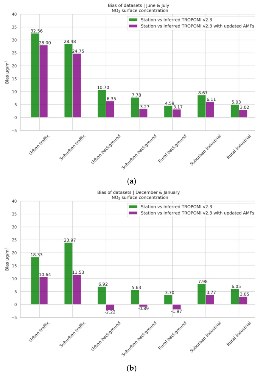
Figure 11. Absolute bias (in \mu\text{g}/\text{m}^3 ) between the in situ measurements and the inferred TROPOMI v2.3 NO 2 surface concentrations for the first (green) and the third (purple) setups: (a) summer; (b) winter.
