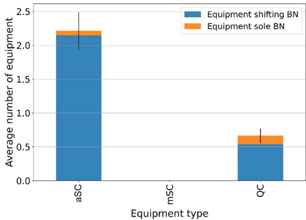
Fig. 7 Results of application of the shifting bottleneck method using 30 aSCs, 24 mSCs, 2 QCs and a truck workload of 81 boxes per hour with a 5-percent significance level. BN bottleneck
