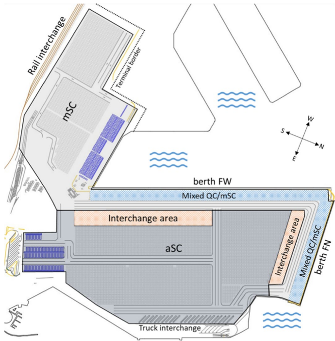
Fig. 4 Operating areas of the different types of equipment present at the Fergusson Container Terminal. mSC manned straddle carrier, aSC automated straddle carrier, eQC quay crane
