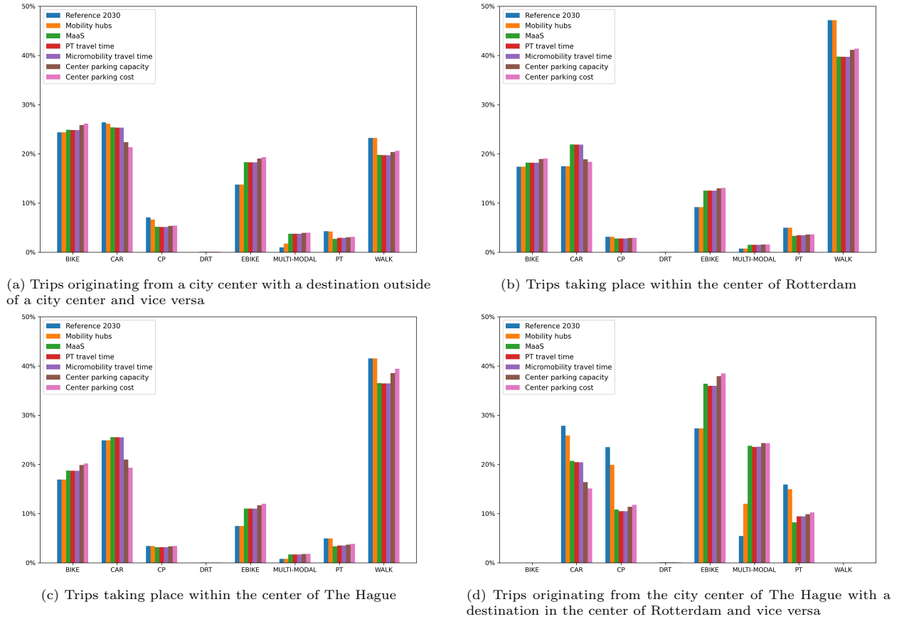
Figure 5: Bar charts representing the modal split for several subsets of the simulated trips
