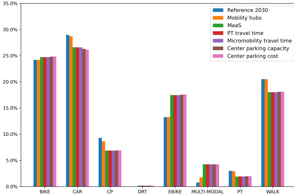
Figure 4: Bar chart representing the modal split of all simulated trips in the MRDH region under the various scenarios
