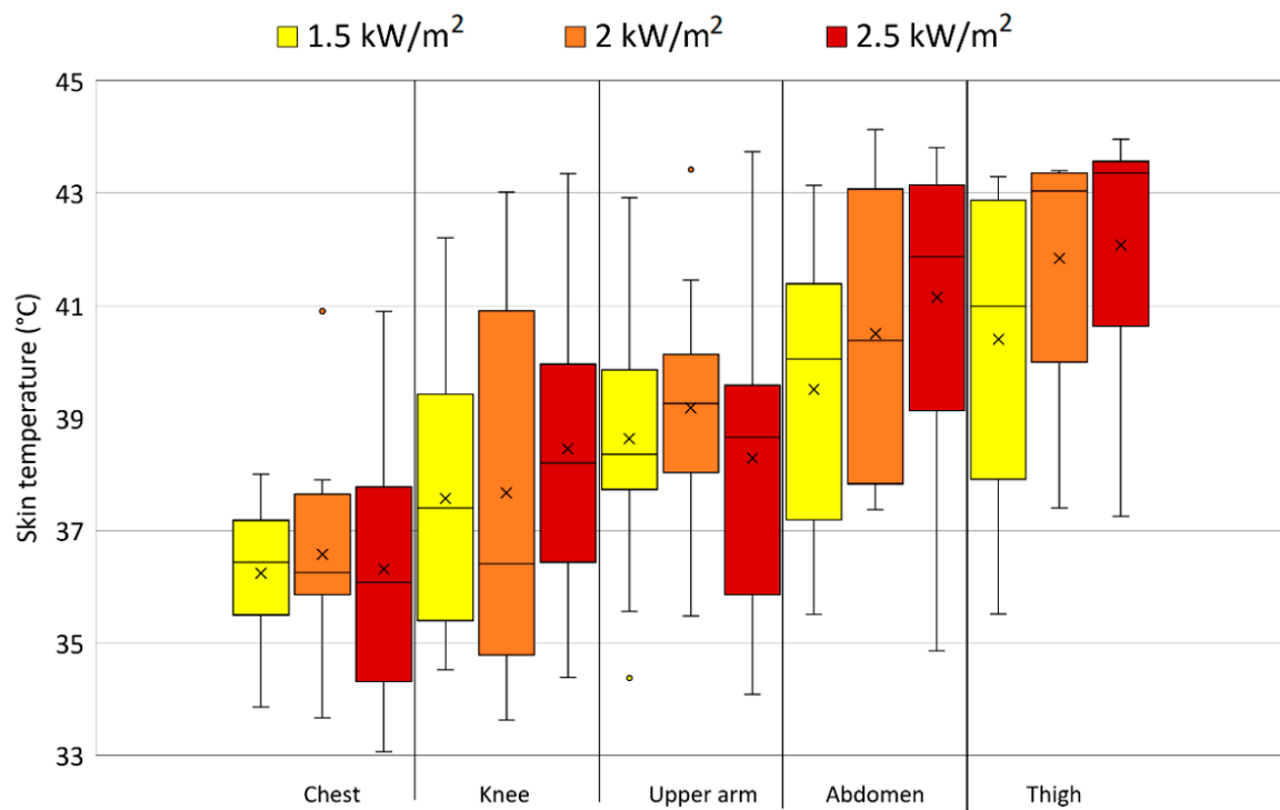
Figure 6. The median (horizontal line) and mean (×) highest measured skin temperatures with the standard deviations and the outliers (○) at the various body locations across the test persons at the different radiation intensities.
