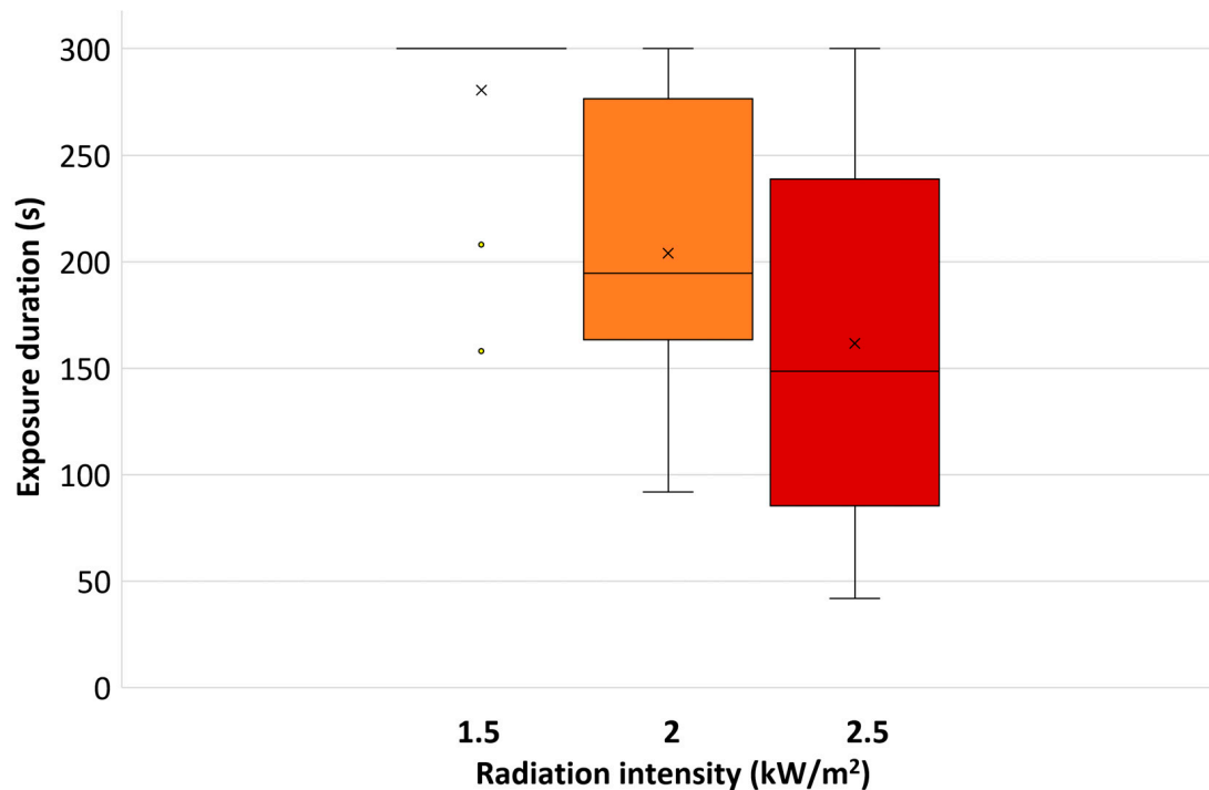
Figure 5. The median (horizontal line) and mean (×) exposure times with the standard deviation and the outliers (o) at the different radiation intensities.
