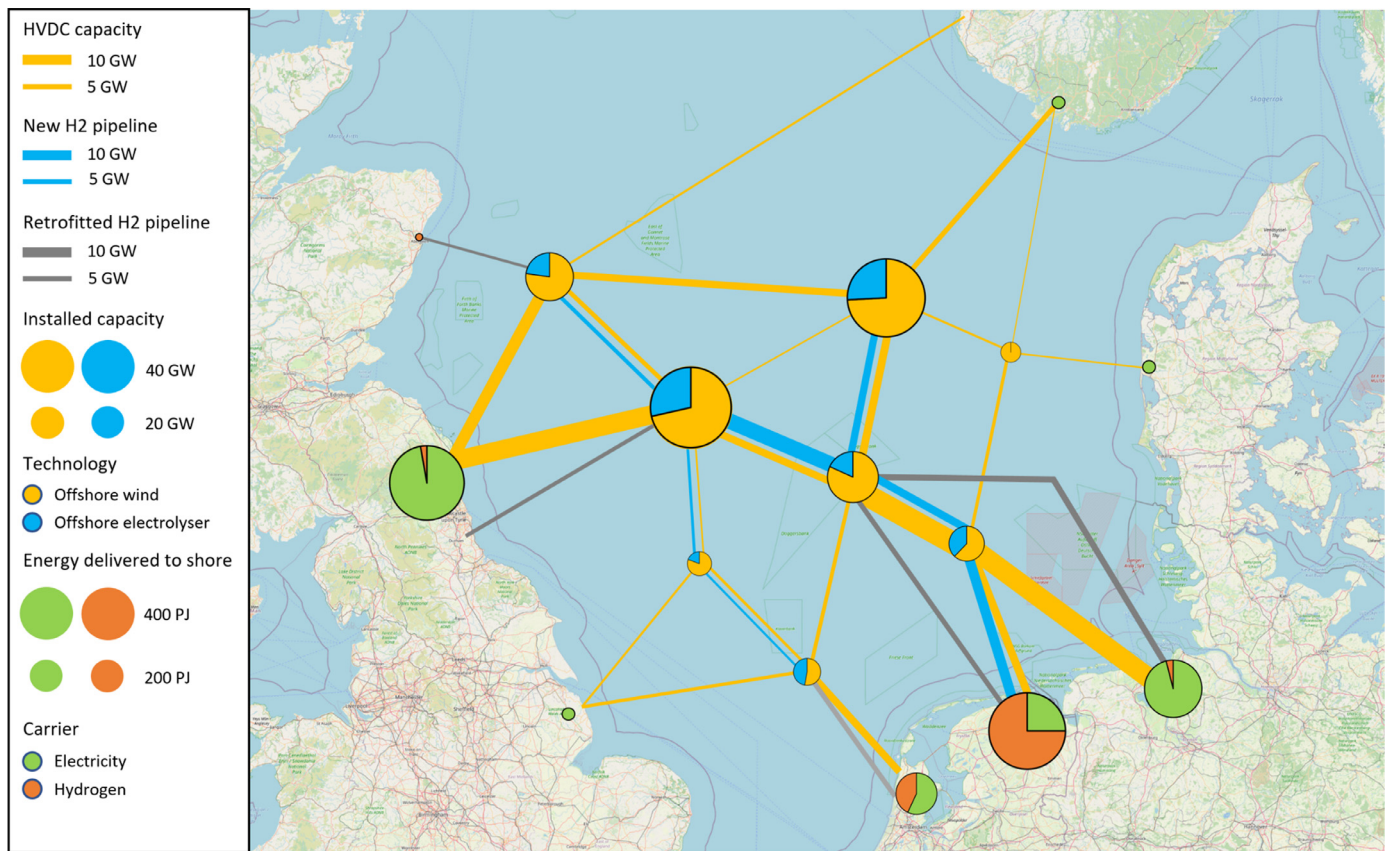
Fig. 16. Optimal investments in HVDC interconnectors and OWPP capacity and in electrolyzers and hydrogen pipelines in H1.
