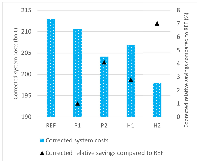
Fig. 22. Difference in total system cost across the NSOG scenarios compared to the base case.
