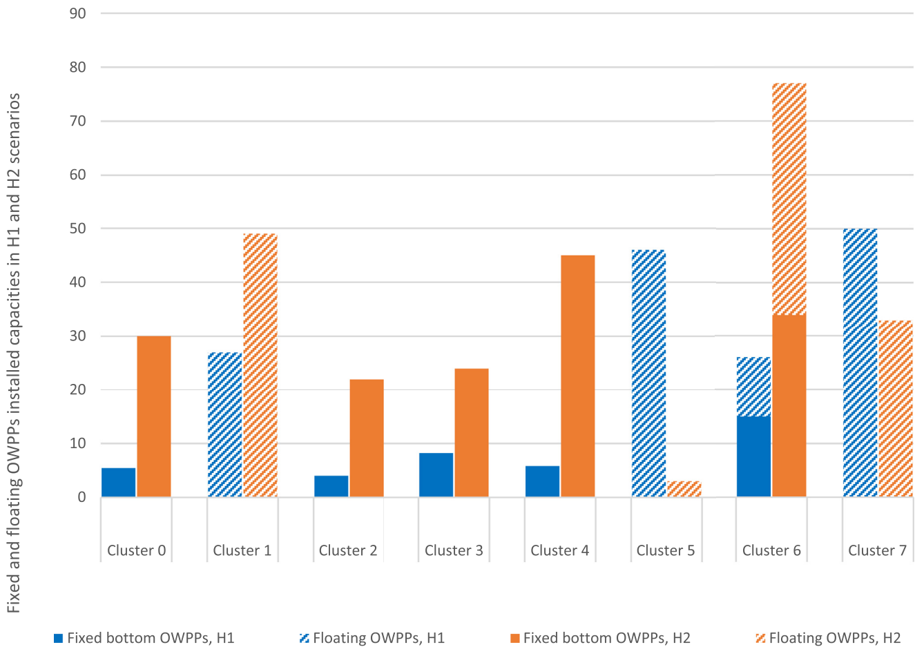
Fig. 18. Fixed-bottom and floating OWPPs installed capacities in the power and hydrogen NSOG scenarios.
