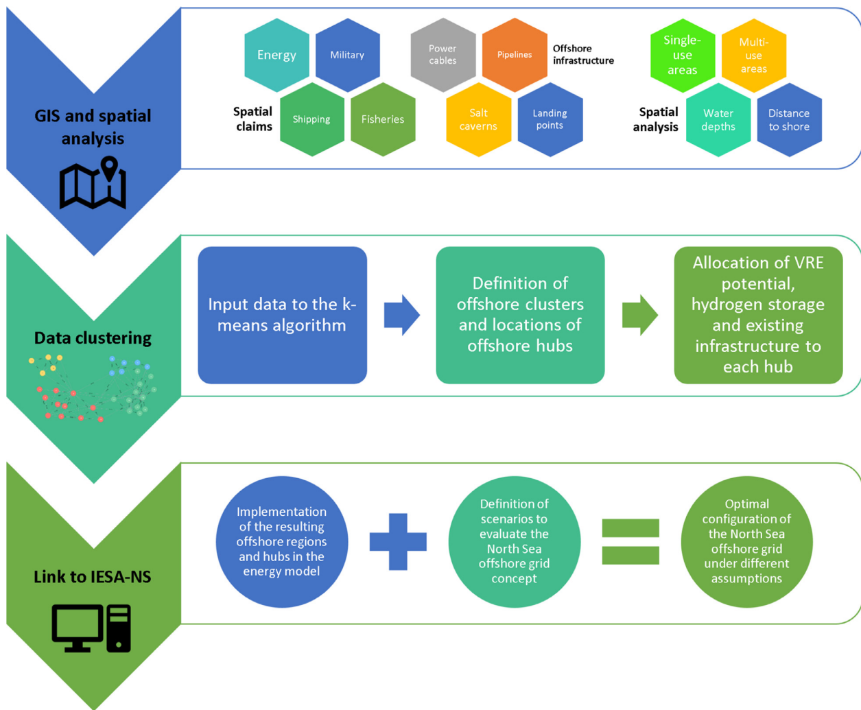
Fig. 2. Spatial clustering data, methodology and link to IES-NS.
