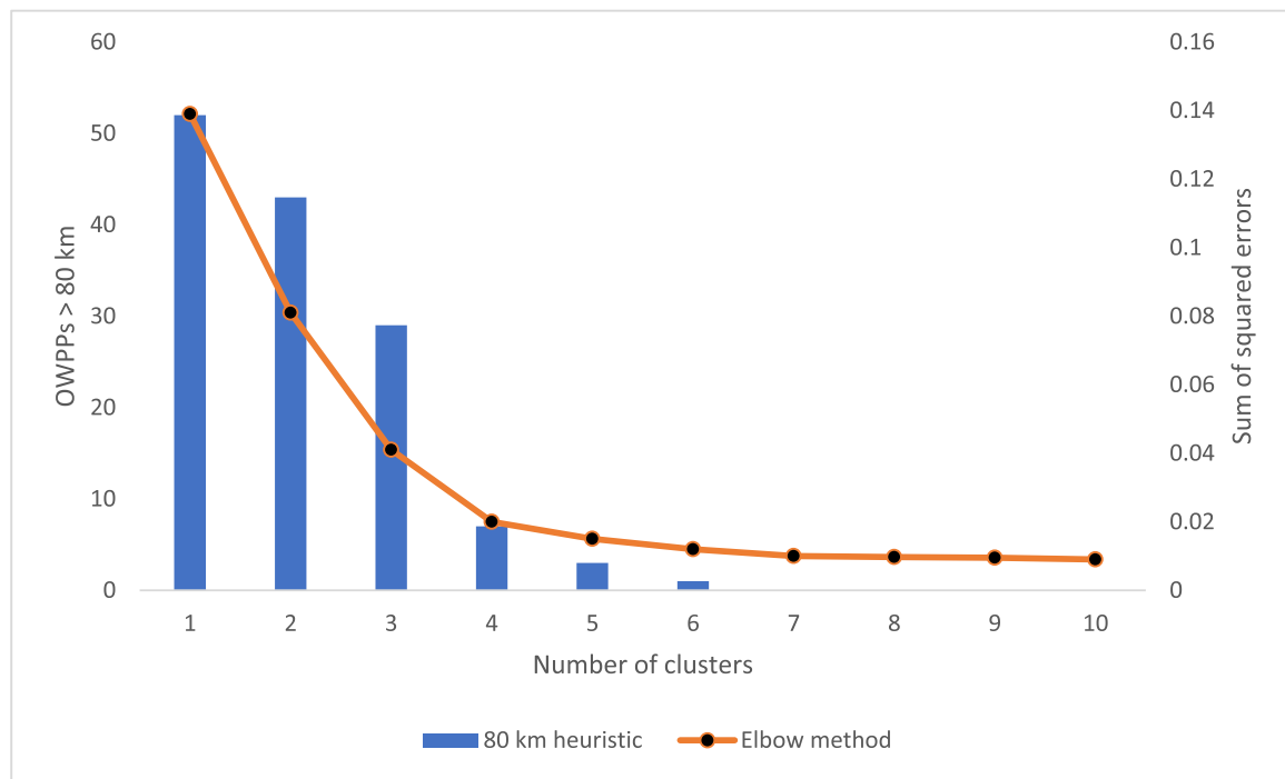
Fig. 6. Elbow method and 80 km heuristic results.
