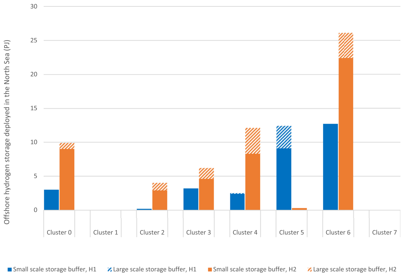
Fig. 20. Size (PJ) of the optimal hydrogen storage deployed in each of the offshore clusters.
