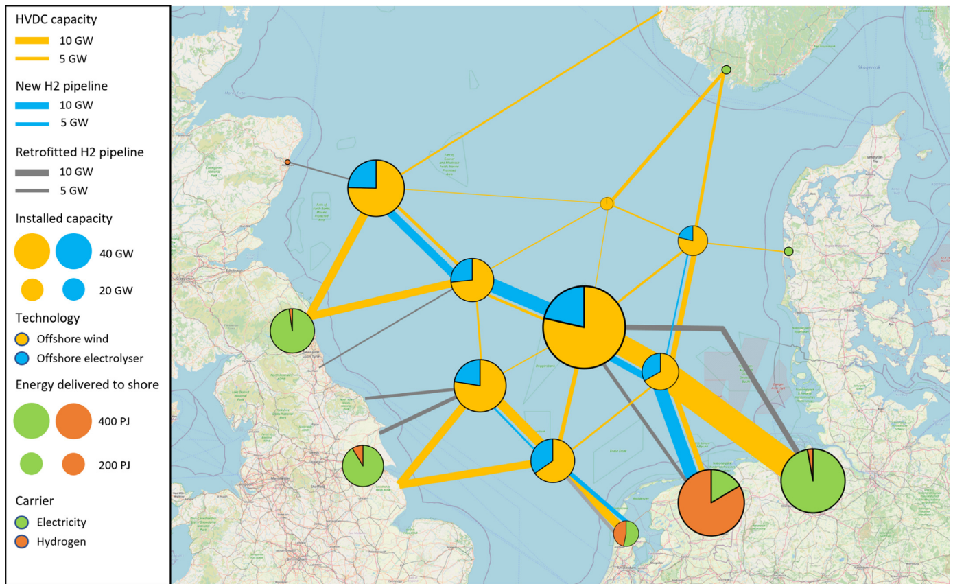
Fig. 17. Optimal investments in HVDC interconnectors and OWPP capacity and in electrolyzers and hydrogen pipelines in H2.
