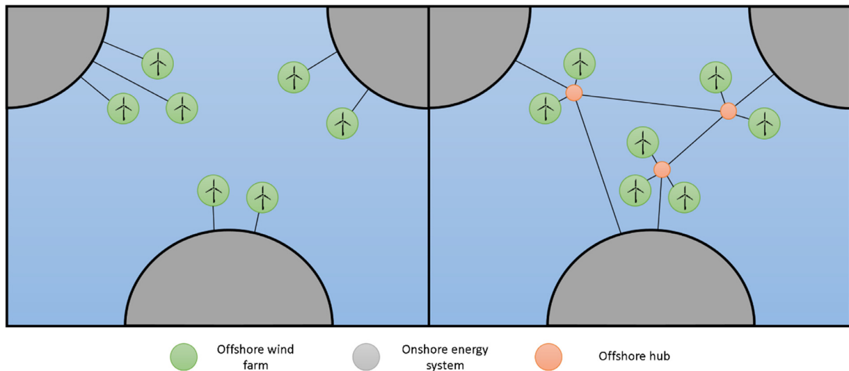
Fig. 1. Comparison between radial connection of OWPPs (left) and the NSOG concept (right).
