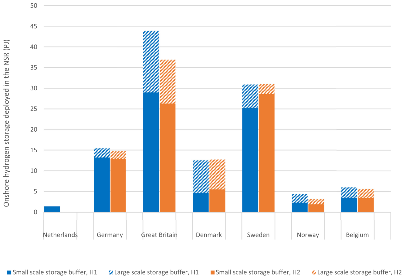
Fig. 21. Size (PJ) of the optimal hydrogen storage deployed in each NSR countries (onshore).
