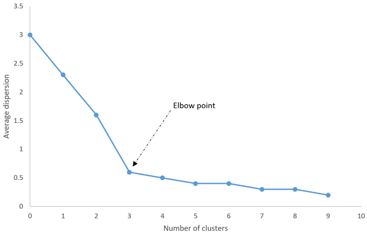
Fig. 24. Elbow method representation.
