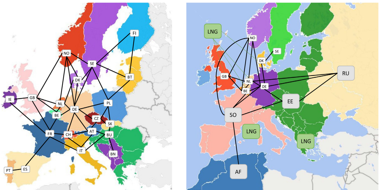
Fig. 3. European nodes and international interconnectors considered for the European power dispatch in IESA-NS (left) and European natural gas and LNG network considered in IESA-NS (right). Note that LNG stands for Liquefied Natural Gas.
