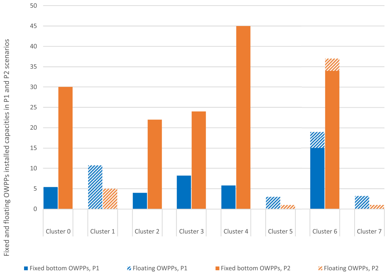
Fig. 15. Fixed-bottom and floating OWPPs installed capacities in the power NSOG scenarios.
