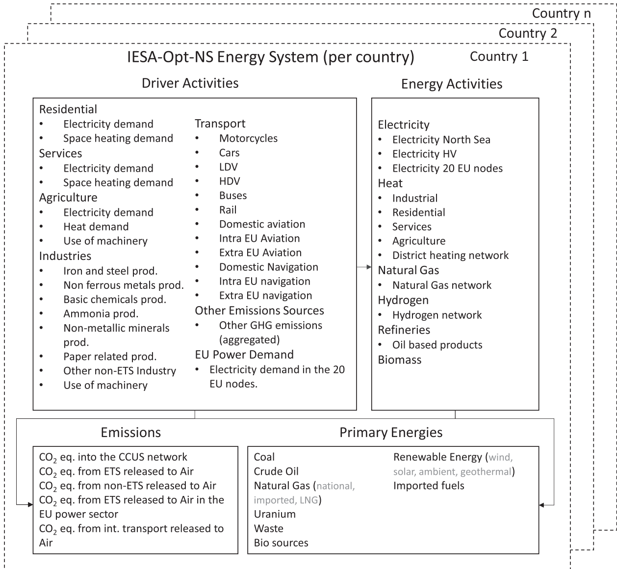
Fig. 26. Energy system representation of activities considered within the IESA-NS framework.
