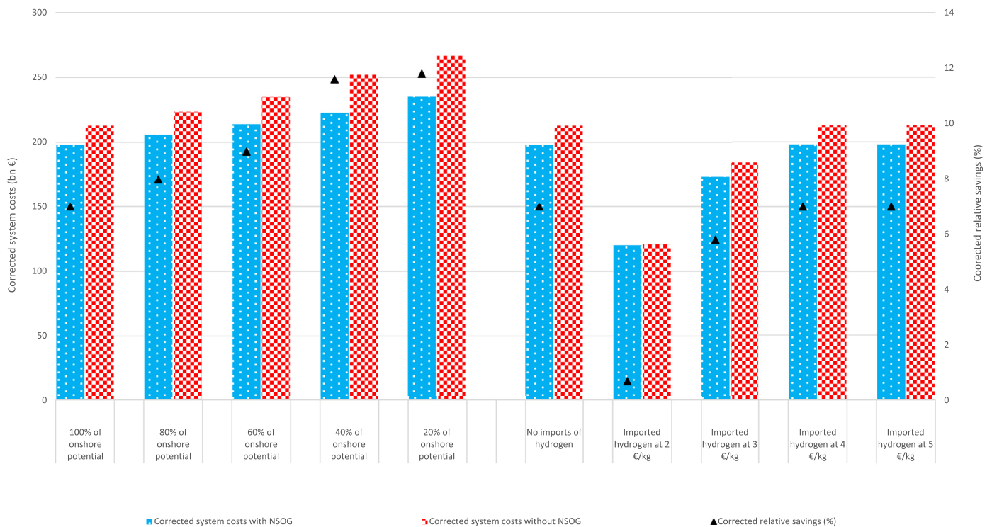
Fig. 23. Corrected system cost of the sensitivity analyses evaluated in this study.
