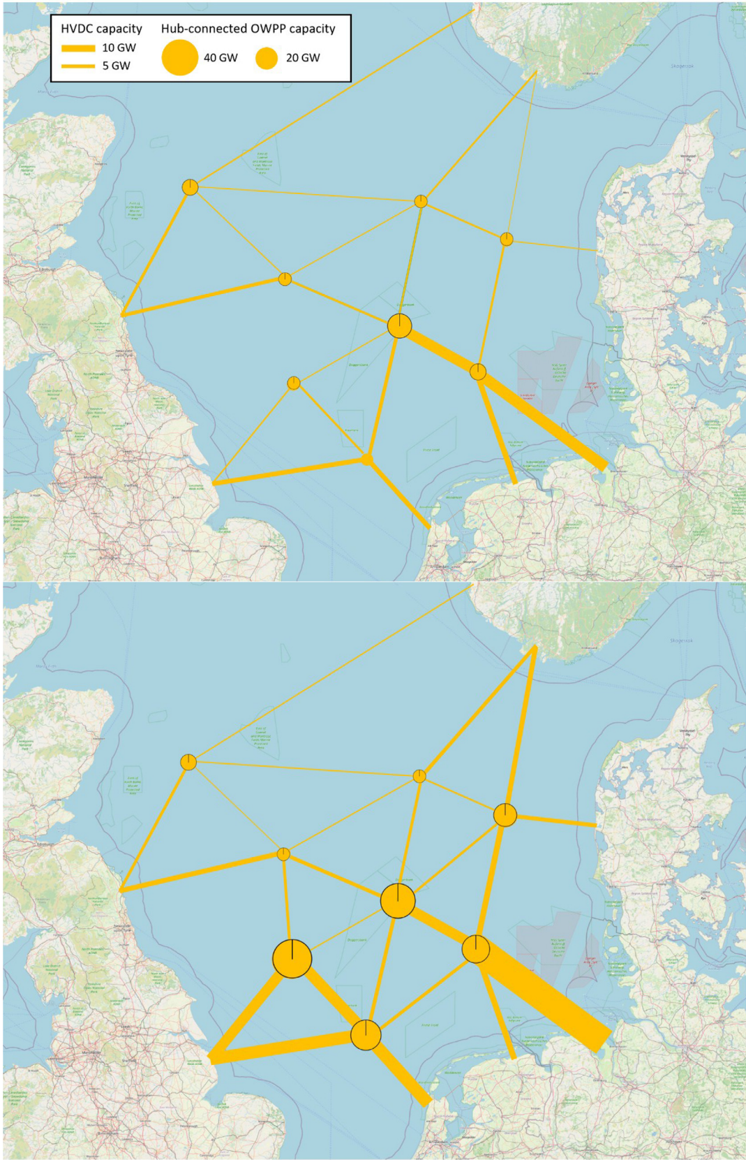
Fig. 14. Optimal investments in HVDC interconnectors and OWPP capacity. Data in GW. The diagram on top represents the scenario with reference OWPP density (P1), the diagram on the bottom represents the scenario with high OWPP density (P2).
