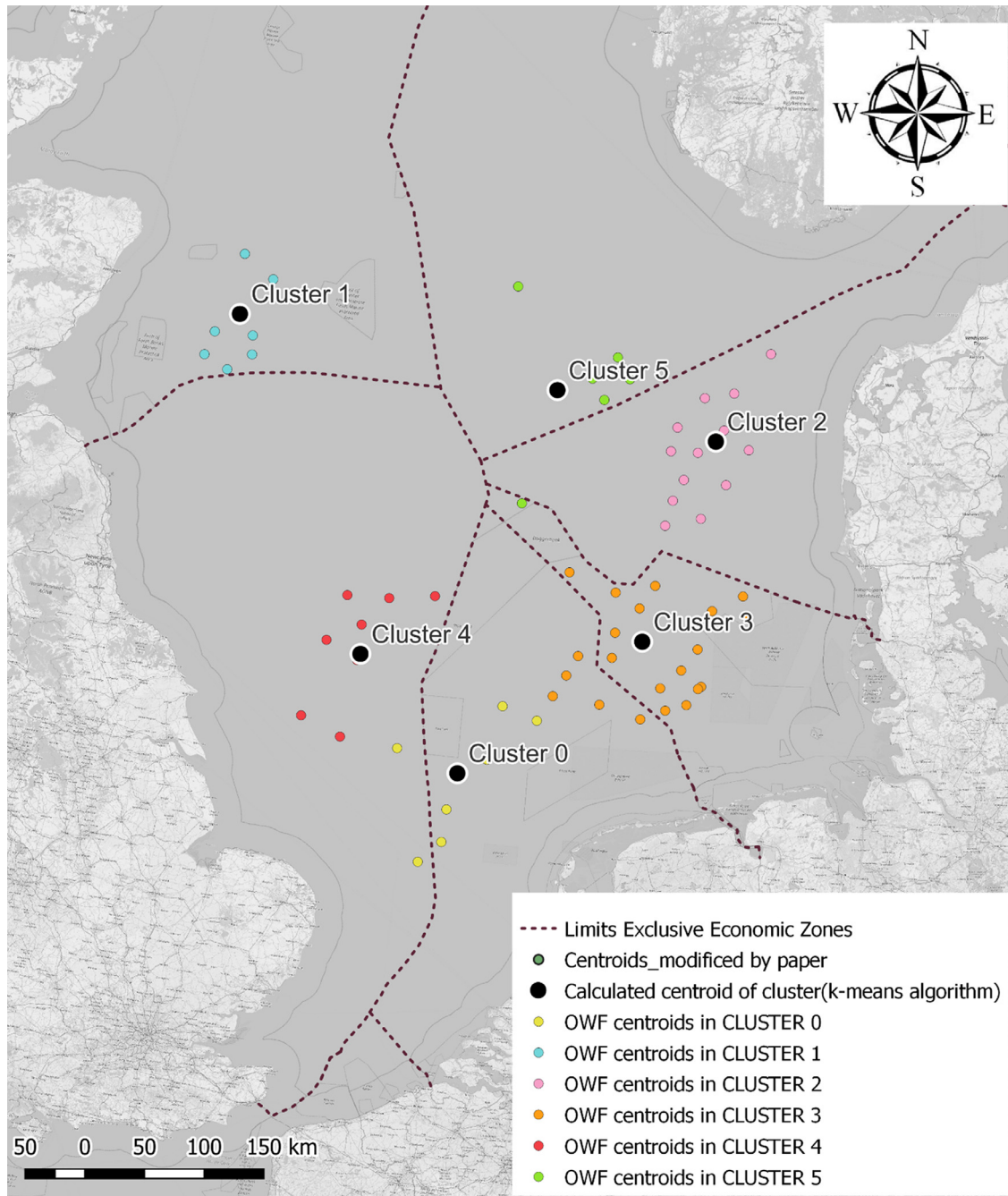
Fig. 7. Output of the k-means algorithm with 6 clusters.
