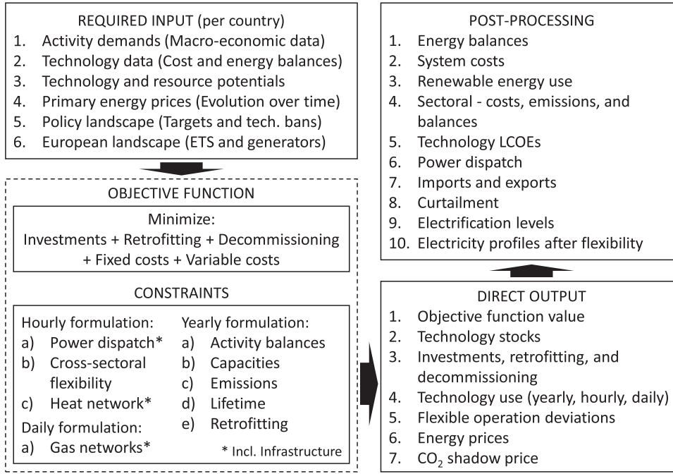
Fig. 25. Methodological elements in the IESA-NS framework.
