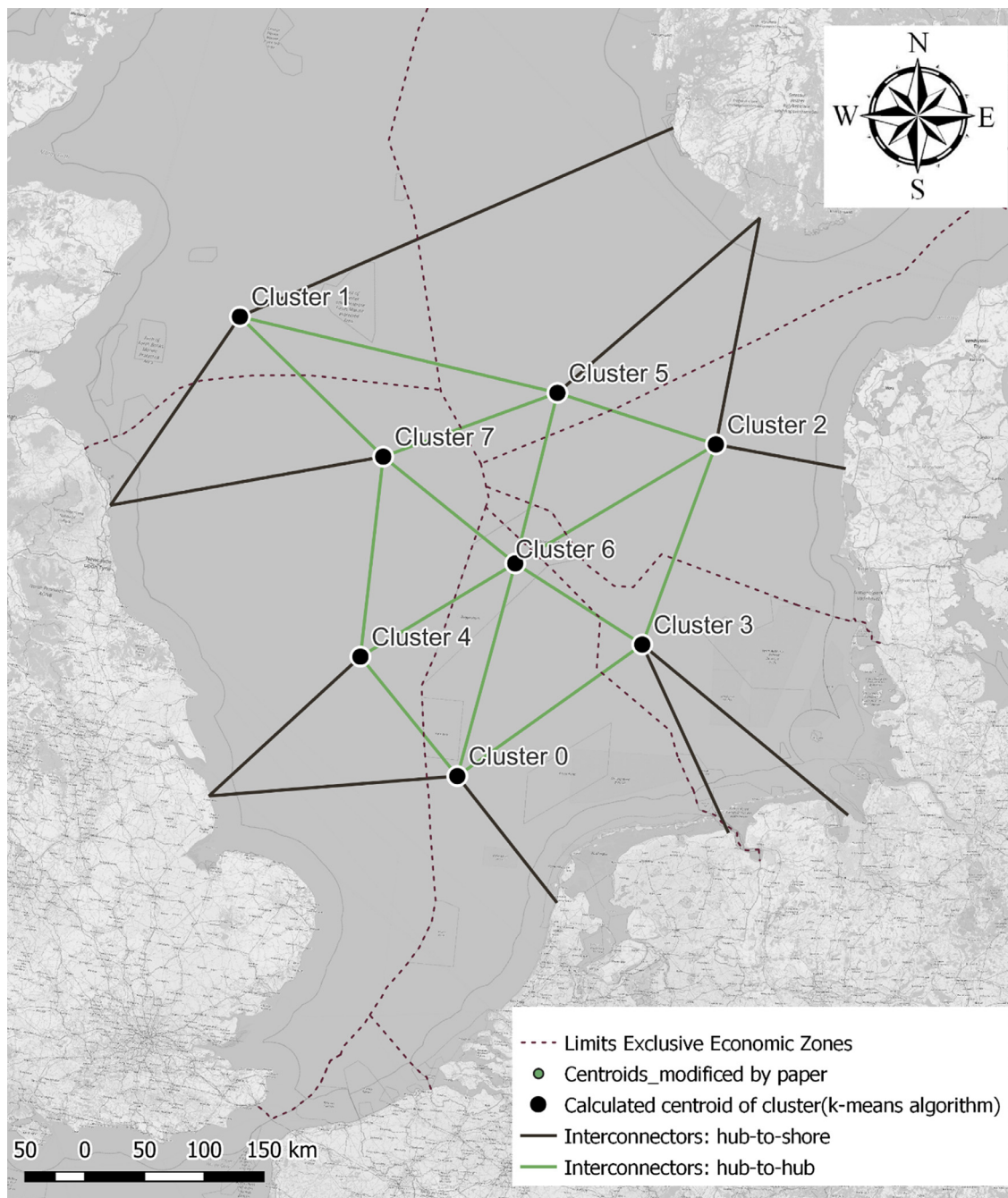
Fig. 11. NSOG interconnectors allowed, divided in hub-to-hub interconnectors (green) and hub-to-shore interconnectors (black). (For interpretation of the references to colour in this figure legend, the reader is referred to the web version of this article.)
