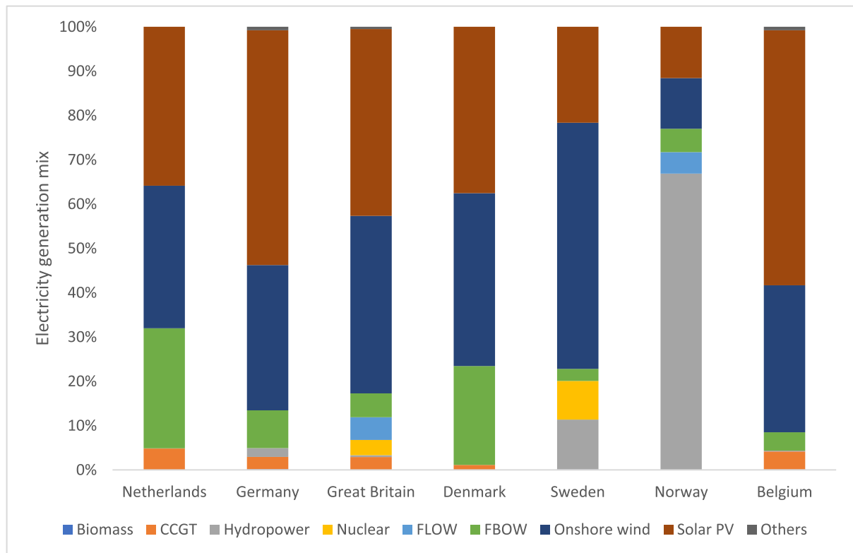
Fig. 12. Breakdown of the power generation in the reference scenario in the NSR countries in 2050.
