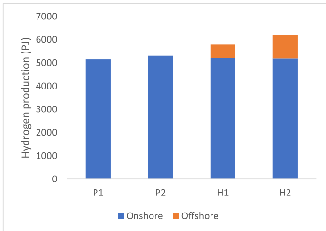
Fig. 19. Total onshore and offshore hydrogen production across the NSOG scenarios.
