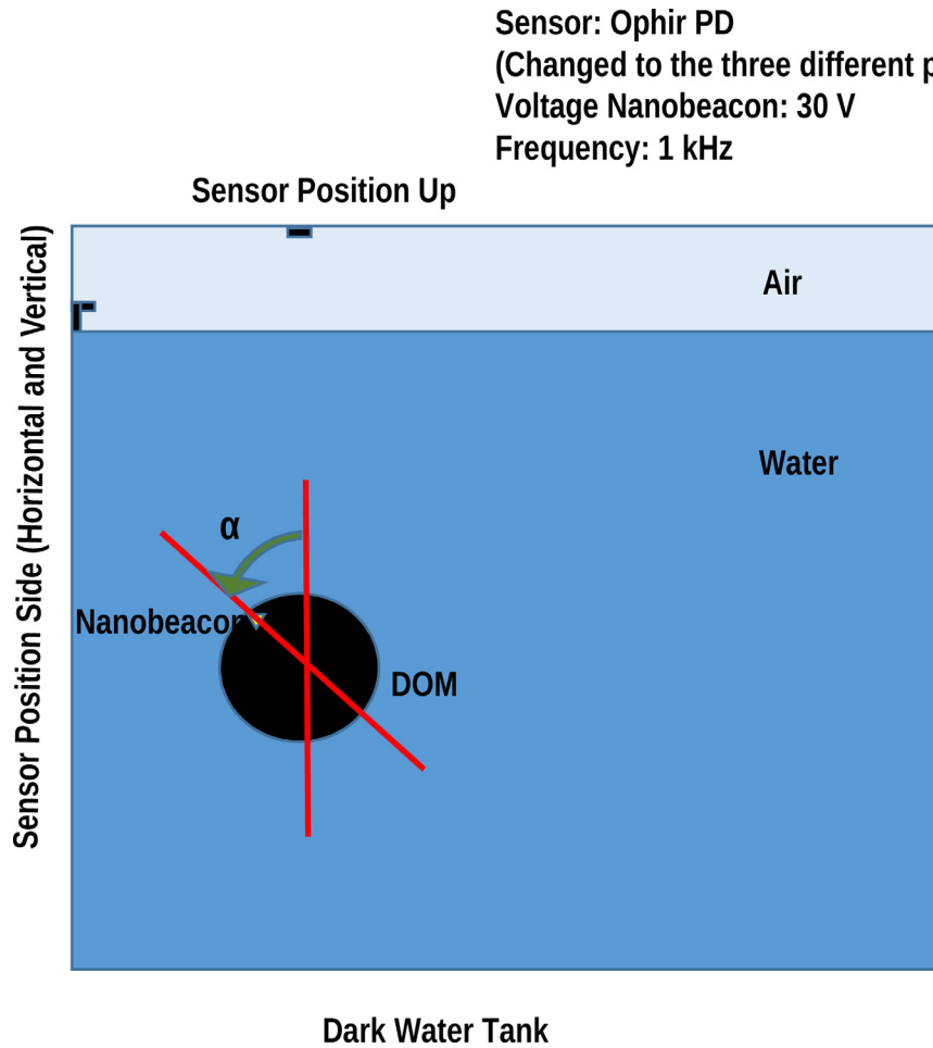
Fig. 6. Light-tight water tank setup. A DOM is submerged in the tank at a depth of approximately 2 m. The DOM can rotate, as shown in the figure. A light sensor is moved to three different positions on the upper part of the container, collecting the light emitted by the Nanobeacon being flashed in the DOM.
