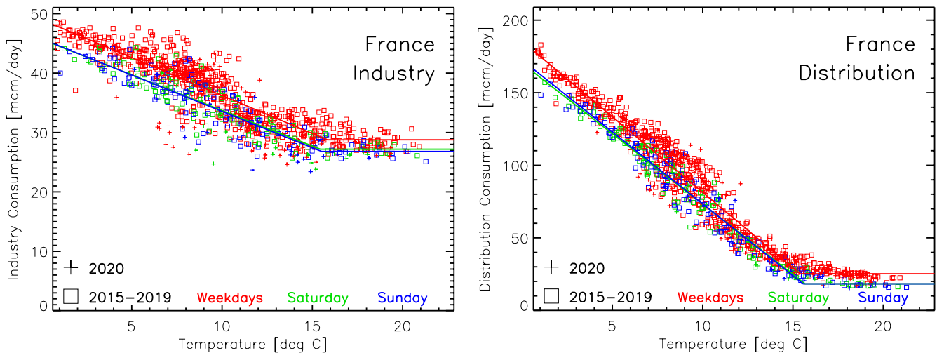
Figure 2. Daily gas consumption in France as a function of the effective temperature (see text) by the industry (left) and gas distribution to the built environment (right).
