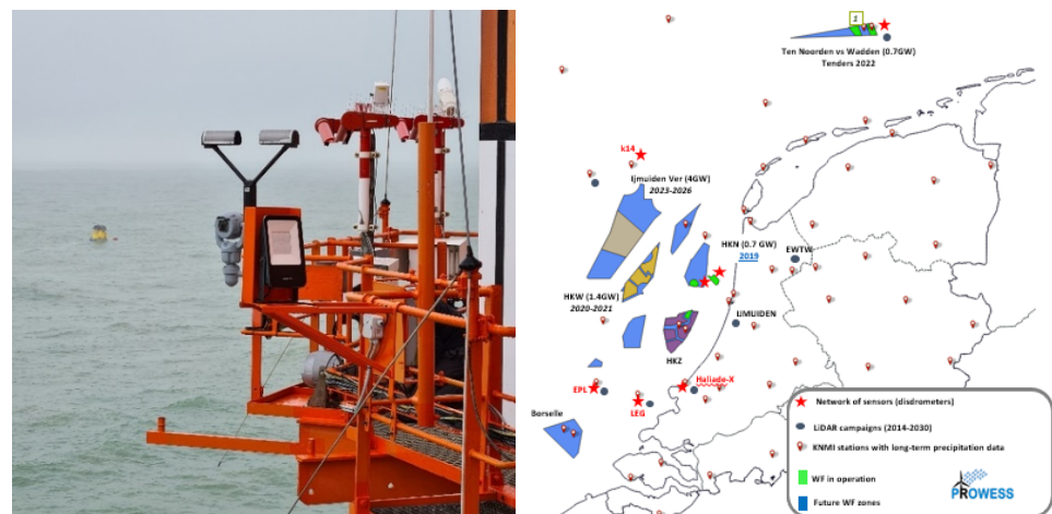
Figure 3 Disdrometer instrument installed at LEG platform (left), an additional disdrometer will be soon installed at EPL platform for the PROWESS project and the measurement campaign layout (right) for PROWESS project running from 2021 until 2023.
