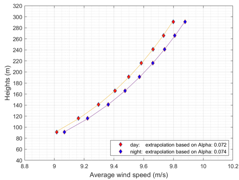
Figure 17 Day and night shear profile for the year 2021 at EPL
