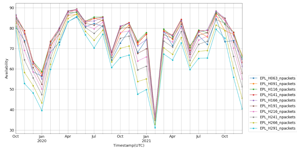
Figure 9 Monthly availability(%) over one LiDAR system measurement period
