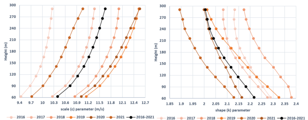
Figure 13 Annual Weibull (left) scale and (right) shape parameters at different heights at the EPL platform from 2016 to 2021.
