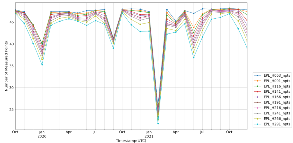
Figure 8 Monthly number of points measured over one LiDAR system measurement period
