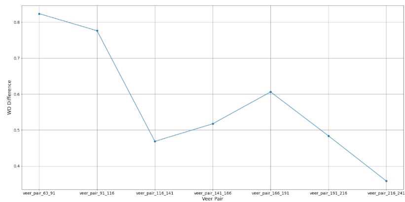
Figure 20 Annualized veer by LiDAR sensor pairing heights
