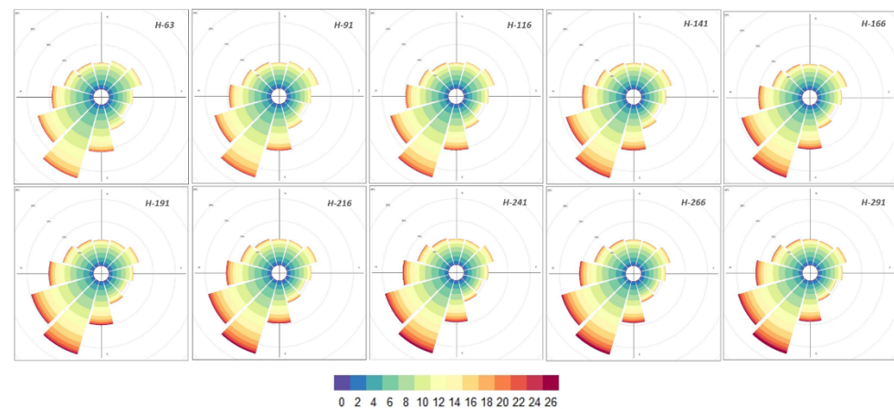
Figure 10 Wind roses at different heights showing the wind prevailing direction for the 2016 -2021 period.
