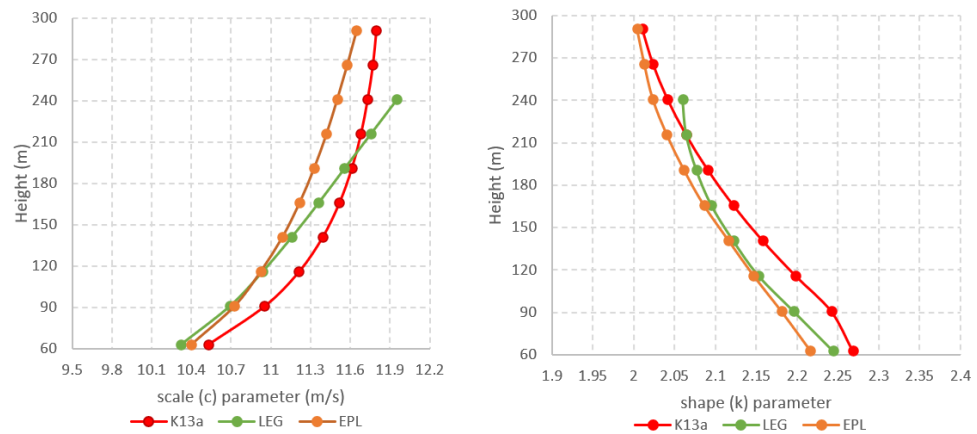
Figure 30 (left) Weibull distribution c and (right) k parameters for all heights at K13a, EPL and LEG over averaged 2016-2021 period.
