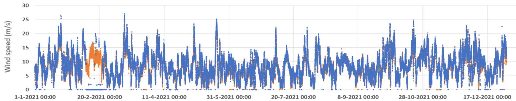
Figure 24 Time series wind speed for the year 2021 between LiDAR (blue) and KNMI (orange) measurements at the EPL platform
