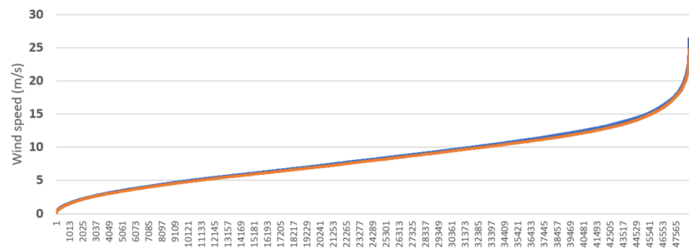
Figure 26 Wind speed duration curves for the 10-min average time stamps (x-axis) the period 2021, KNMI (orange) and LiDAR (blue)
