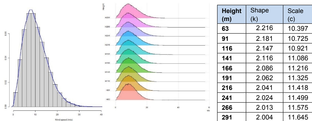
Figure 11 (left) Weibull distribution and curve fitting at 141 m height and (centre) Weibull distributions at different heights for the measurement campaign with k and c parameters (table) at EPL for 2016-2021.
