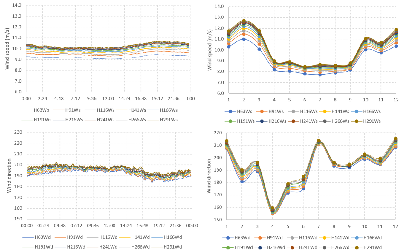
Figure 12 Monthly wind speed and direction monthly averages (right) and average daily cycles (left) at different heights for the 2016-2021 period.
