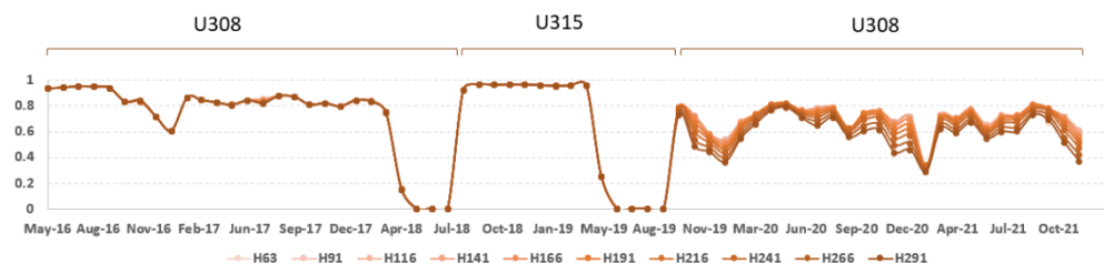
Figure 7 Monthly averages of the data available (fraction based) measured by the ZX 300 LiDAR by height at the EPL platform for the period 2016-2021.
