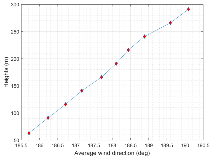
Figure 19 Variations in average wind direction for different sensor heights over the year 2021
