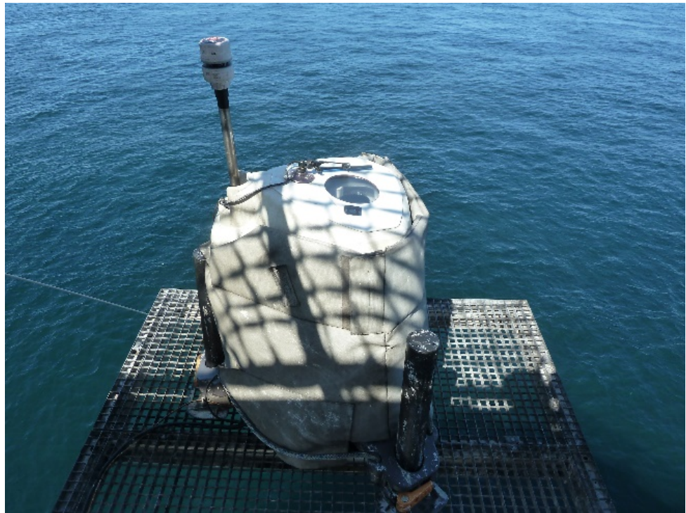
Figure 5 View of LiDAR unit for the scheduled maintenance period in 2020.
