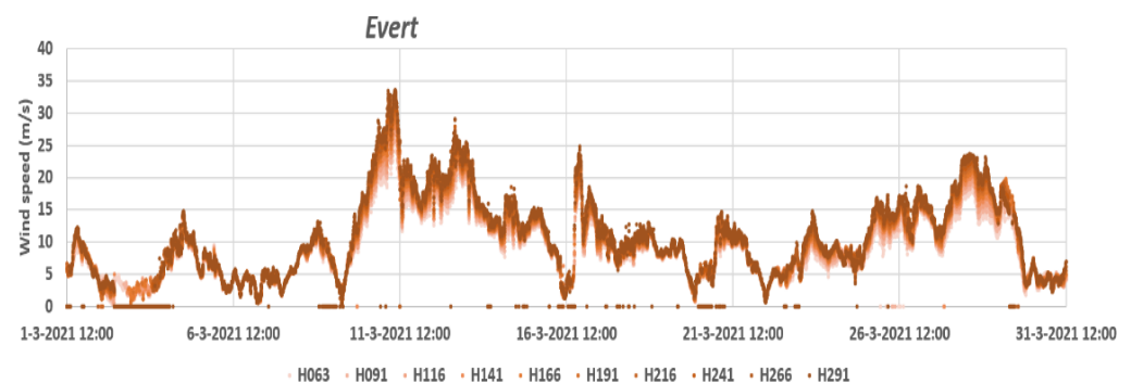
Figure 22 Time series of wind speed measured by the LiDAR at EPL platform during March 2021
