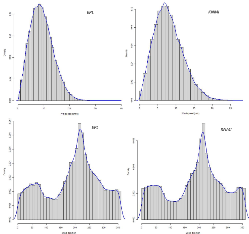
Figure 28 Distribution histograms the wind speed (m/s) (top) and wind direction (°) (bottom) between the LiDAR at 63 m height (left) and KNMI at 38 m height (right) measurements at the EPL platform for the year 2021.
