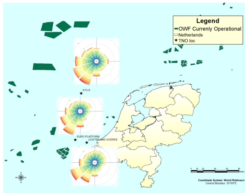
Figure 29 International and Dutch offshore wind farms currently operational and TNO measurement locations with wind roses at 141m for the 2016-2021 period
