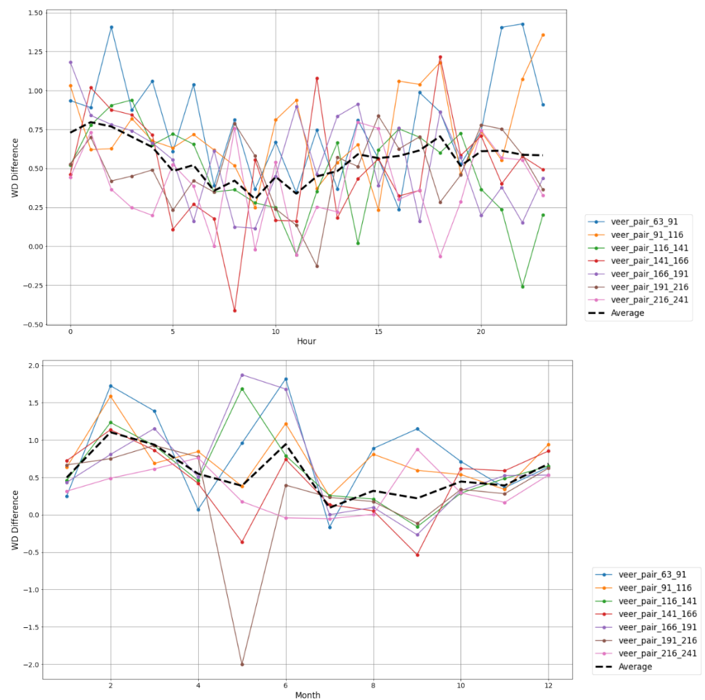
Figure 20 Annualized veer by LiDAR sensor pairing heights
