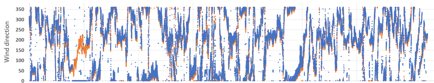
Figure 25 Time series wind direction for the year 2021 between LiDAR (blue) and KNMI (orange) measurements at the EPL platform
