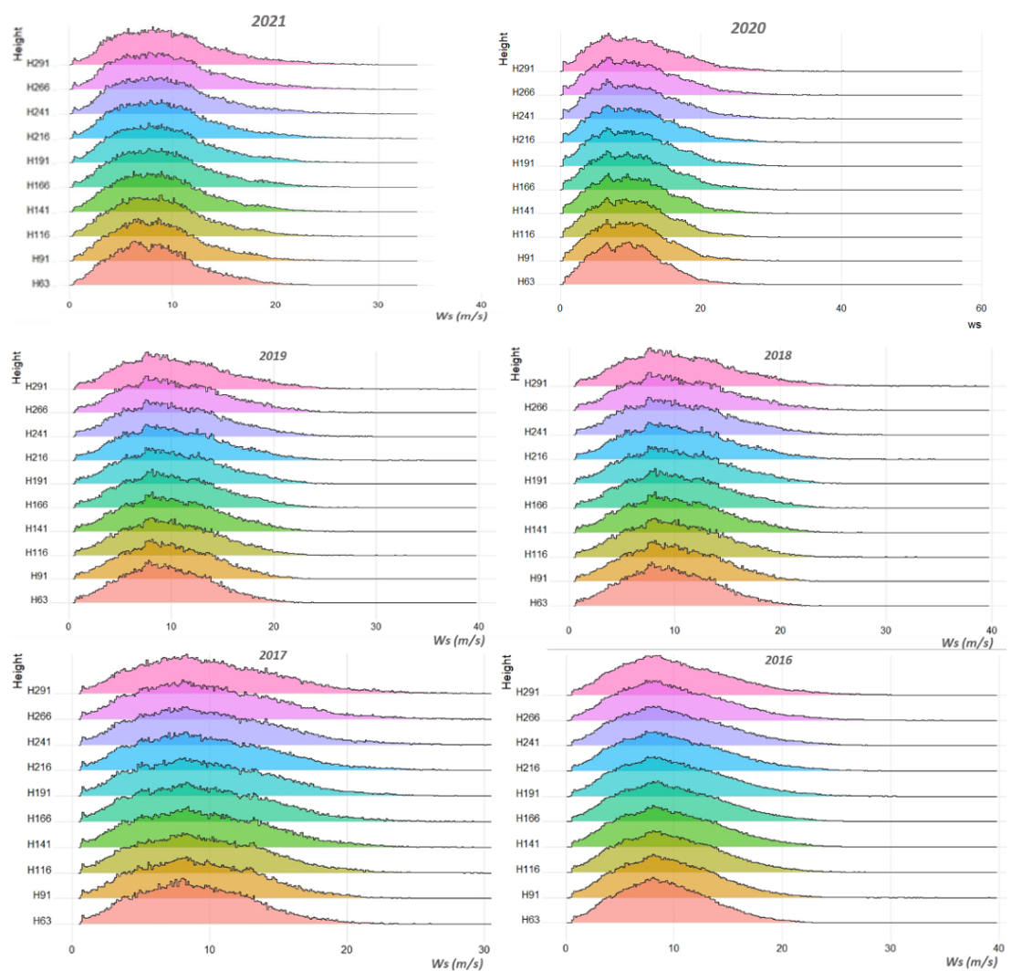
Figure 14 Annual Weibull distributions at different heights for the 2016-2021 period.
