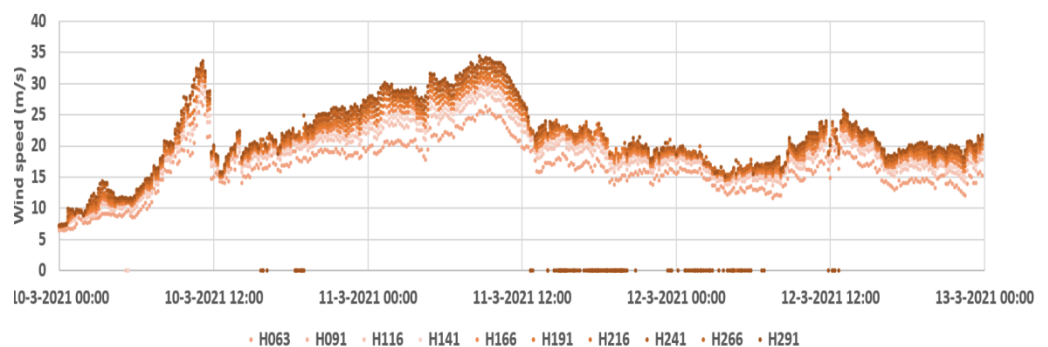
Figure 23 Focus on wind speeds measurements during Evert storm between 11 th and 13 th March
