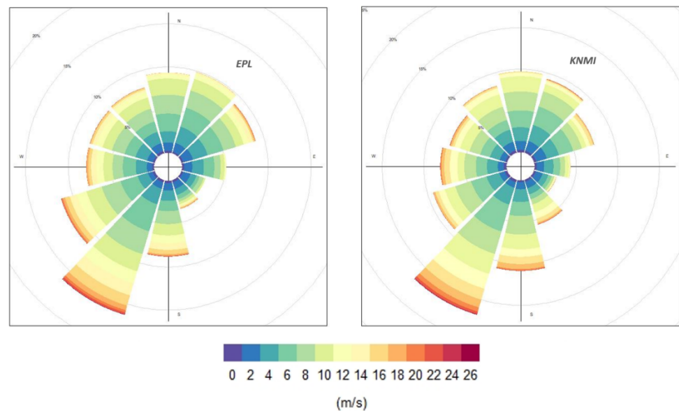
Figure 27 Wind roses for LiDAR at 63m (left) and KNMI at 38m (right) measurements at the EPL platform for the year 2021.
