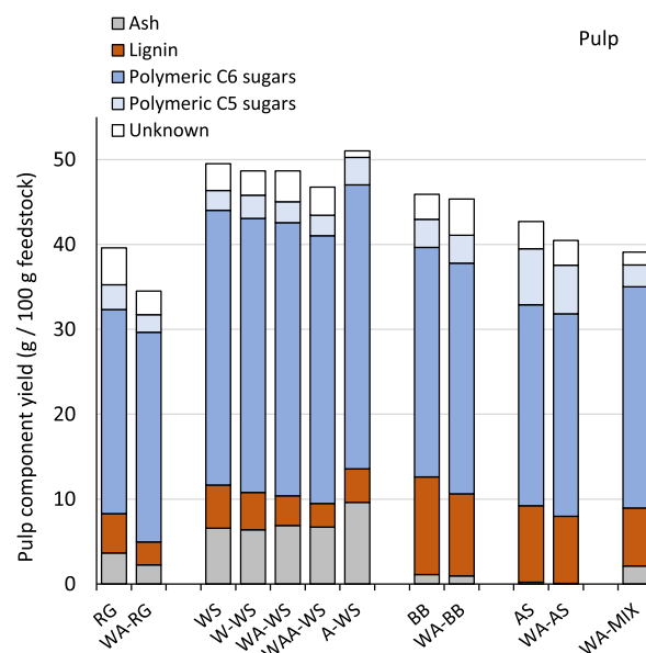
Figure 4. Yield of pulp components expressed as g of component per 100 g of the initial feedstock (dry weight basis).
