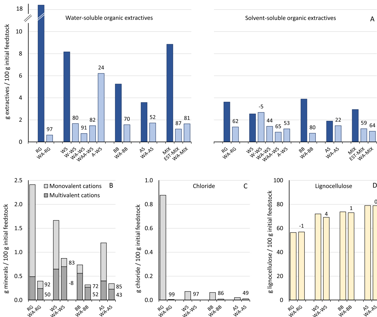
Figure 3. Organic extractives (A), minerals (B), chloride (C), and lignocellulose content (D) of untreated and pre-extracted feedstocks expressed as g/100 g initial untreated feedstock (dry weight basis). Labels represent the percent removal after pre-extraction (negative values may result from experimental error and feedstock composition heterogeneity). EST–MIX shows the values for the feedstock mixture estimated from the single feedstock extraction results. Solvent-soluble organic extractives are the sum of extractives soluble in 50% acetone, 100% acetone, and 100% pentanone. Monovalent cations include K and Na; multivalent cations include, among others, Ca, Mg, Fe, Al, Ni, Cr, Mn, and Zn. Lignocellulose content is the summative value of the contents of hexose/pentose sugars and total lignin in the extracted feedstocks corrected for mass loss after extraction (g/100 g of initial untreated feedstock).
