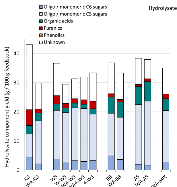
Figure 5. Yield of hydrolysate components expressed as g of component per 100 g of the initial feedstock (dry weight basis).
