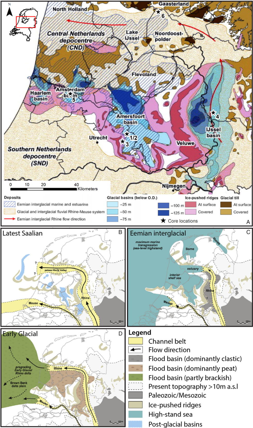
Fig. 8. (A) Map of the late Saalian ice-pushed ridges and glacial basins and Eemian fluvial and coastal deposits to illustrate the environmental setting of the investigated sites. (B–D) Palaeogeographic maps of the latest Saalian, Eemian and Weichselian Early Glacial, respectively (after Peeters et al. , 2015).
