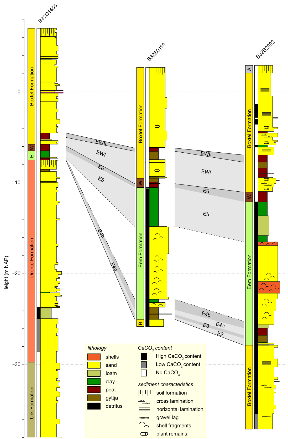
Fig. 3. Sedimentary logs and biostratigraphical correlation of the cores in the Amersfoort Basin. Horizontal axis not to scale. E is Eem Formation; W is Woudenberg Formation. For location, see Fig. 1.
