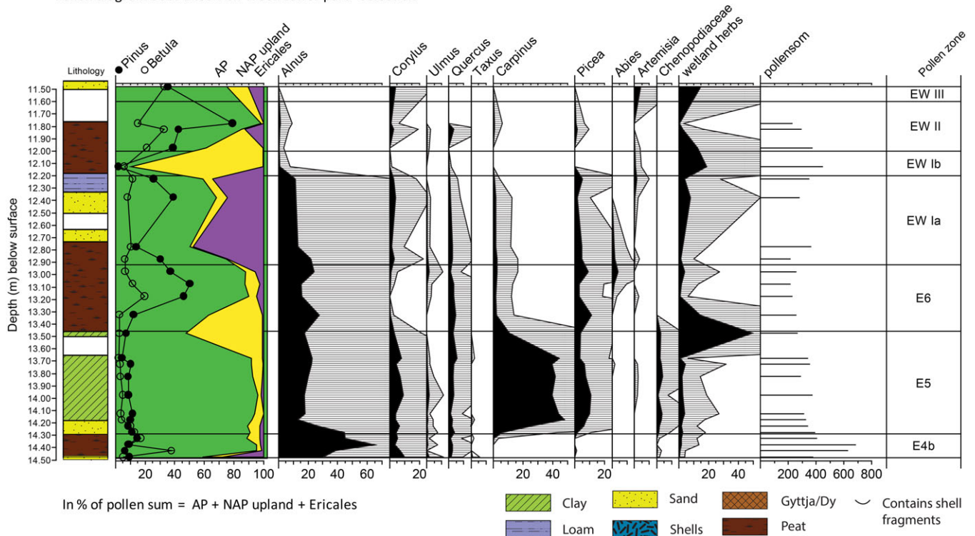
Fig. 6. Concise pollen diagram of core Den Treek (B32D1455) at the margin of the Amersfoort Basin, showing the late Eemian and transition to the Weichselian Early Glacial. Pollen sum contains the arboreal pollen, upland herbs and Ericales.
