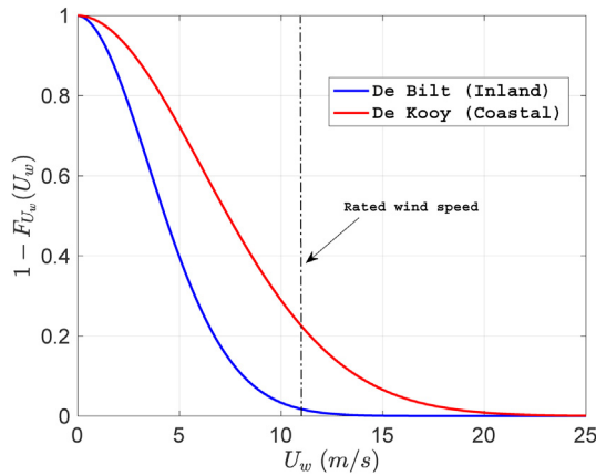
Fig. 22. Comparison of exceedance probability of wind speed for the inland De Bilt and coastal De Kooy site.
