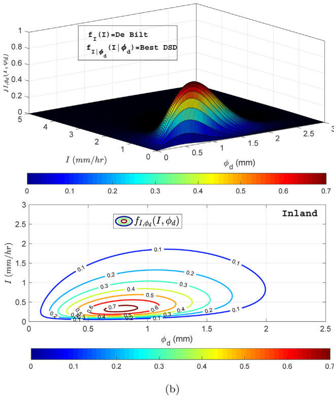
Fig. 17. Joint PDF ( f_{\phi_d|I}(\phi_d|I) ) for inland De Bilt site with (a) De Bilt's DSD (b) Best's DSD.
