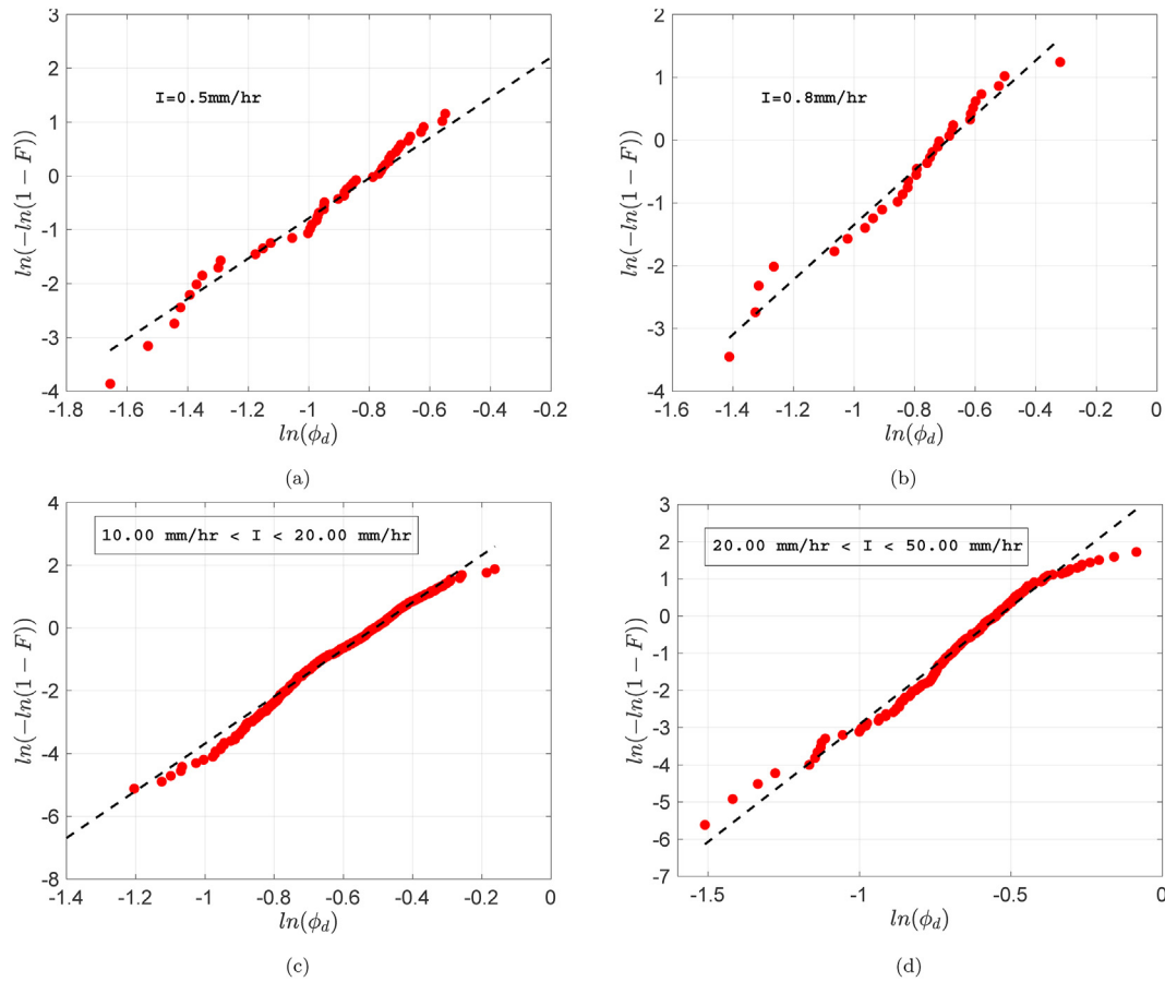
Fig. 8. Two-parameter Weibull fitting of rain droplet diameter ( \phi_d ) for different (a) I = 0.5 mm/h (b) I = 0.8 mm/h (c) 10 \text{ mm/h} < I < 20 \text{ mm/h} (d) 20 \text{ mm/h} < I < 50 \text{ mm/h}
