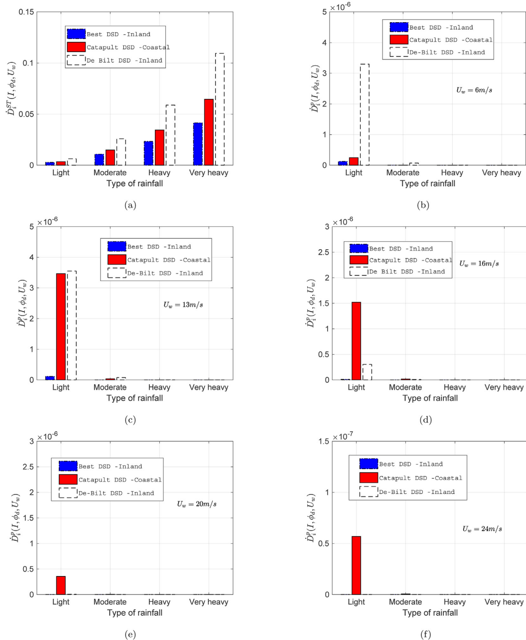
Fig. 20. (a) Comparison of short term damage erosion rate ( \dot{D}_i^{ST}(I, \phi_d, U_w) ) for different rainfall conditions, inland and coastal sites and their associated DSDs; probabilistic damage erosion rate ( \dot{D}_i^P(I, \phi_d, U_w) ) for different rainfall types (b) U_w = 6 \text{ m/s} , (c) U_w = 13 \text{ m/s} , (d) U_w = 16 \text{ m/s} , (e) U_w = 20 \text{ m/s} , (f) U_w = 24 \text{ m/s} .
