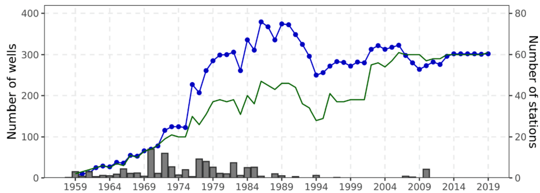
Fig. 2. Total number of active observation wells (blue line with dots, left Y axis) and number of active stations (green line, right Y axis) in corresponding year, and number of newly installed wells (columns, left Y axis) within each year. (For interpretation of the references to colour in this figure legend, the reader is referred to the web version of this article.)
