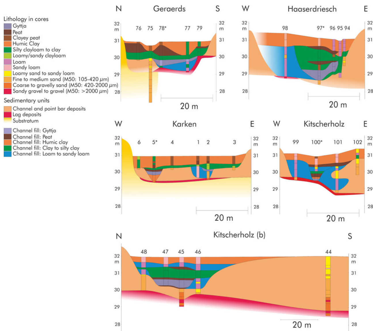
Fig. 7. Lithogenetic cross sections over abandoned channels of level B in the Dutch–German border area of the Roer valley. Asterisks indicate positions of pollen diagrams. For location see Figure 5.
