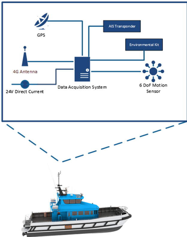
FIGURE 2 Schematic overview of the VMMS
