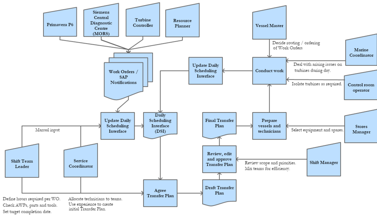
FIGURE 8 Daily maintenance planning process
