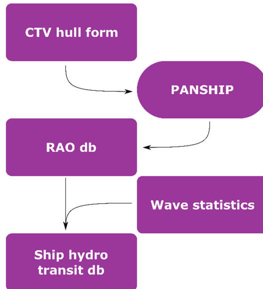
FIGURE 4 Information flow for hydrodynamic modelling
