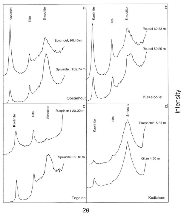
Figure 3.1.12 X-ray diffractograms of samples with clay mineralogy typical for the Oosterhout (A), Kiezeloöliet (B), Tegelen (C) and Kedichem (D) Formations. Horizontal axis: 2\theta , vertical axis: intensity. 'Kaolinite', 'Illite' and 'Smectite' at respectively 7, 10 and 14 Å.
