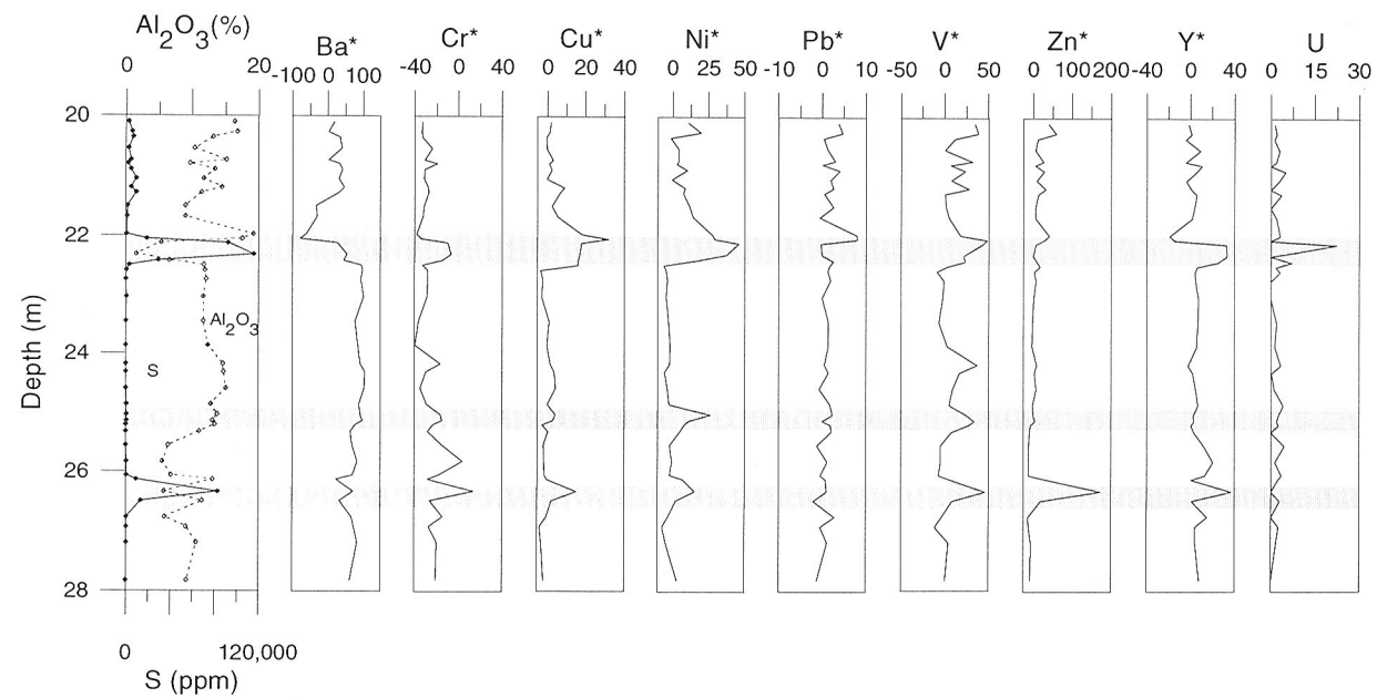
Figure 4.2.5 Depth profile of trace element concentrations corrected for Al in a part of section Heerjansdam. The shaded bands indicate organic-rich layers. Each of the organic layers shows elevated contents of several of the elements Cr, Cu, Ni, Pb, V, Zn, Y and U. Ba is depleted in the upper organic layer.
