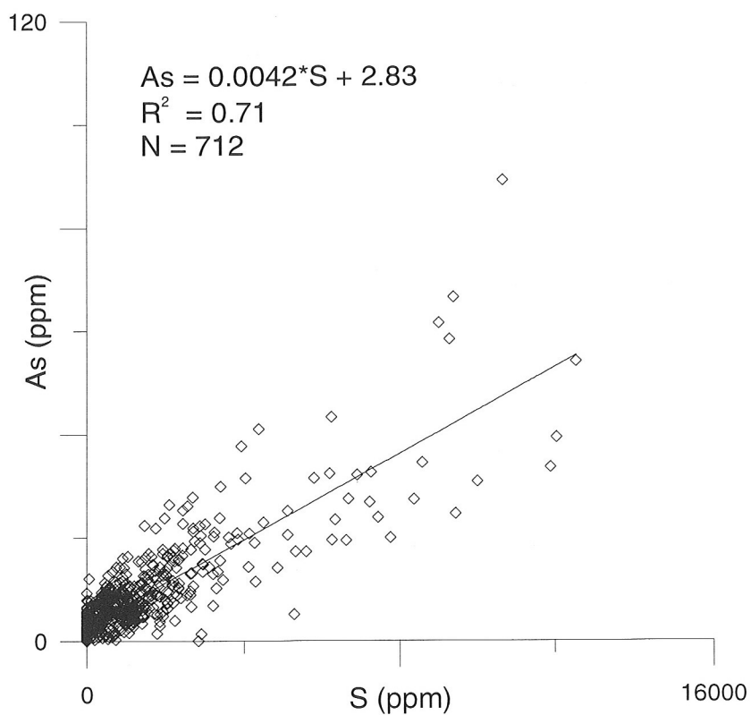
Figure 5.12 Scatterplot of As versus S with regression line. Glaucanite-bearing, peat and bog iron ore samples left out.
