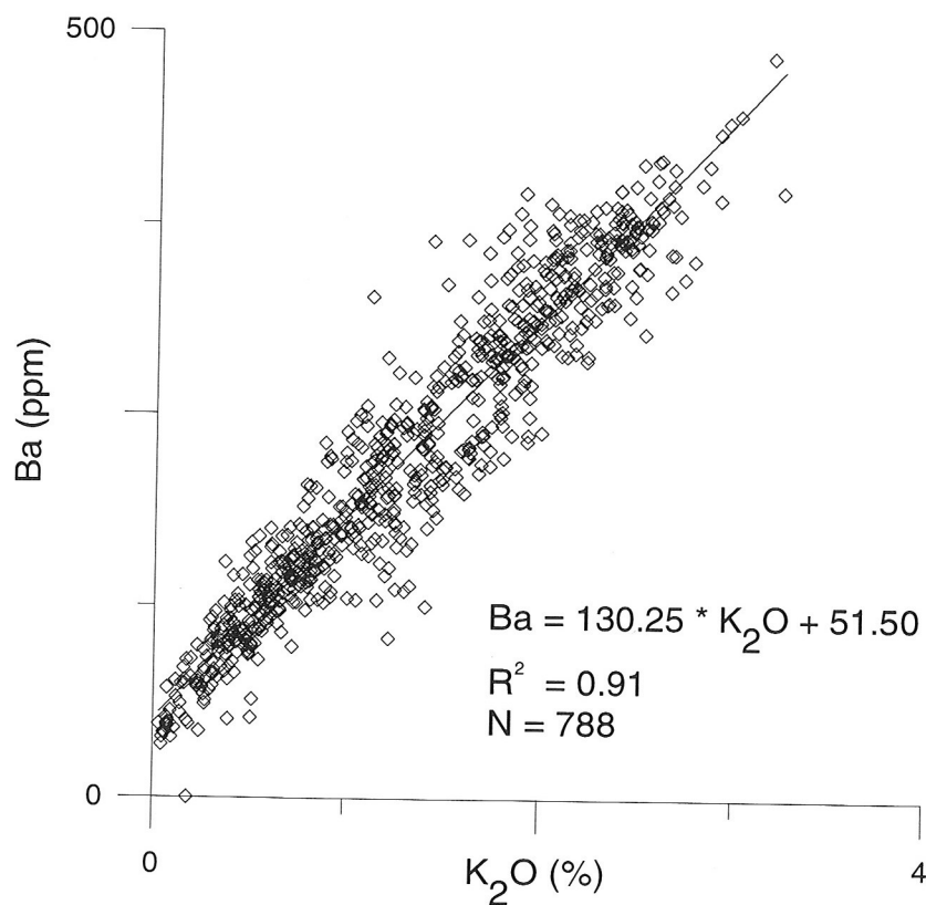
Figure 5.13 Scatterplot of Ba versus K content with regression line. Diagenetically enriched and glauconite-rich samples left out
