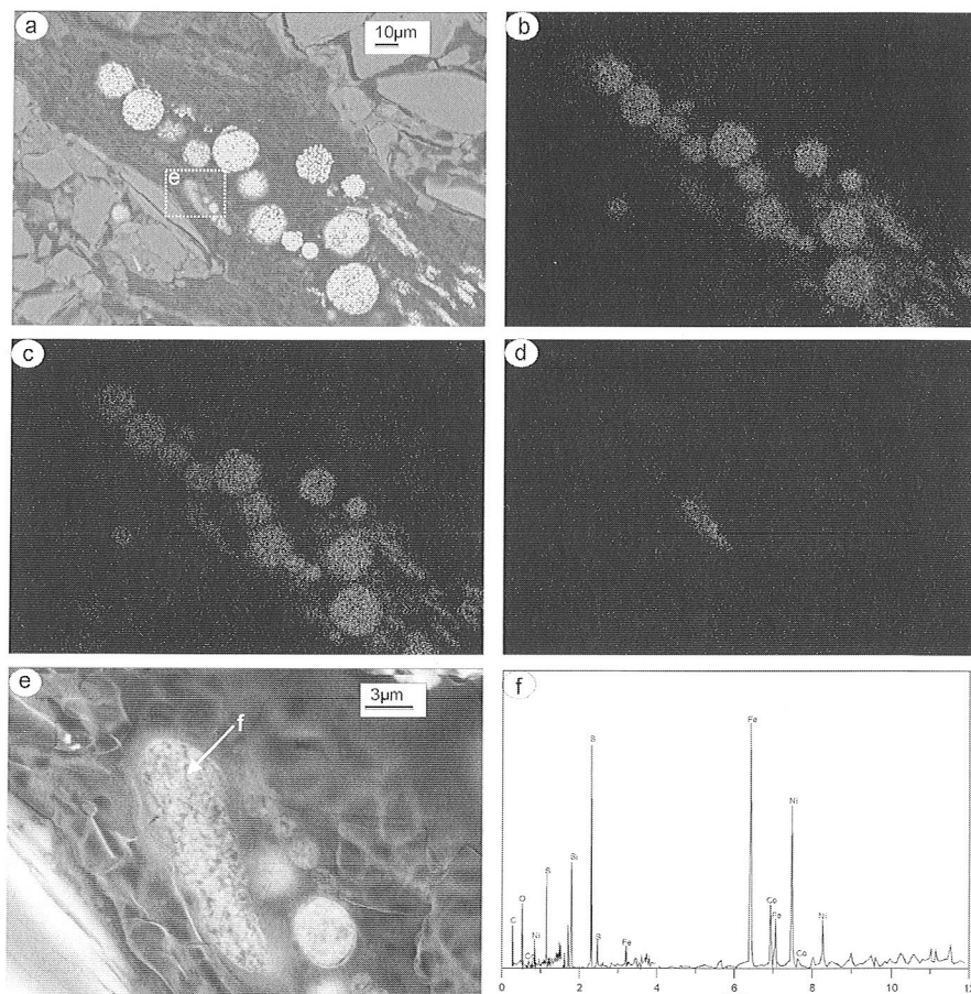
Figure 4.2.10 SEM-WDAX analyses of pyrites from Ulicoten 1. A. Pyrite framboids in organic material. Stippled square delineates the enlargements in E. B. S X-ray map of A. C. -Fe X-ray map of A. D. Ni X-ray map of A. Note that the Ni occurs only in a cluster of small framboid-like pyrites. E. Ni-rich framboids; detail of A. Note that the pyrite is less well crystallized than the Ni-poor framboids. Arrow "f" indicates WDAX-measurement presented in F. F. WDAX-measurement (composite) of framboid in E.
