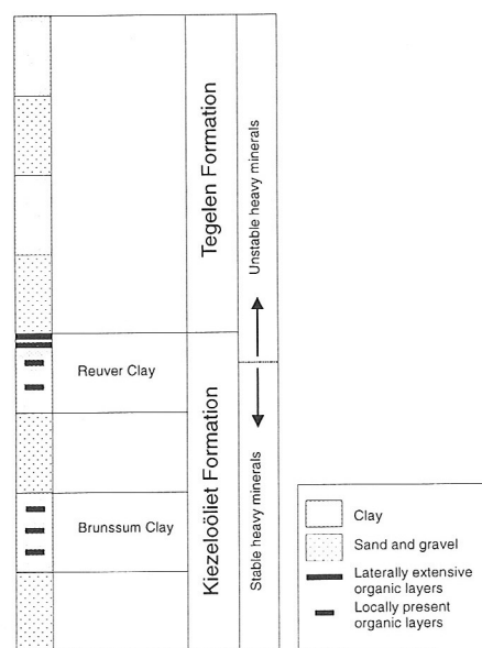
Figure 3.2.2 Schematic stratigraphic overview.
