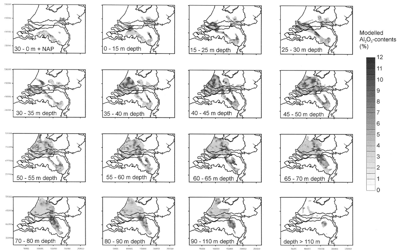
Figure 6.10 Spatial geochemical model of \text{Al}_2\text{O}_3 for the Kedichem formation.
