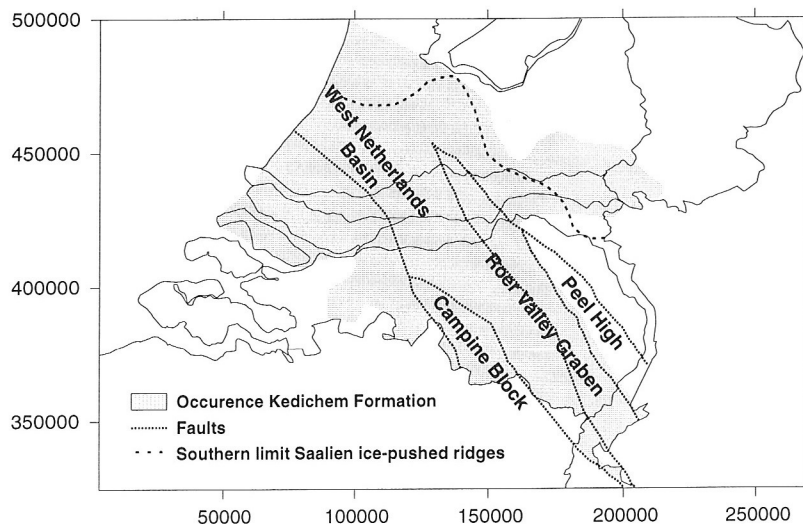
Figure 6.1 Occurrence of the Kedichem formation in the Southern Netherlands, with fault pattern used in this study (from Van den Berg, 1996 and pers. comm.) and the maximum extent of the Saalien ice sheet (Zagwijn and Van Staaldin, 1975)
