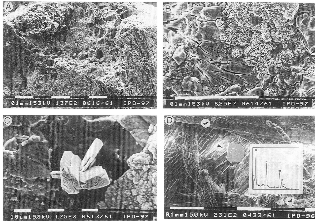
Figure 4.2.9 SEM photos of A . Pyritized cell walls of plant; Beerse. B . Pyrite from rim of rimmed plant fossil (Beerse). C . Galena crystal from the rim of a plant fossil (Beerse). D . Barite crystals (see arrow) in peat (Rijsbergen) with EDAX-scan.
