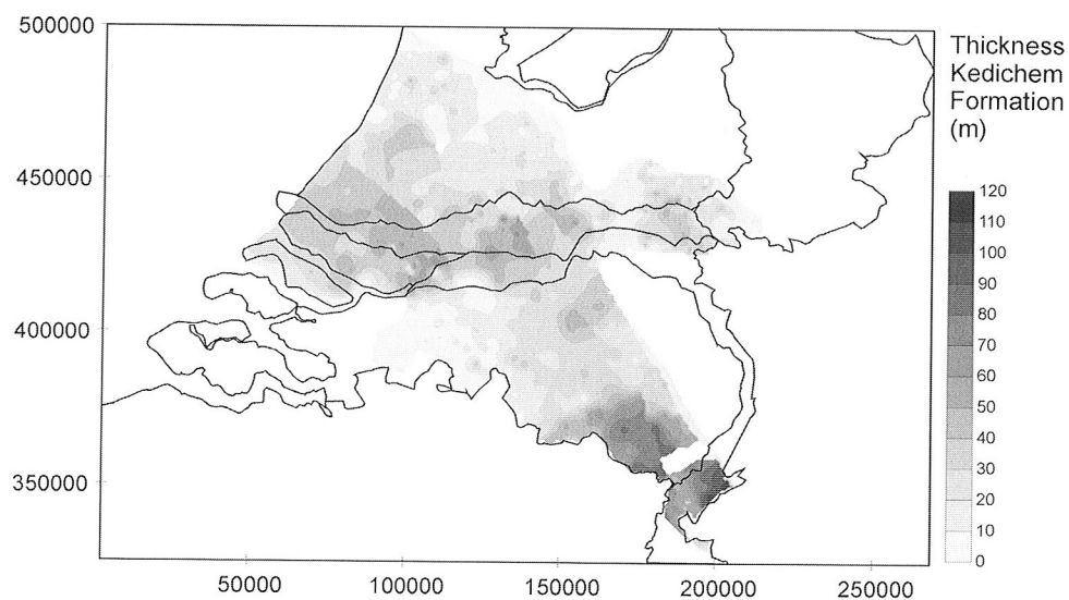
Figure 6.2 C Thickness of the Kedichem formation.
