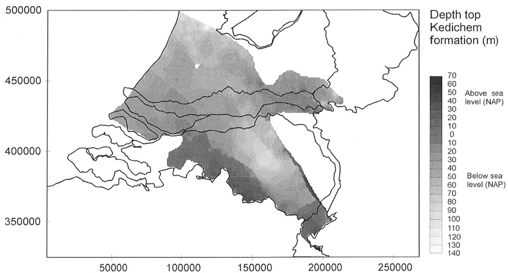
Figure 6.2 A Upper boundaries of the Kedichem formation.
