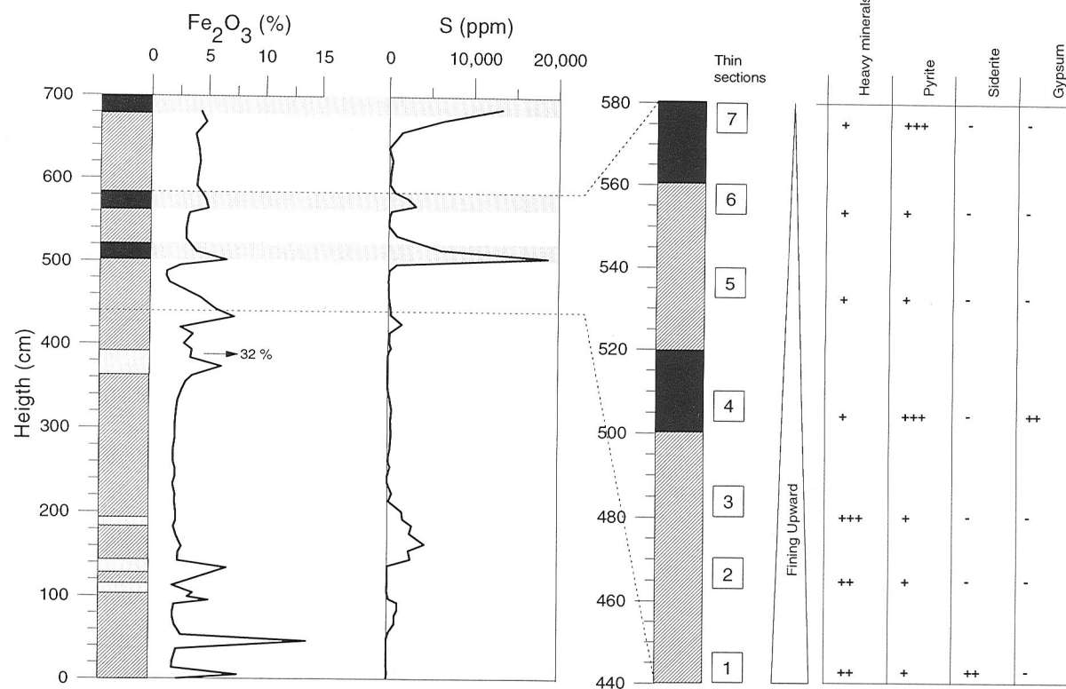
Figure 3.2.6 Depth profile of Fe- and S-contents (section BTAB). Part of the section is enlarged to indicate the and micromorphological observations. S-contents are elevated in the organic layers due to the presence of pyrite. Fe 2 O 3 -contents show a large amounts of local elevations, related to the presence of pyrite (in the organic layers) and (hydr)oxides.
