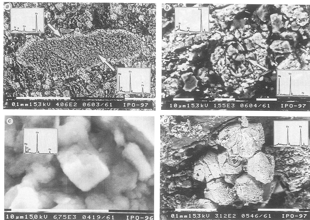
Figure 4.1.6 SEM photographs (backscatter). Results of EDAX measurements of different locations are shown in the enclosed graphs. A. 1 Dolomite grain coated with siderite (type ii). Around the grain siderite nodules (type iv) can be seen (bright dots). B. 1 Siderite nodule with a nucleus of dolomite (type ii). C. 2 In the center a euhedral grain is shown with a botryoidal shaped surface. The chemical composition points towards dolomite with a siderite coating (type ii). D. 2 A concretion of subangular concentric nodules, probably consisting of a mixture of calcite and dolomite. EDAX measurements on different locations on the nodules showed some variation of the Fe and Ca content. 1 photo from thin section. 2 photo from rough surface.
