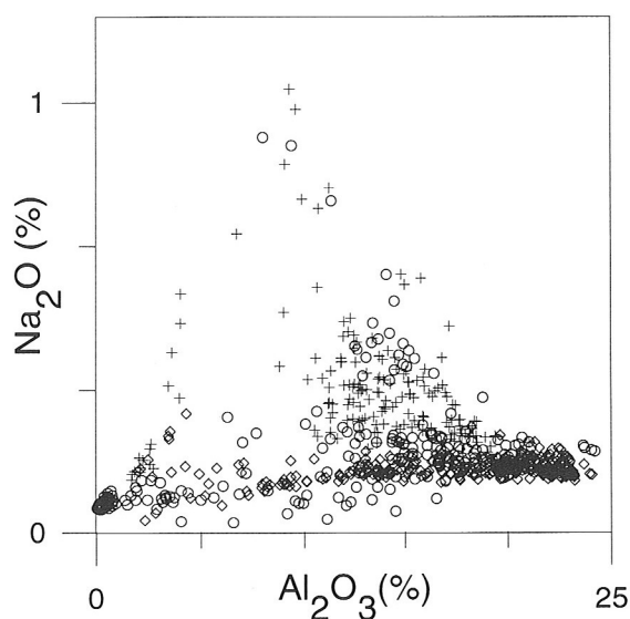
Figure 3.2.14 Scatterplot of \text{Na}_2\text{O} versus \text{Al}_2\text{O}_3 for all sections. Legend as 3.2.13. Samples from the Tegelen formation show elevated \text{Na}_2\text{O} -contents. Reuver and Brunssum samples usually have low \text{Na}_2\text{O} -contents, except for the Reuver samples from Hoher Stahl.
