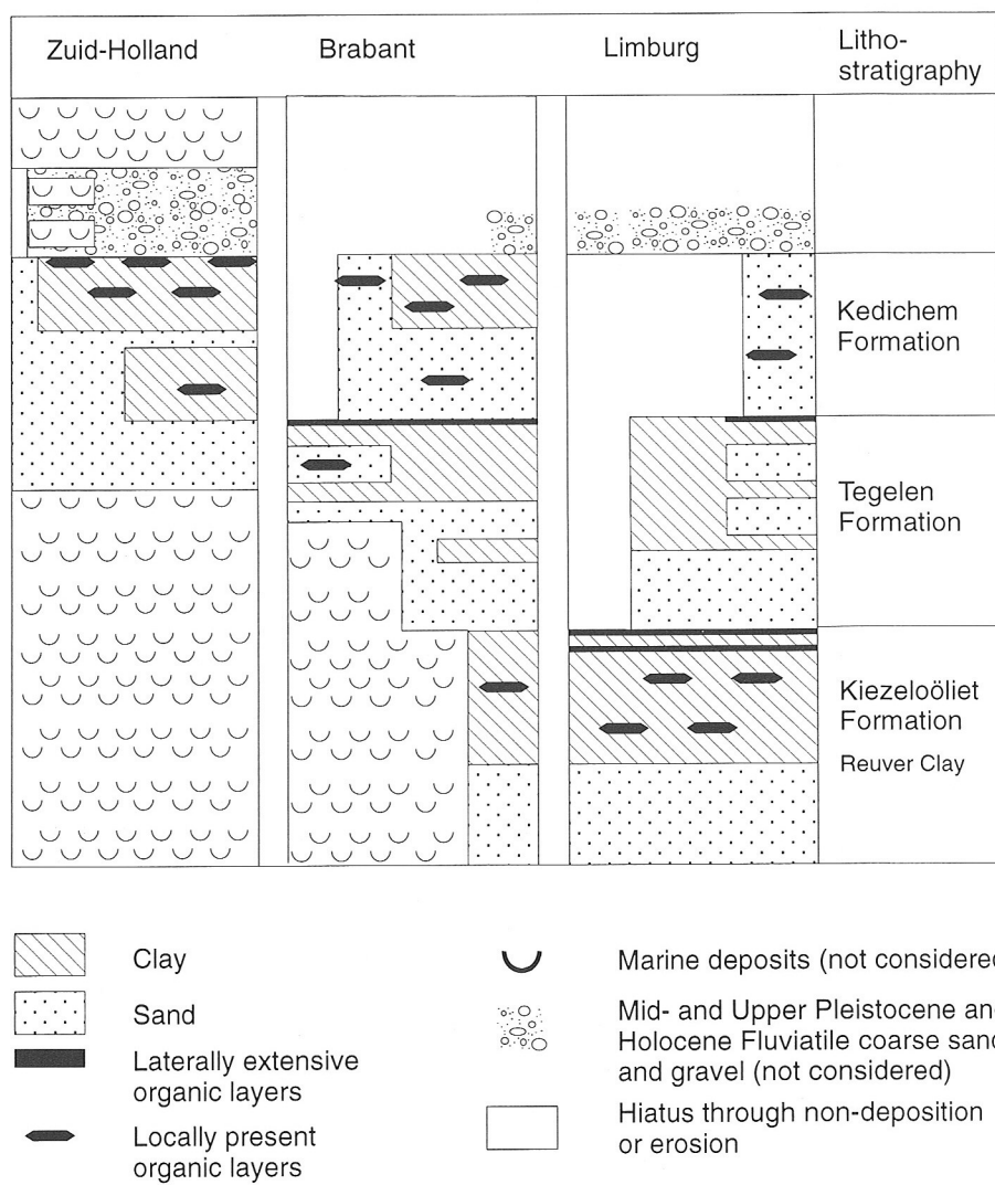
Figure 4.2.2 Schematic stratigraphy of the Pliocene and Early Pleistocene deposits in the research areas.
