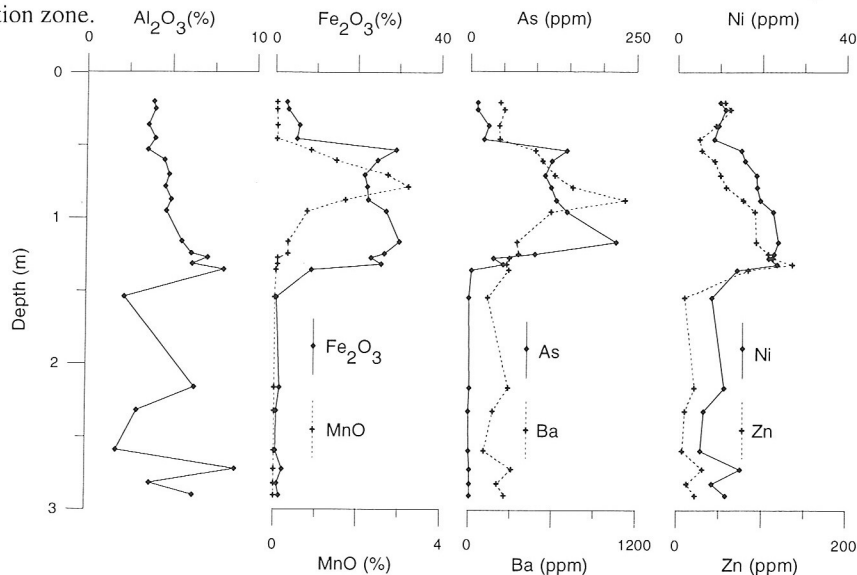
Figure 5.6 Depth profile of Al, Fe, Mn, As, Ba, Zn and Ni, boring Ulvenhout. Between 0.50 and 1.50 m, the presence of hydromorphic Fe,Mn(hydr)oxides causes elevated Fe and Mn contents. Associated with this are elevated contents of As, Ba, Ni and Zn.
