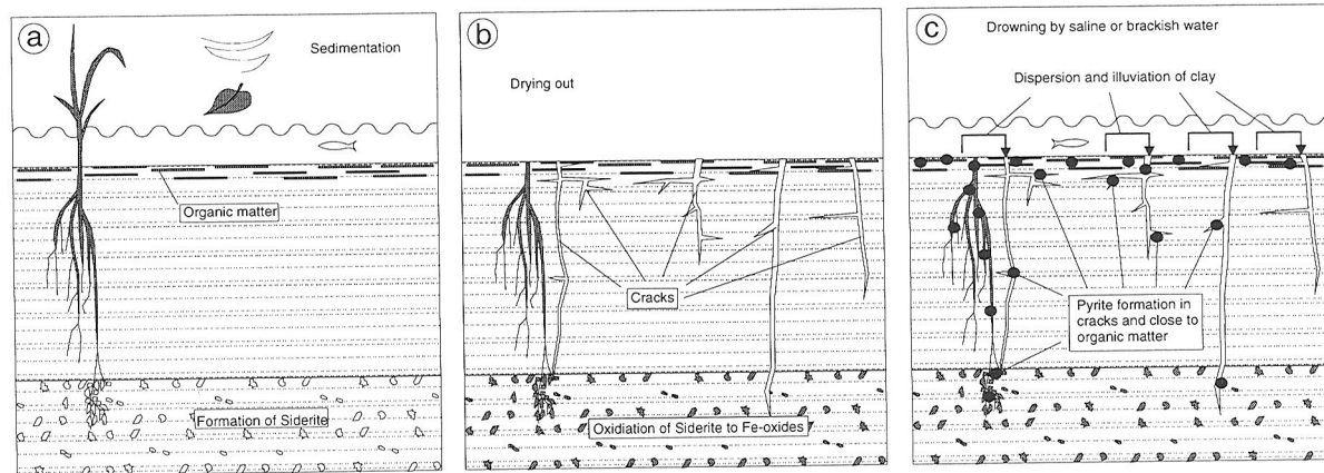
Figure 3.2.11 Reconstruction of deposition history of the organic layers in section BTAB. During the first stage (A), organic-rich sediments are deposited in a fresh-water environment, and small siderite nodules are formed. In the second stage (B), the sediments dry out, cracks form, and the siderite is oxidized to form Fe(hydr)oxides. In the third stage, one or more short-termed incursions by brackish or saline water cause dispersion and illuviation of clay, and the formation of pyrite in cracks and close to organic matter.
