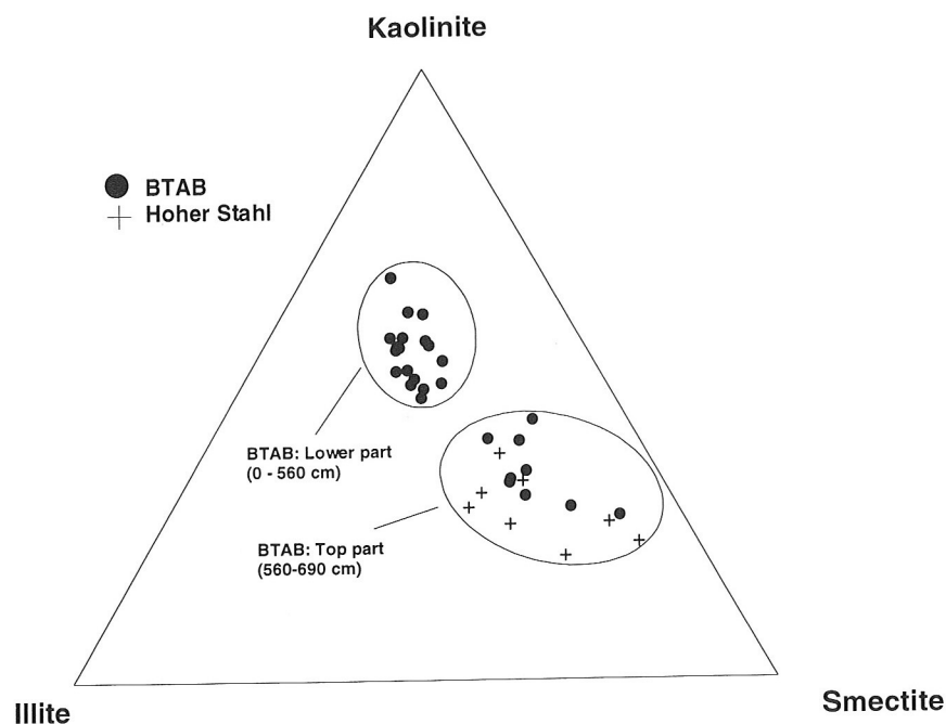
Figure 3.2.9 Triangular graph of the clay mineralogical composition of sections BTAB and Hoher Stahl. Clay mineral percentages based on relative peak height. The clay from the top of the BTAB section can be discerned clearly from the lower part of the section. The clay from Hoher Stahl has a similar mineralogy as the upper part of the BTAB section.
