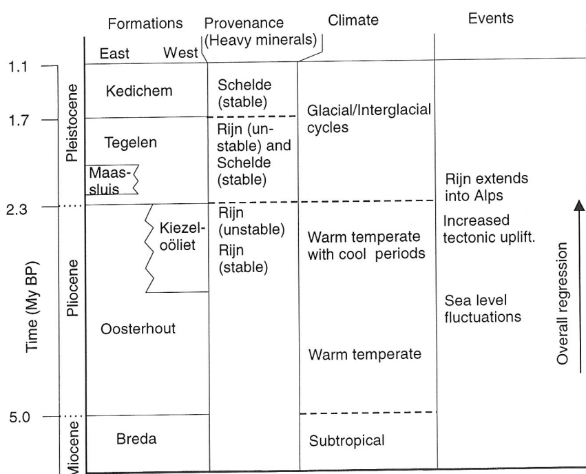
Figure 3.1.3 Summary of stratigraphy, heavy-mineral provenance and geological history of Late Cenozoic sediments in the Southern Netherlands.
