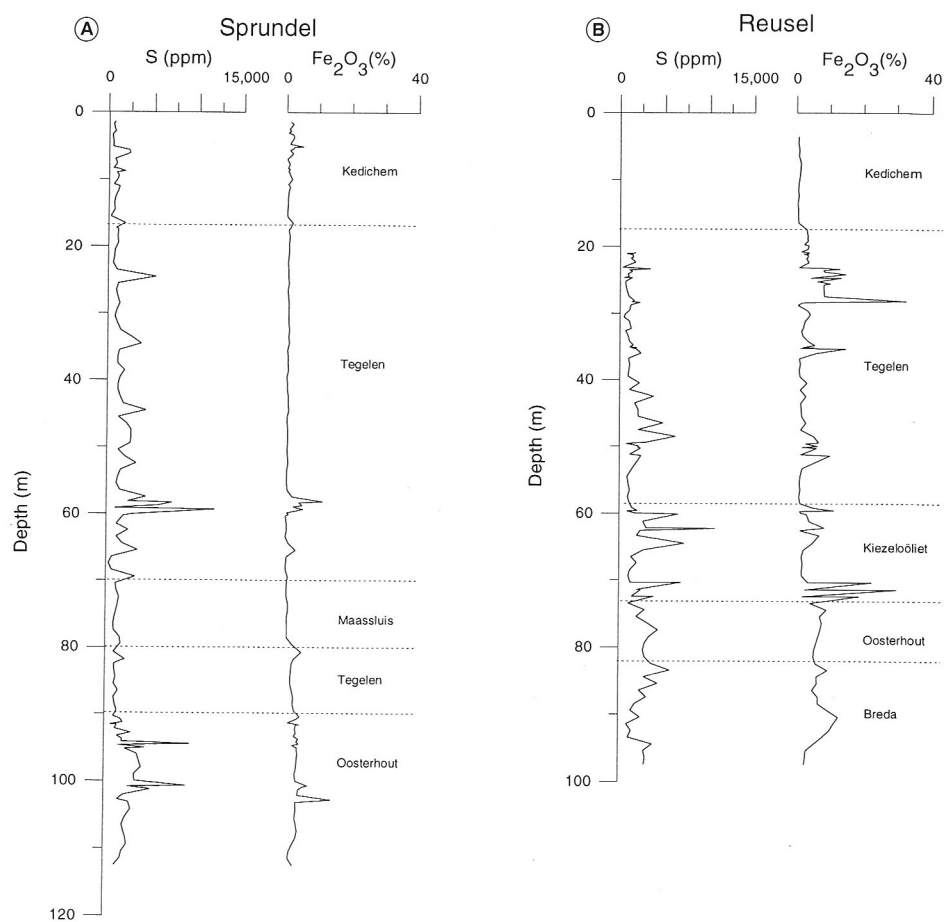
Figure 3.1.11 Depth profiles of S and \text{Fe}_2\text{O}_3 in borings Sprundel (A), Reusel (B) and Rucphen 2 (C; previous page). S-contents are indicative for the presence of pyrite, whereas the \text{Fe}_2\text{O}_3 -contents are related to pyrite or siderite. The elevated Fe-contents in boring Reusel between 70 and 73 m depth, however, are related to the presence of Fe(hydr)oxides. Note enlarged depth scale of Rucphen 2. Formation names are indicated.
