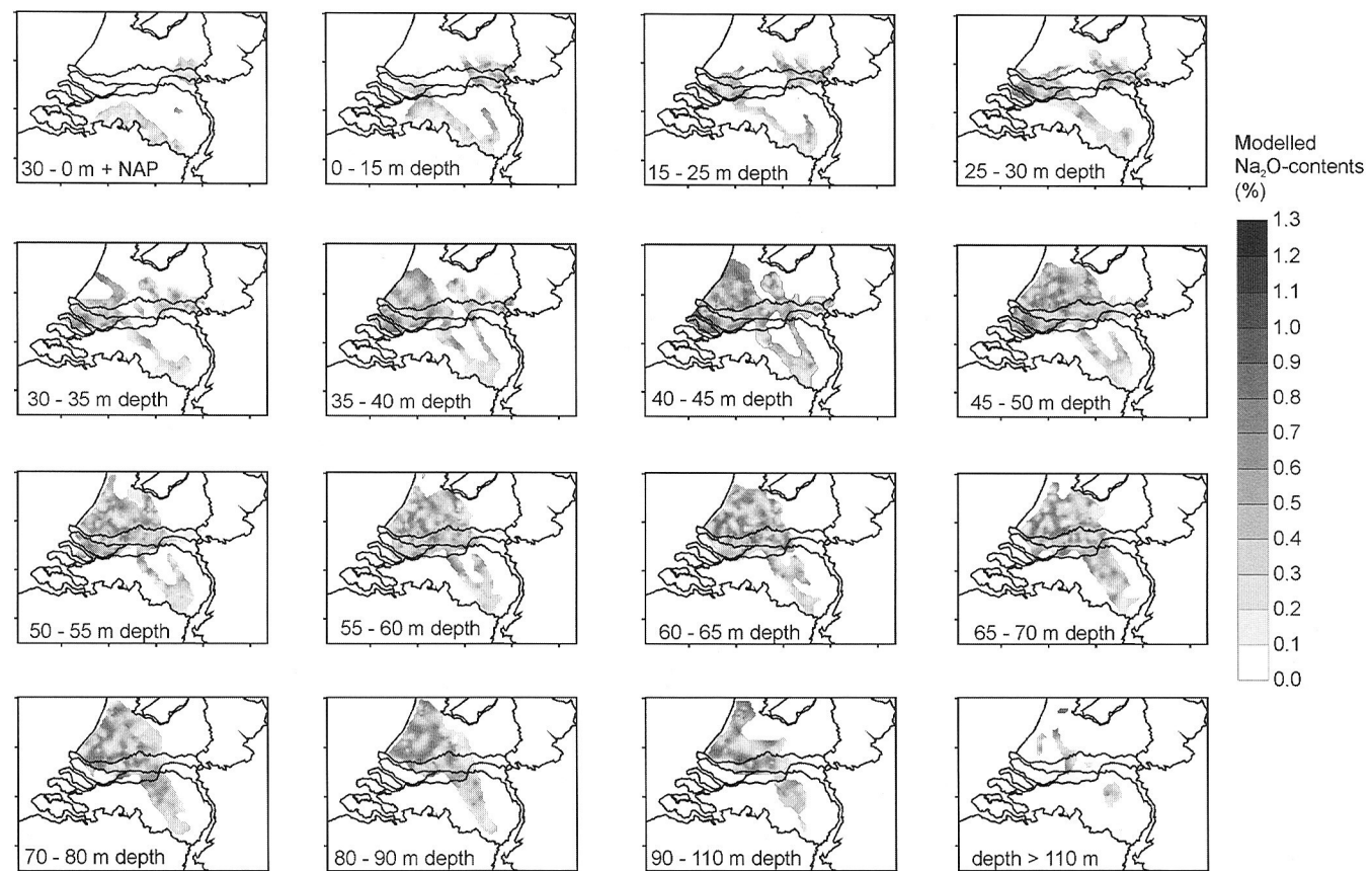
Figure 6.12 Spatial geochemical model of \text{Na}_2\text{O} for the Kedichem formation.
