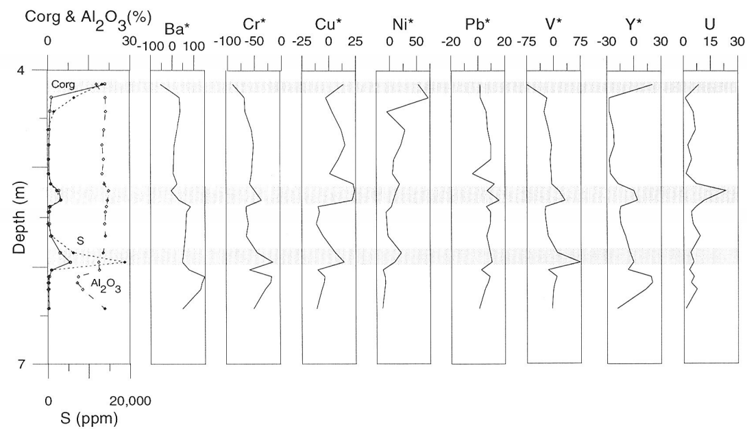
Figure 4.2.4 Depth profile of trace element concentrations corrected for Al in a part of section BTAB. The shaded bands indicate organic-rich layers. Each of the organic layers shows elevated contents of several of the elements Cr, Cu, Ni, V, Y and U. Note that the Ni-enrichments associated with the upper two organic layers is just at the edge, of the layers. Ba, Cr and V are depleted in the upper organic-rich layer.
