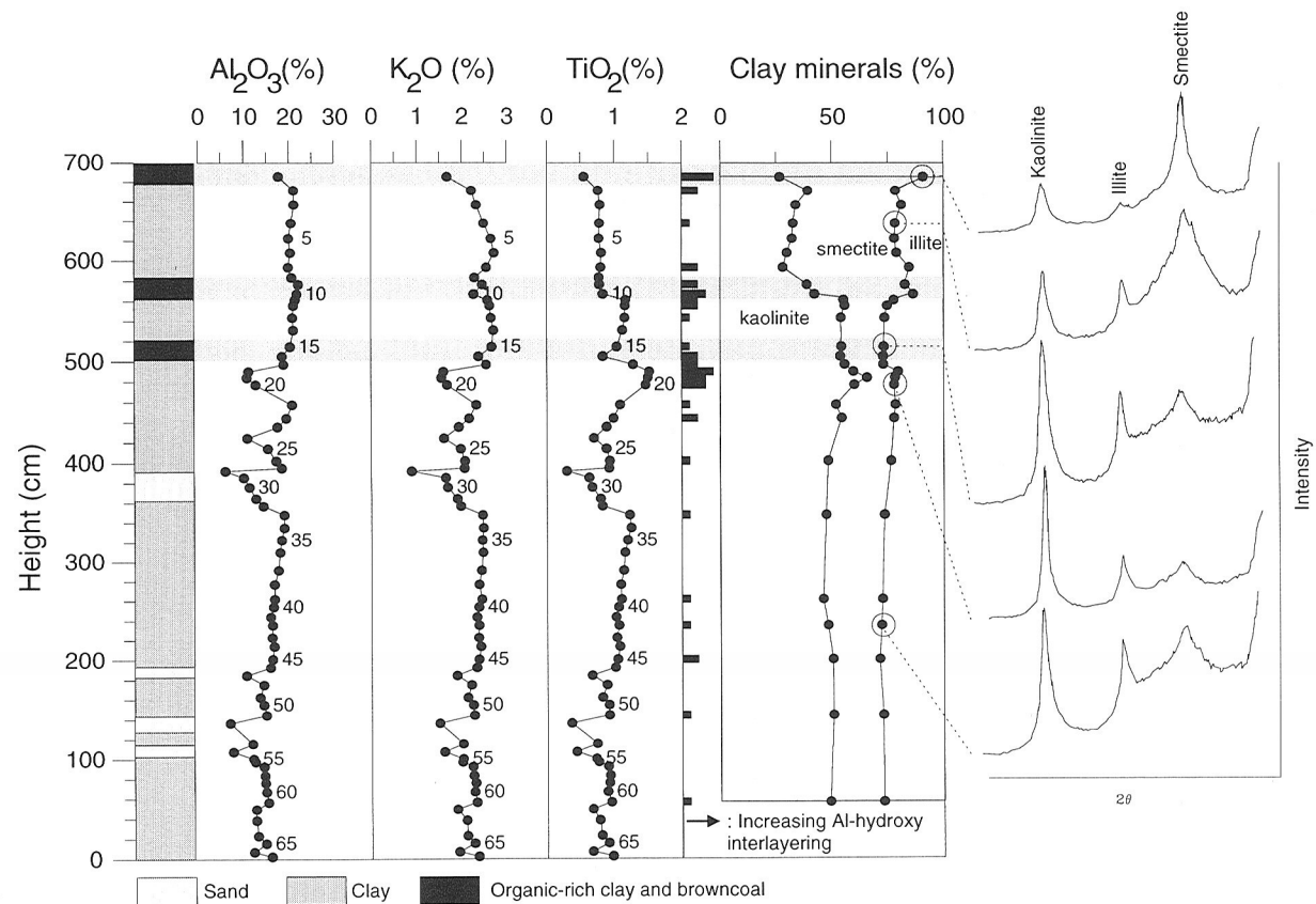
Figure 3.2.4 Depth profiles of \text{Al}_2\text{O}_3 , \text{K}_2\text{O} and \text{TiO}_2 -contents and clay mineralogical properties of section BTAB. Figures indicate sample numbers (referred to in text). Degree of Al-hydroxy interlayering is a qualitative scale. Clay mineral percentages are based on relative peak heights. The diffractograms of five representative samples are given, with “kaolinite”, “illite” and “smectite” at 7, 10 and 14\text{\AA} respectively. The clay above the middle organic-rich layer is smectite-rich, whereas the clay below it shows higher contents of kaolinite and \text{TiO}_2 . \text{TiO}_2 and kaolinite contents are further elevated immediately below the lower organic-rich layer. \text{K}_2\text{O} -contents drop in all three organic-rich layers, and there is an increase in Al-hydroxy interlayering.
