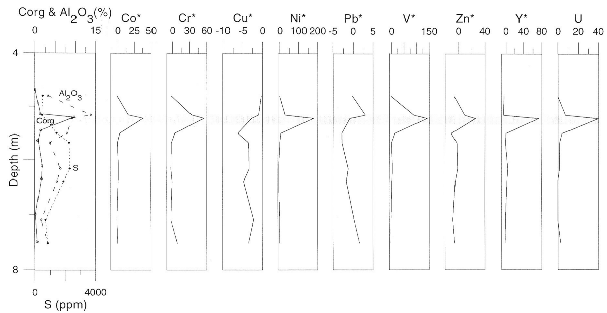
Figure 4.2.3 Depth profile of trace element concentrations, corrected for Al, in a part of section Sprundel. The shaded band indicates an organic-rich clay layer. In this layer, the contents of Co, Cr, Ni, V, Zn, Y and U are elevated.
