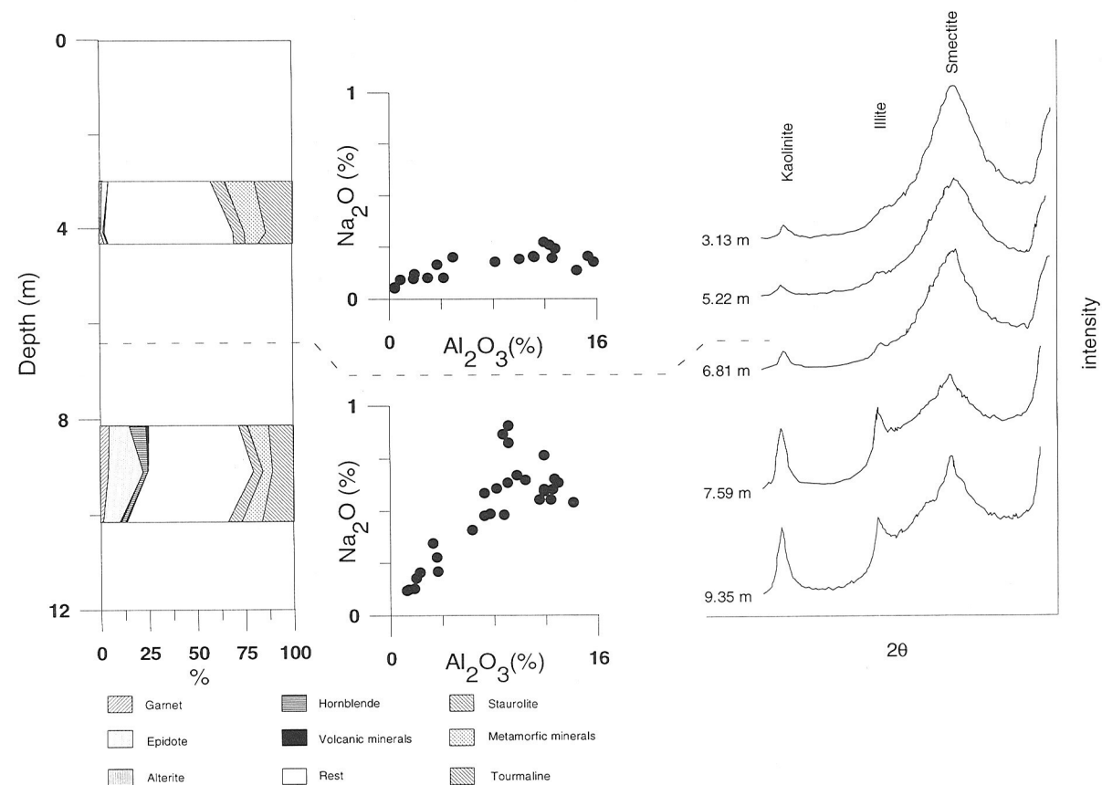
Figure 3.1.13 Heavy mineralogy, Na/Al relation and clay mineralogy of the Kedichem Formation in boring Rucphen 2. See 'Introduction' for heavy-mineral names. Dashed line indicates boundary between high and low \text{Na}_2\text{O} contents. High \text{Na}_2\text{O} contents correlate with a mixed heavy mineral composition, whereas low \text{Na}_2\text{O} -contents correlate with a stable heavy-mineral suite. Somewhat below the boundary between high and low \text{Na}_2\text{O} -contents, the clay mineralogy shifts from smectite-dominated to kaolinite-illite-dominated.
