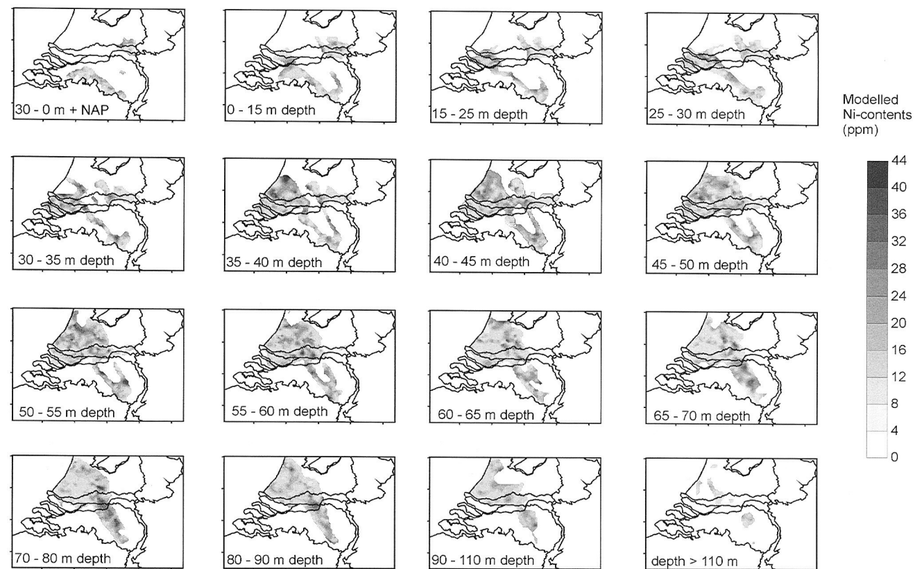
Figure 6.11 Spatial geochemical model of Ni for the Kedichem formation.
