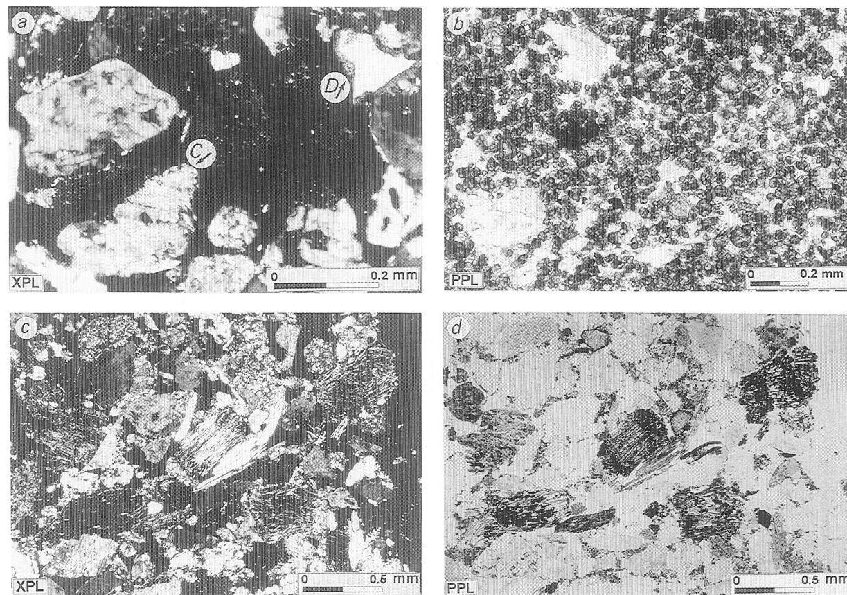
Figure 4.1.5 Thin section photographs taken under a petrographic microscope. A. Within the lower left corner (C) a calcite grain is shown (type i). The denticulated border and the holes within the grain indicate dissolution of the mineral. In the upper right corner a dolomite grain (D) coated with siderite can be seen (type ii). B. Equidimensional siderite grains (type iv). C. Siderite grains between the platelets of micas. The mica platelets show high interference colors, while the siderite is visible as dark dots. Left of the middle mica a siderite dolomite grain can be seen. D. PPL of C., showing the abundant amount of siderite nodules within the micas.
