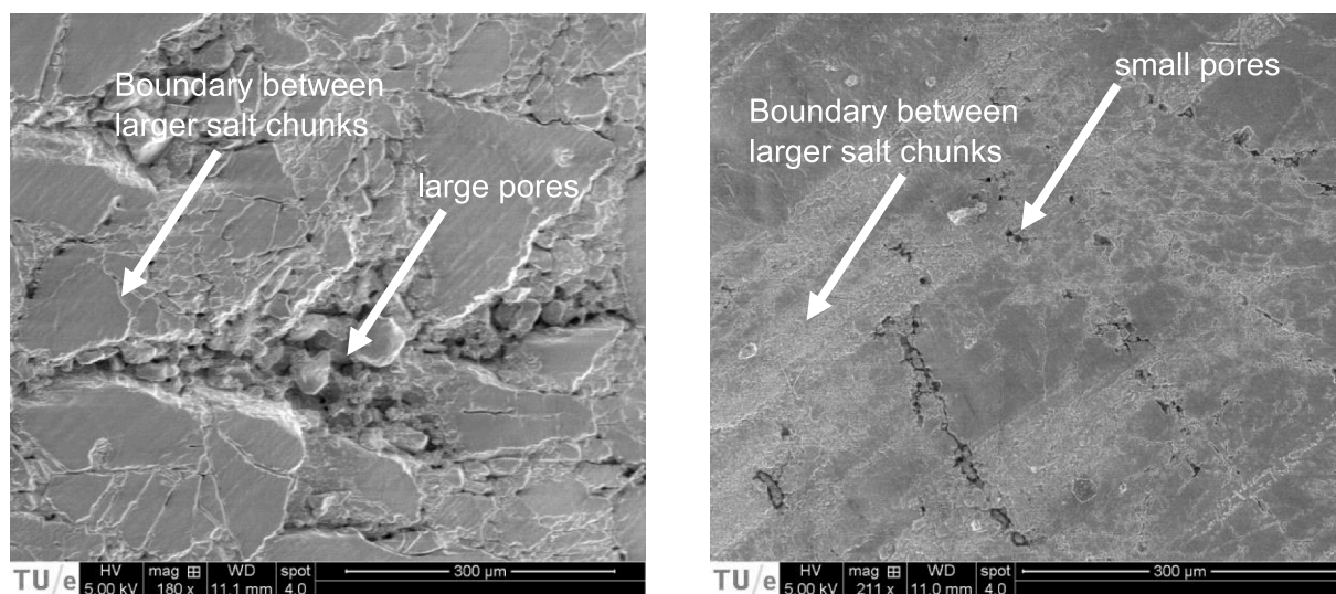
Fig. 6. SEM image of the cross-section of a hydrated particle made from 300-500 \mu\text{m} powder, pressed at low pressure with lower relative density (83%, left) and high pressure with higher relative density (96%, right).
