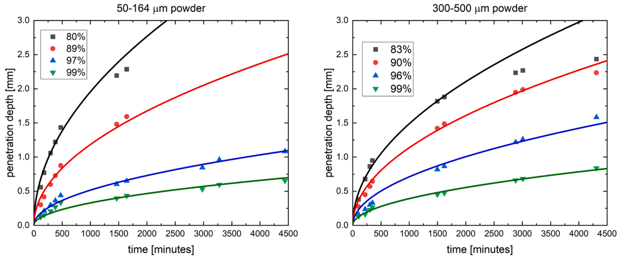
Fig. 13. Penetration depth versus time plots for particles made from 50-164 \mu\text{m} (left) and 300-500 \mu\text{m} (right) powder with different relative densities of the hydrated particles. Fitting was done using Eq. (22). Particles were hydrated at 33% relative humidity and 20°C. Only data points below 100% conversion are shown since the exact time of reaching 100% conversion could not be determined. The solid lines correspond to the fitted curves.
