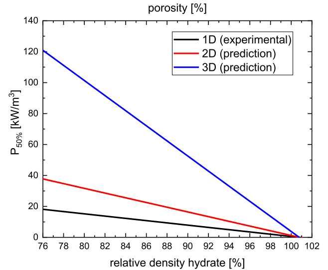
Fig. 18. Linear fit of the experimentally calculated power output from Fig. 16 for a 1D system (black line) and predicted values for equal particles as if they would be 2D (red line) or 3D (blue line).
