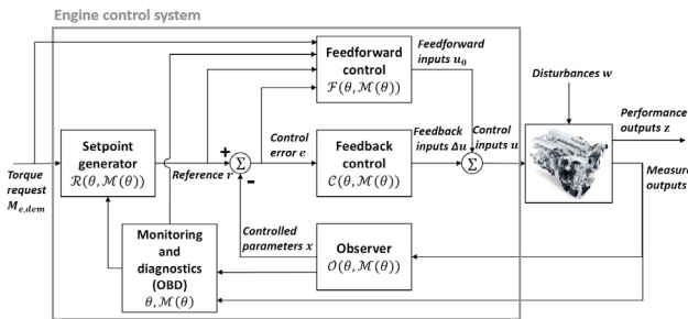
Fig. 2. General engine control system architecture.
