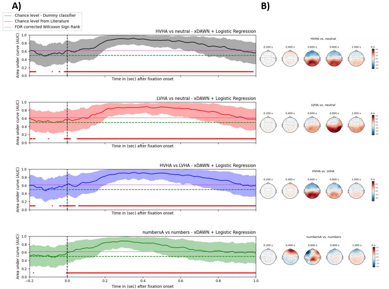
Figure 1. Temporal decoding of a logistic regression to discriminate emotional states and workload levels. A) Grand-average classification performance of the Monte Carlo Simulation (MCS; 100 iterations) measured with the metric Area Under Curve (AUC) and averaged across subjects, folds, and iterations. Shaded areas represent the 5 and 95 percentiles. Dotted purple line: Theoretical chance level at 0.62 [24]. Dashed green line: Dummy classifier with stratified as method. Red dots: Significant time points examined via a Wilcoxon Sign Rank test (one-sided) with False Discovery Rate (FDR) correction for multiple comparisons and a significance level at \alpha = .01 comparing the average classification performance of the MCS tested against the empirical chance level. B) Topographical plots represent the spatial patterns of the coefficients from the decoding models.
