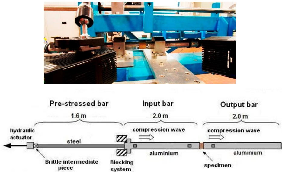
Fig. 3. Split Hopkinson Bar Test Setup
