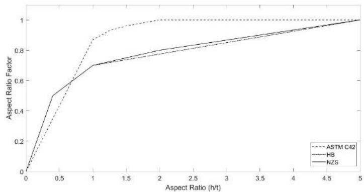
Fig. 4. Aspect ratio correction factors according to different standard (HB, NZS, ASTM)
