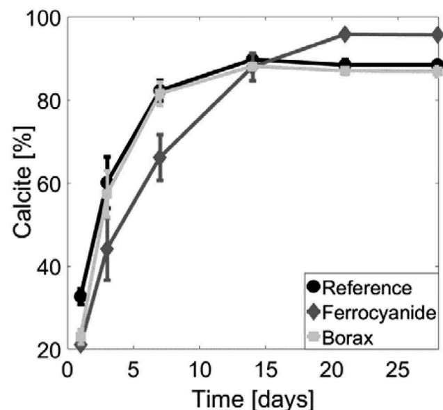
Figure 1. Carbonation rate determined by PXRD.
