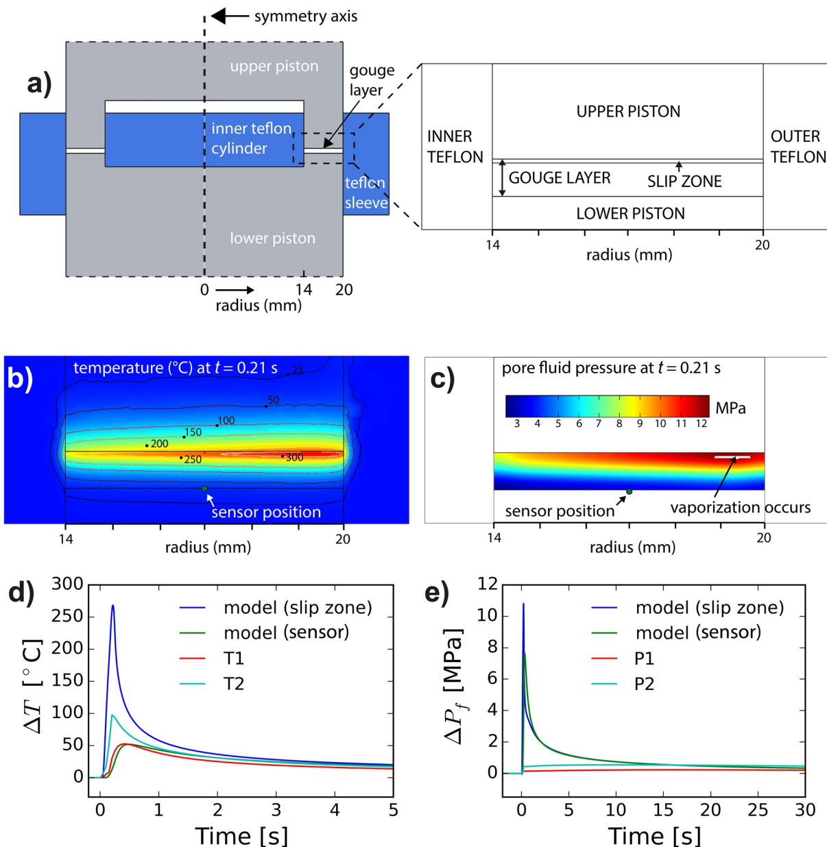
Figure 5. Thermal pressurization model results for Basal Zechstein run LHV1442 (ring setup, 20 MPa normal stress), using \Lambda = 0.06 MPa/ ^{\circ}\text{C} and \alpha_h = 0.1 mm 2 /s (see Supporting Information S5). (a) Schematic representation of the FEM configuration (shown in more detail in Figure S7). Slip is assumed to localize in a 100 \mu\text{m} thick zone at the top of the 0.8 mm gouge layer. (b) and (c) Temperature and pore fluid pressure distribution at t = 0.21 s after initiation of slip. Vaporization is expected to occur within \sim 5\% of the slip zone, as indicated. (d and e) Comparison between the modeled temperature/pore fluid pressure and the measurements (at sensors T1, T2, P1, P2—refer Figure 4a), showing the volume-averaged results for the localized zone as well as for the point corresponding to the sensor positions (green dot in Figures 5b and 5c).
