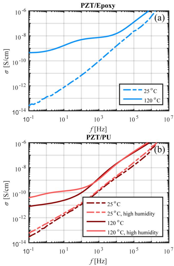
Figure 11. Composite conductivity, \sigma , as a function of frequency, f , for (a) PZT/Epoxy and (b) PZT/PU composites, with a volume fraction of 50%. Measurements are both performed at room temperature and the poling temperature of 120 °C.
