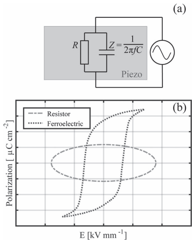
Figure 9. (a) Equivalent circuit diagram of a piezoelectric material exposed to an AC electric field is applied. (b) Typical hysteresis loops of a resistor and a ferroelectric [31].
