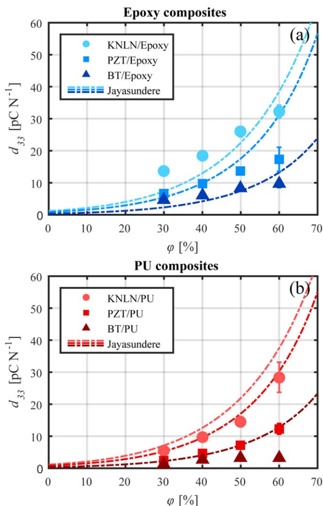
Figure 4. Composite piezoelectric charge constant, d_{33} , versus filler volume fraction, \phi , of (a) epoxy composites and (b) PU composites. The three different filler materials, KNLN, PZT and BT, are given in different shades of blue and red, with different symbols. The dashed lines are obtained from Jayasundere's model.
