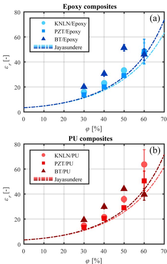
Figure 2. Composite relative dielectric constant, \epsilon_r , versus filler volume fraction, \phi , of (a) epoxy composites and (b) PU composites. The three different filler materials, KNLN, PZT and BT, are given in different shades of blue and red, with different symbols. The dashed lines are obtained from Jayasundere's model. Note that only two dashed lines are visible since two of them, the PZT and BT line, closely overlap each other. This happens due to their similar value of \epsilon_f .
