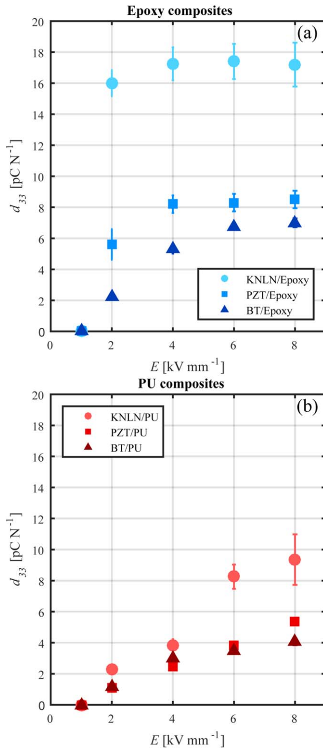
Figure 5. Composite piezoelectric charge constant, d_{33} , versus DC electric poling field, E , of (a) epoxy composites and (b) PU composites. All composites are poled for 5 min at 120 °C. Due to its low T_c , only the BT composites are cooled down to below 50 °C before the poling field is removed. The three different filler materials, KNLN, PZT and BT, are given in different shades of blue and red, with different symbols.
