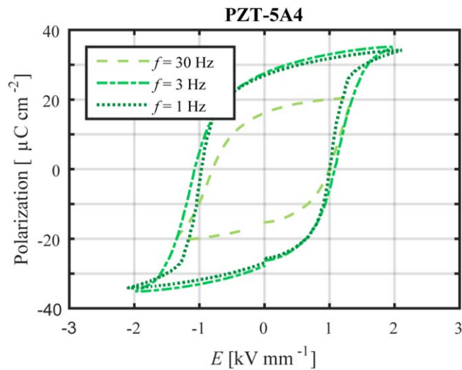
Figure 8. Hysteresis loop of PZT-5A4 ceramics, varying the applied AC electric field frequency.
