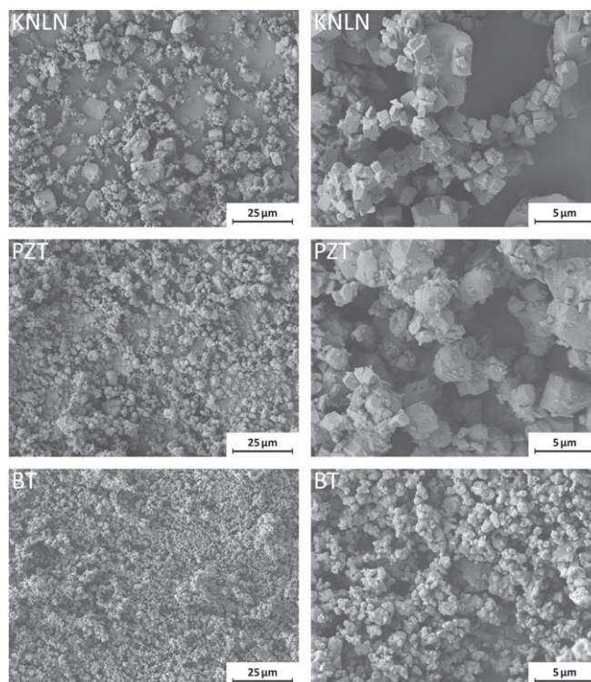
Figure 1. SEM micrographs of calcined KNLN particles, PZT particles and BT particles, at a 1000 \times (left) and 5000 \times (right) magnification.
