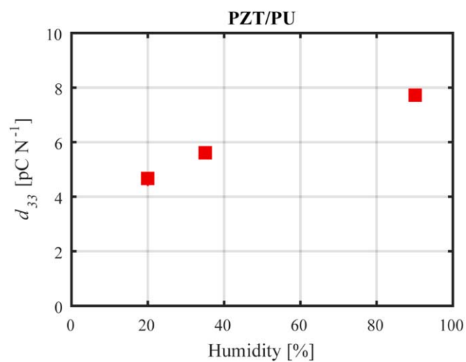
Figure 12. Piezoelectric charge constant, d_{33} , of 40 volume percent PZT/PU composites as a function of the humidity in which the composites are aged at for a week.
