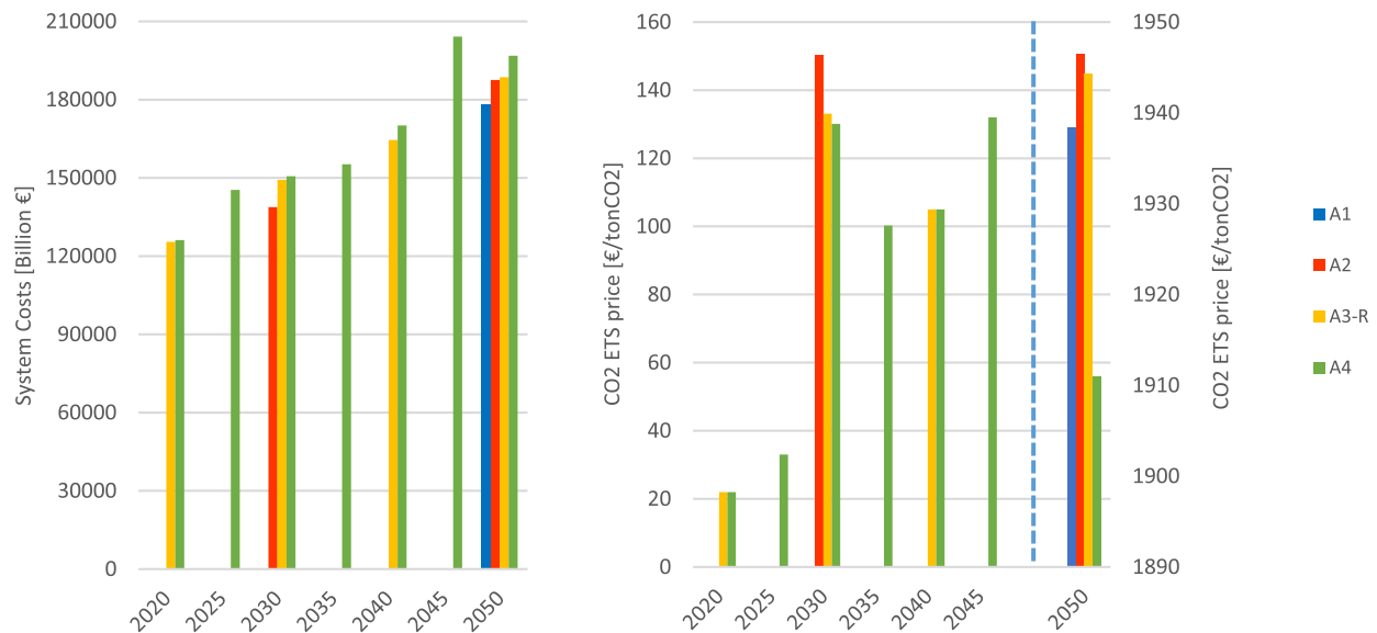
Fig. 10. Left: comparison of the system costs at the different years of the transition for the 4 cases used to explore the transitional scope considerations of the model. Right: comparison of CO 2 ETS price between cases A1-A4. To better demonstrate differences in 2050, the results are reflected on the secondary right axis.
