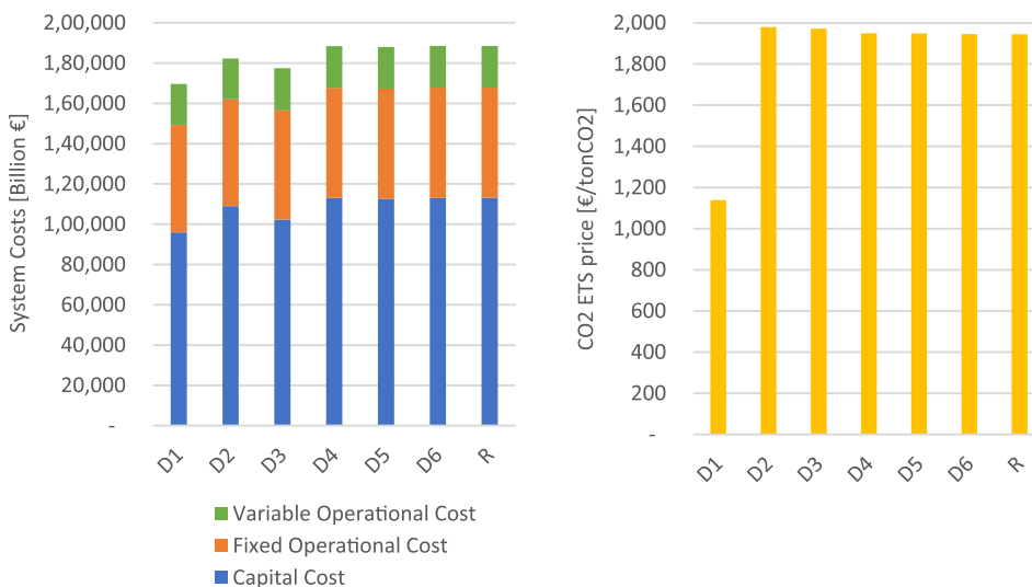
Fig. 16. Comparison of the system costs (left) and CO2 piece (right) in 2050 for the seven cases used to explore the infrastructure representation in IESA-Opt. Assuming a freely connected energy network in case D1 can drastically reduce emission prices.
